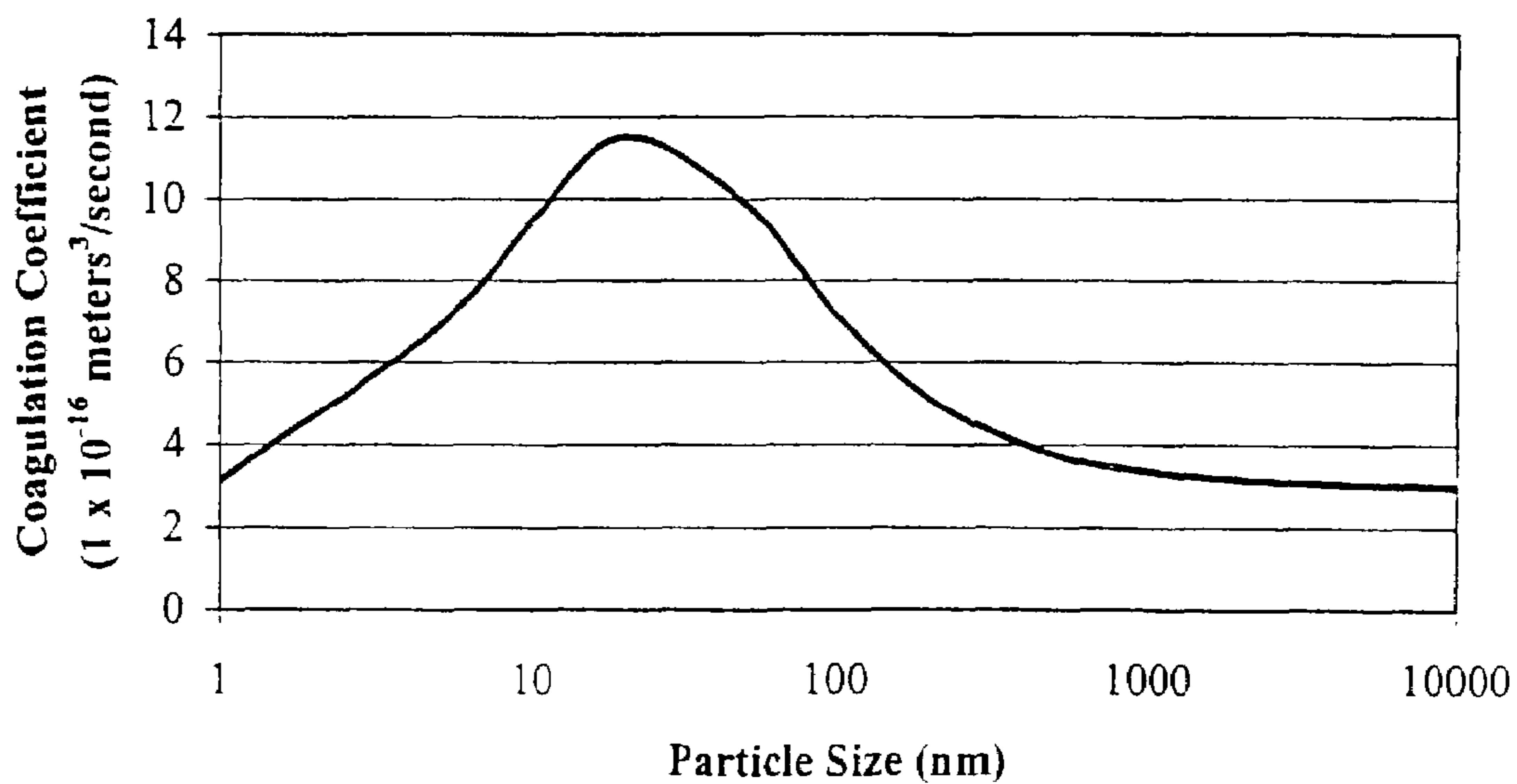
Coagulation Coefficient vs. Particle Size
