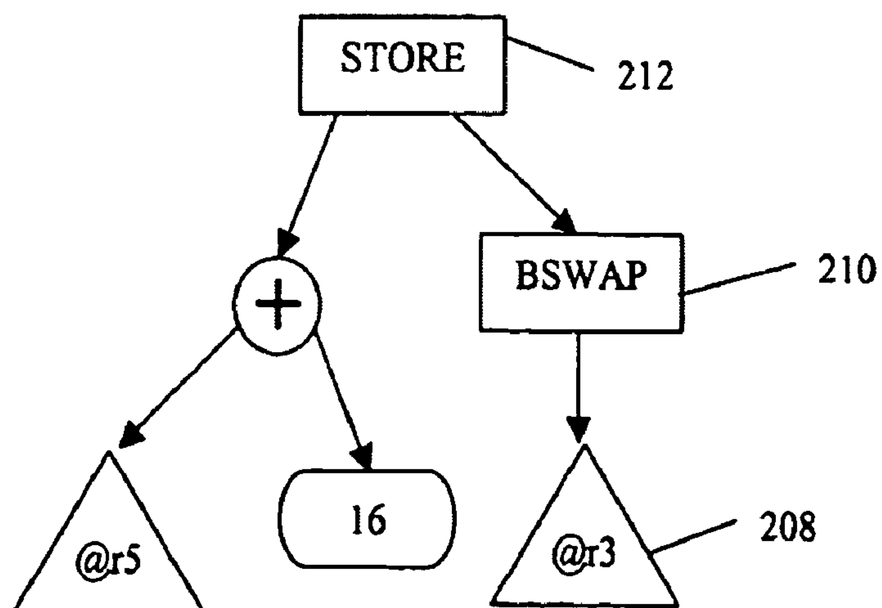
Block 2 IR Without Lazy Byteswapping
