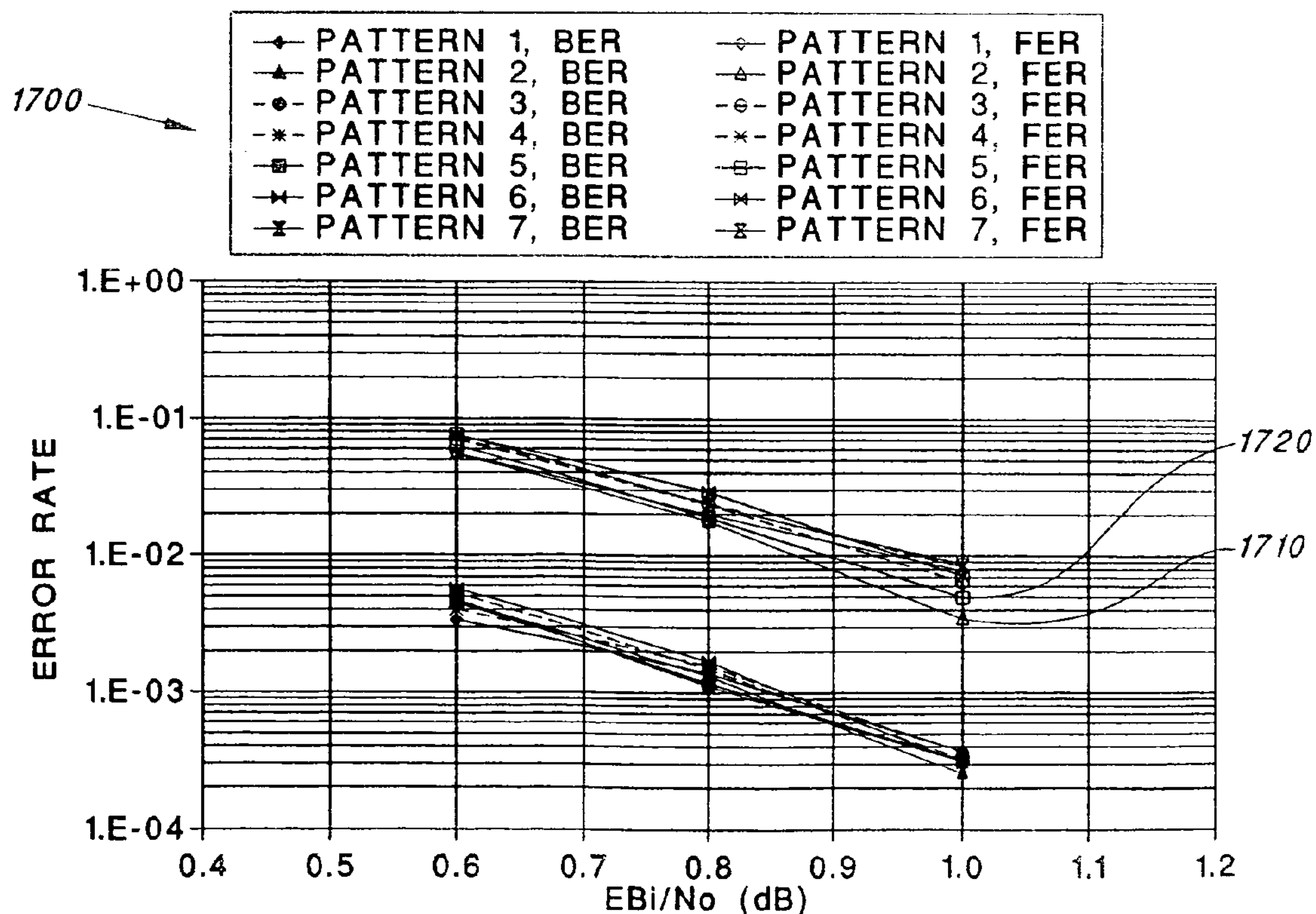
FIG. 17 COMPARISON OF RATE 1/3 PUNCTURING SCHEMES, FRAME=512
