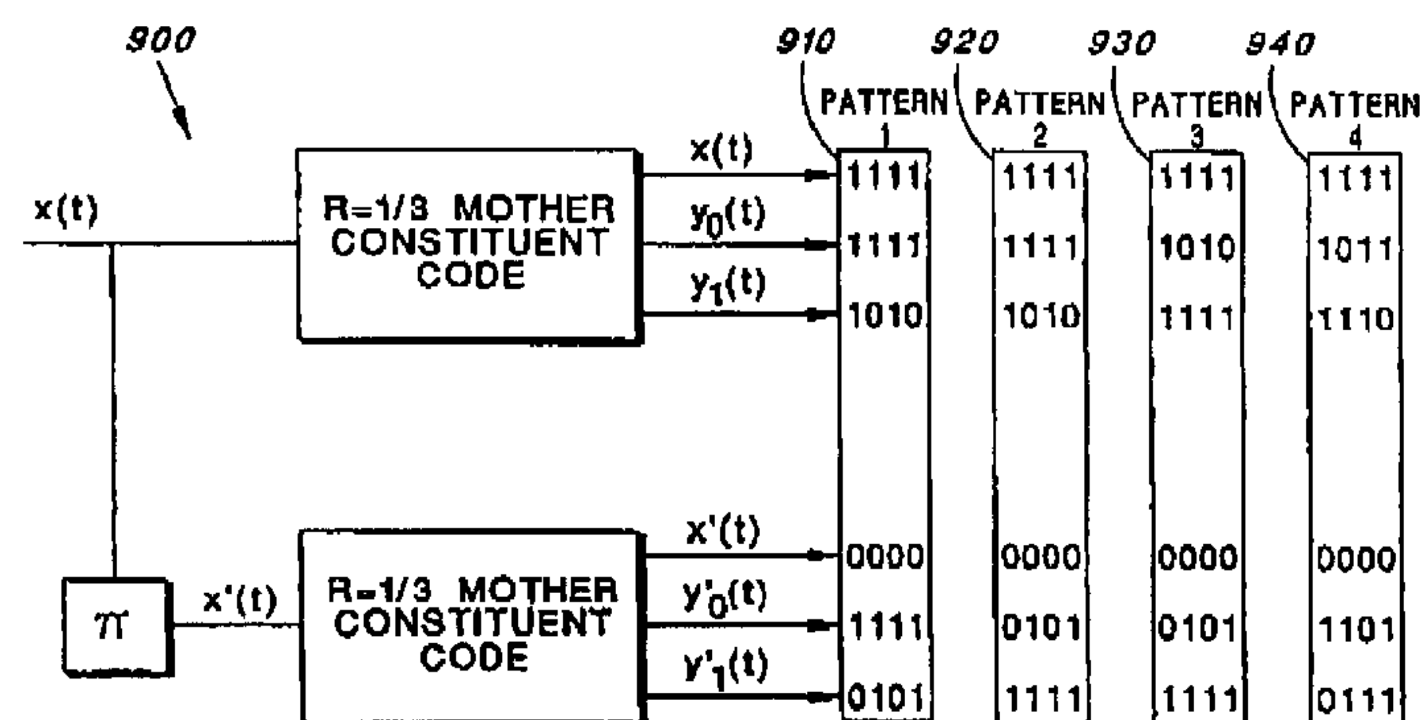
PUNCTURING SCHEMES STUDIED FOR OPTIMIZING THE RATE 1/4 TURBO CODE
