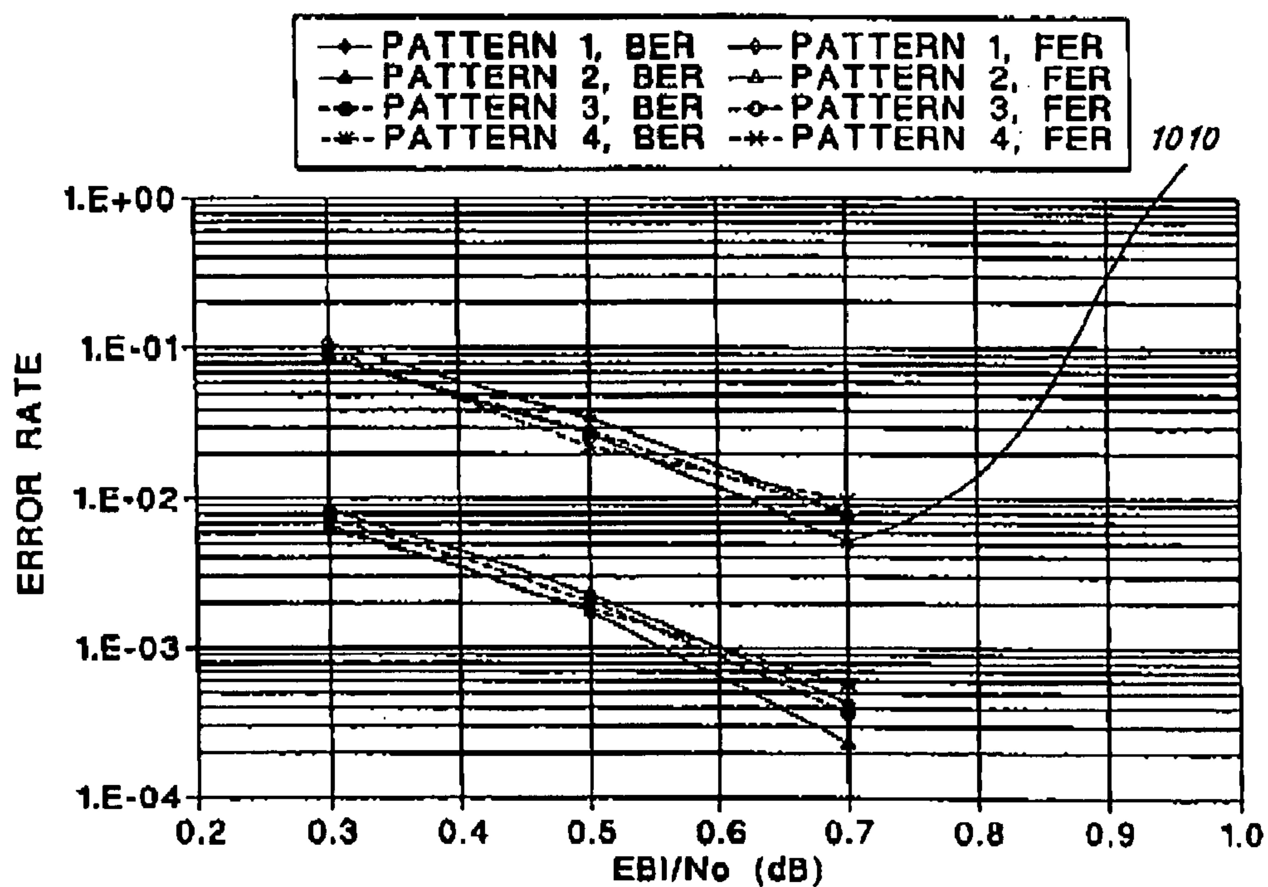
FIG. 10 PERFORMANCE OF CODE #1, FRAME SIZE=512
