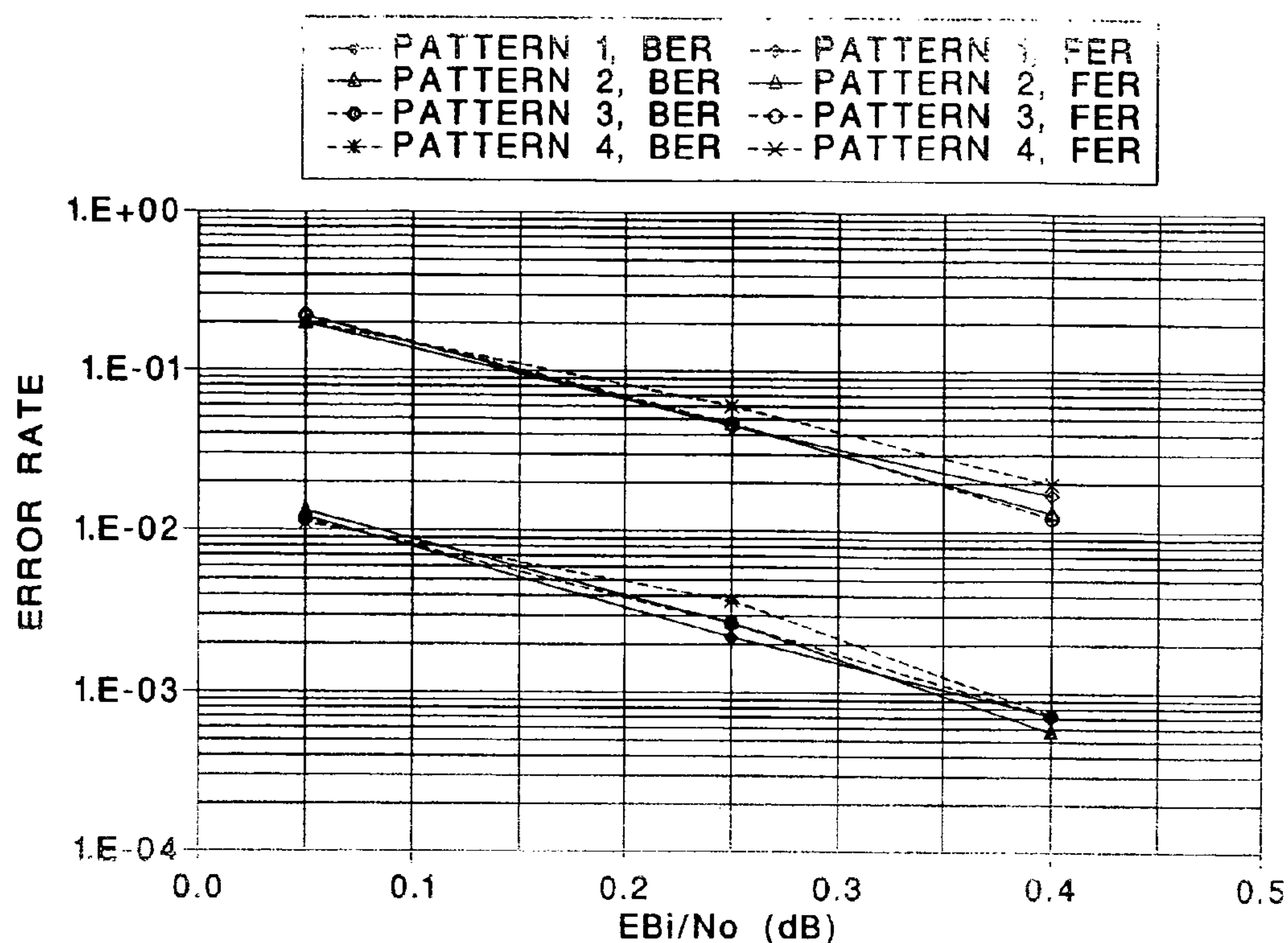
FIG. 13 BER/FER PERFORMANCE OF CODE #1, FRAME SIZE=1024
