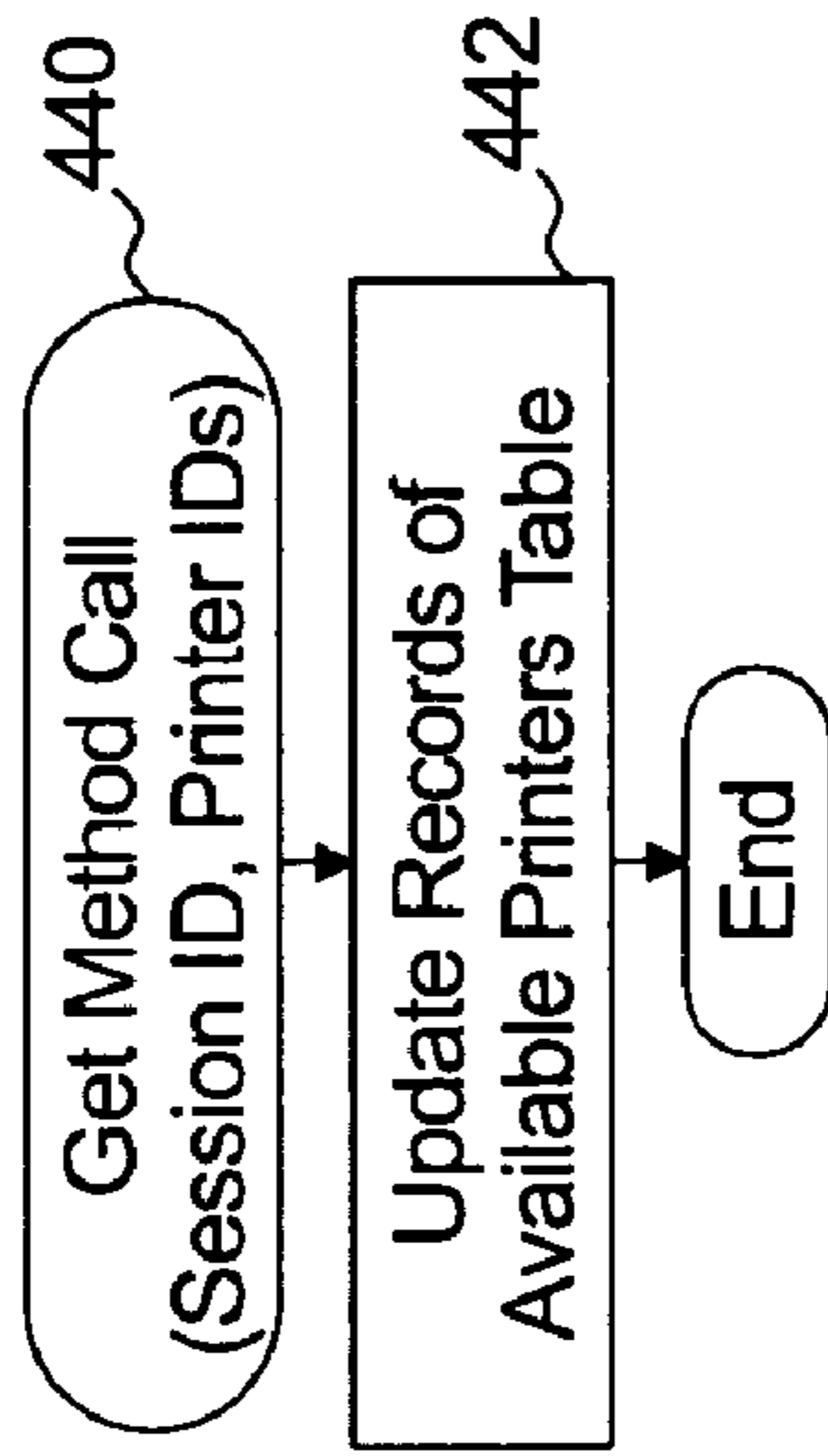
Figure 12 (Send Printers)
