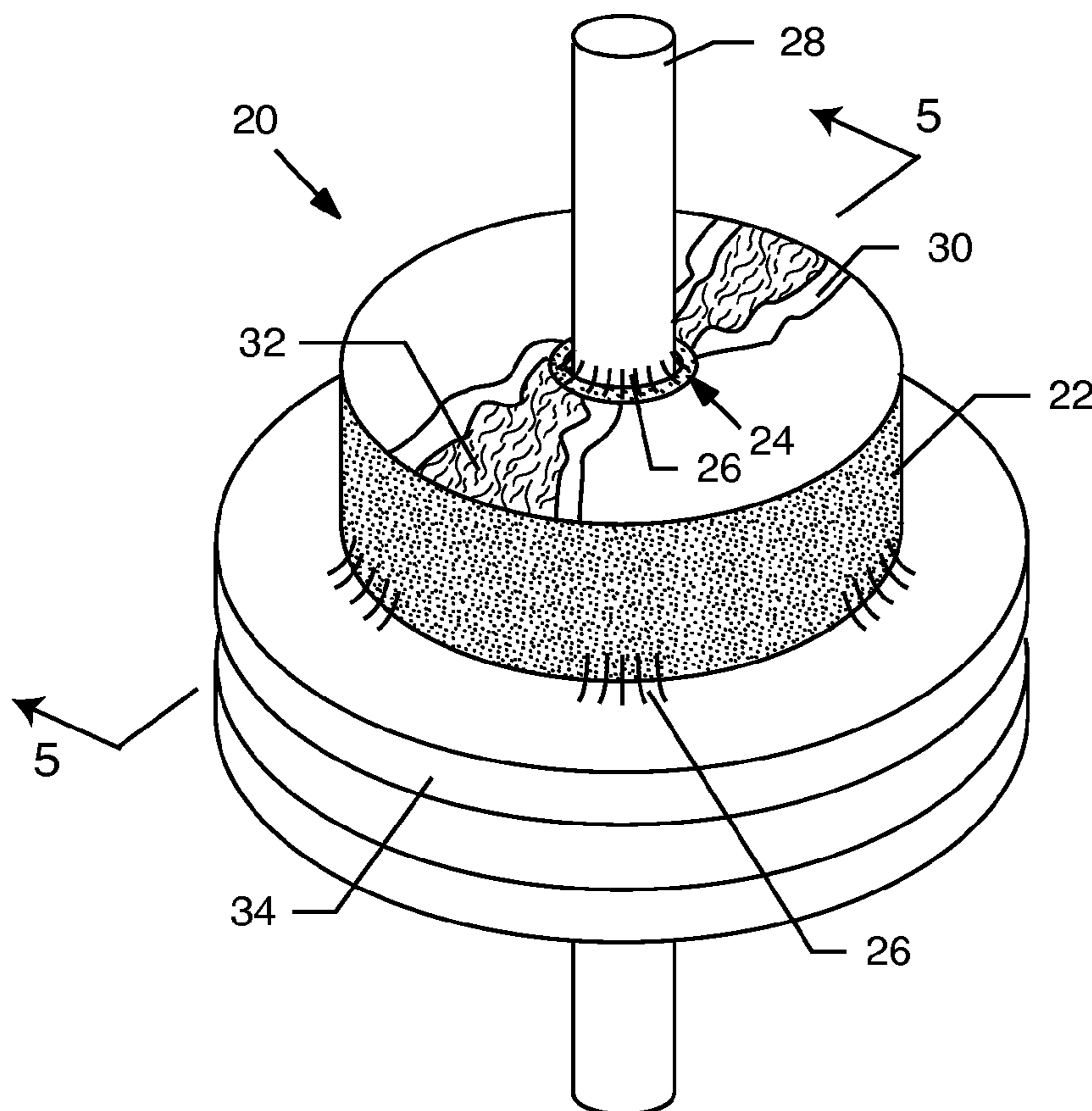
FIG. 1 PRIOR ART
