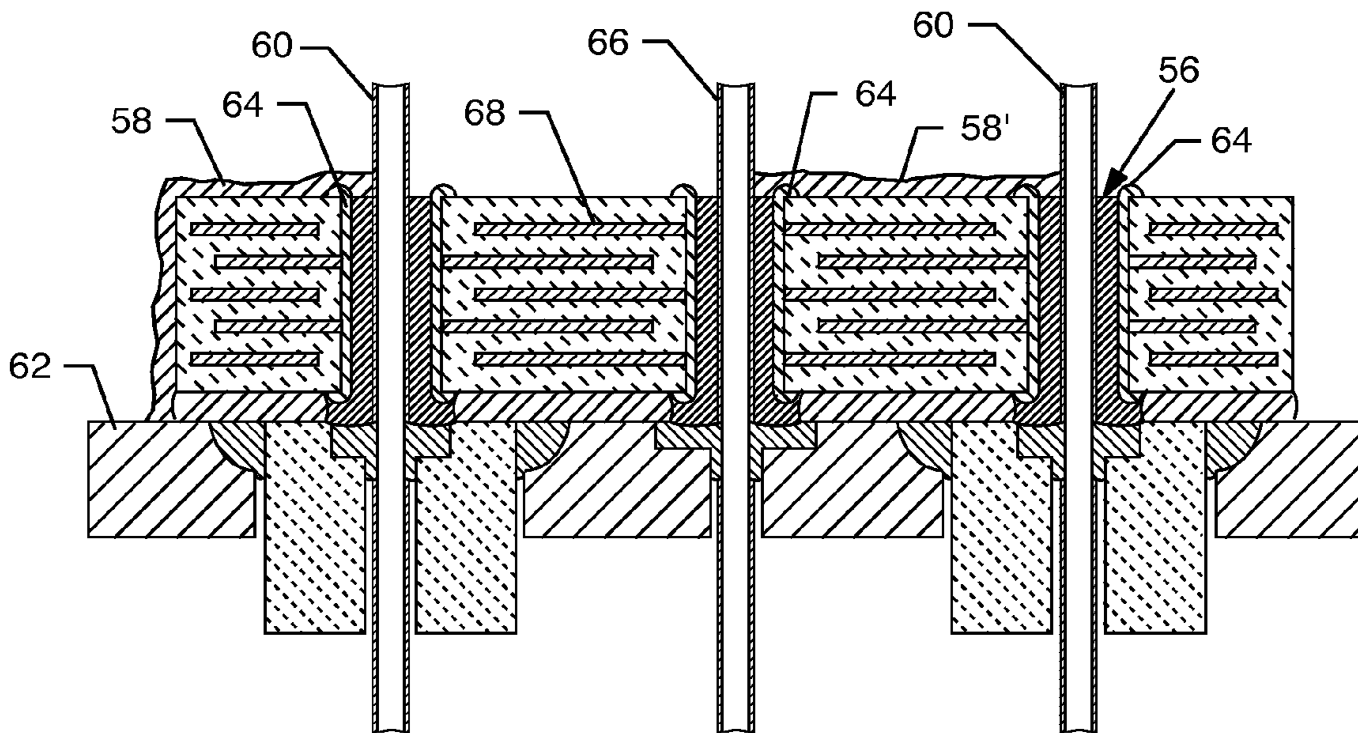
FIG. 12 PRIOR ART
