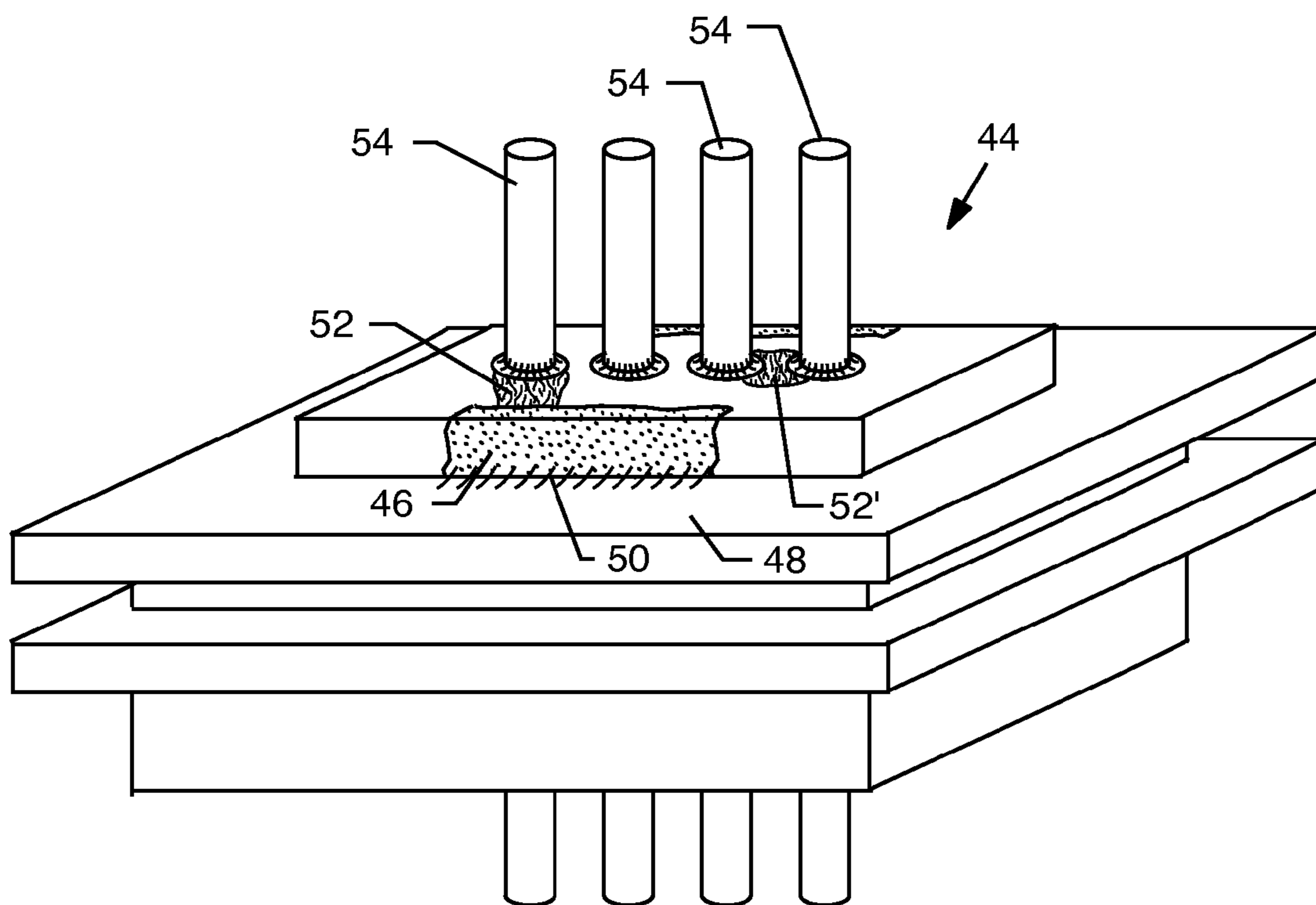
FIG. 8 PRIOR ART
