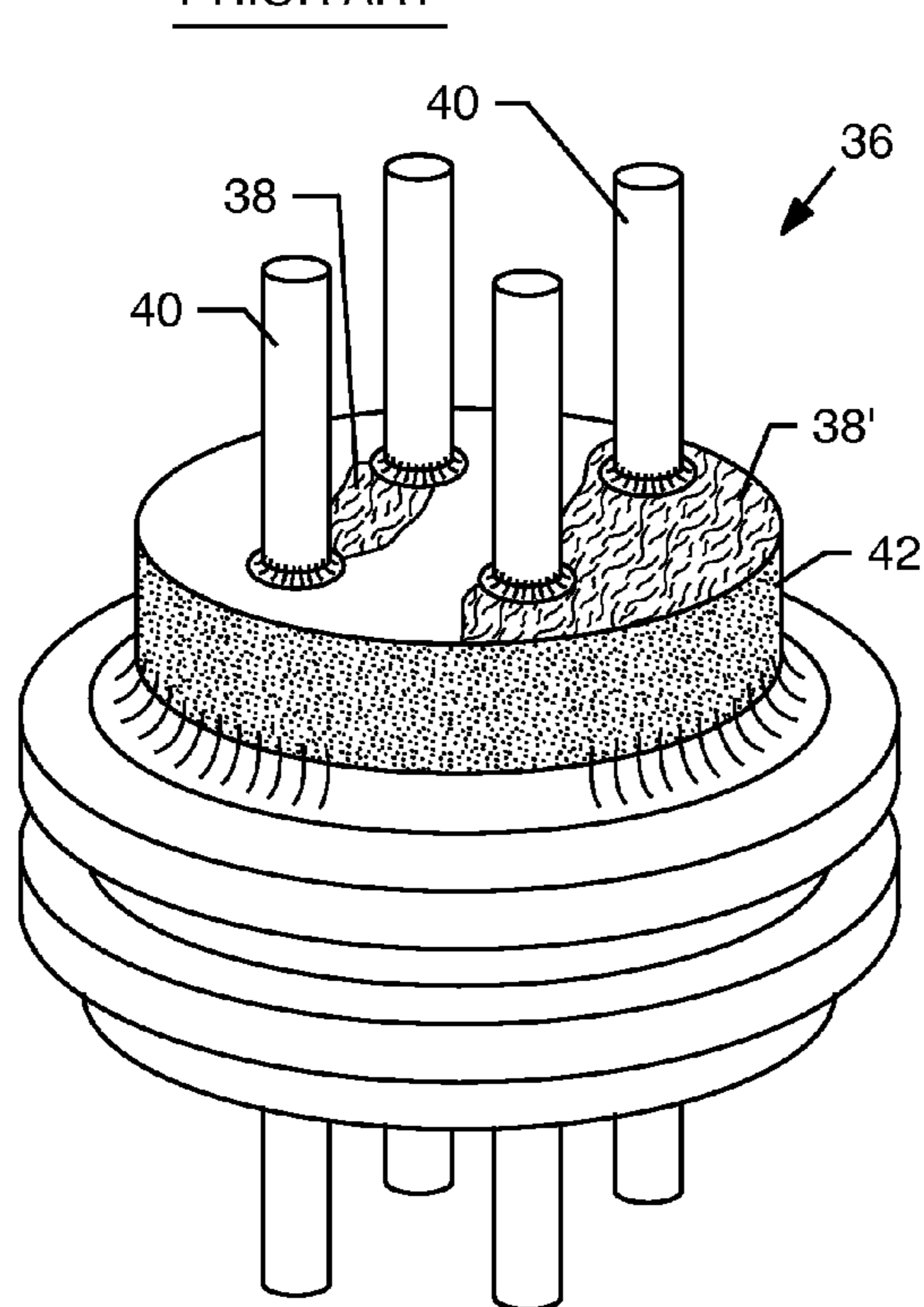
FIG. 6 PRIOR ART
