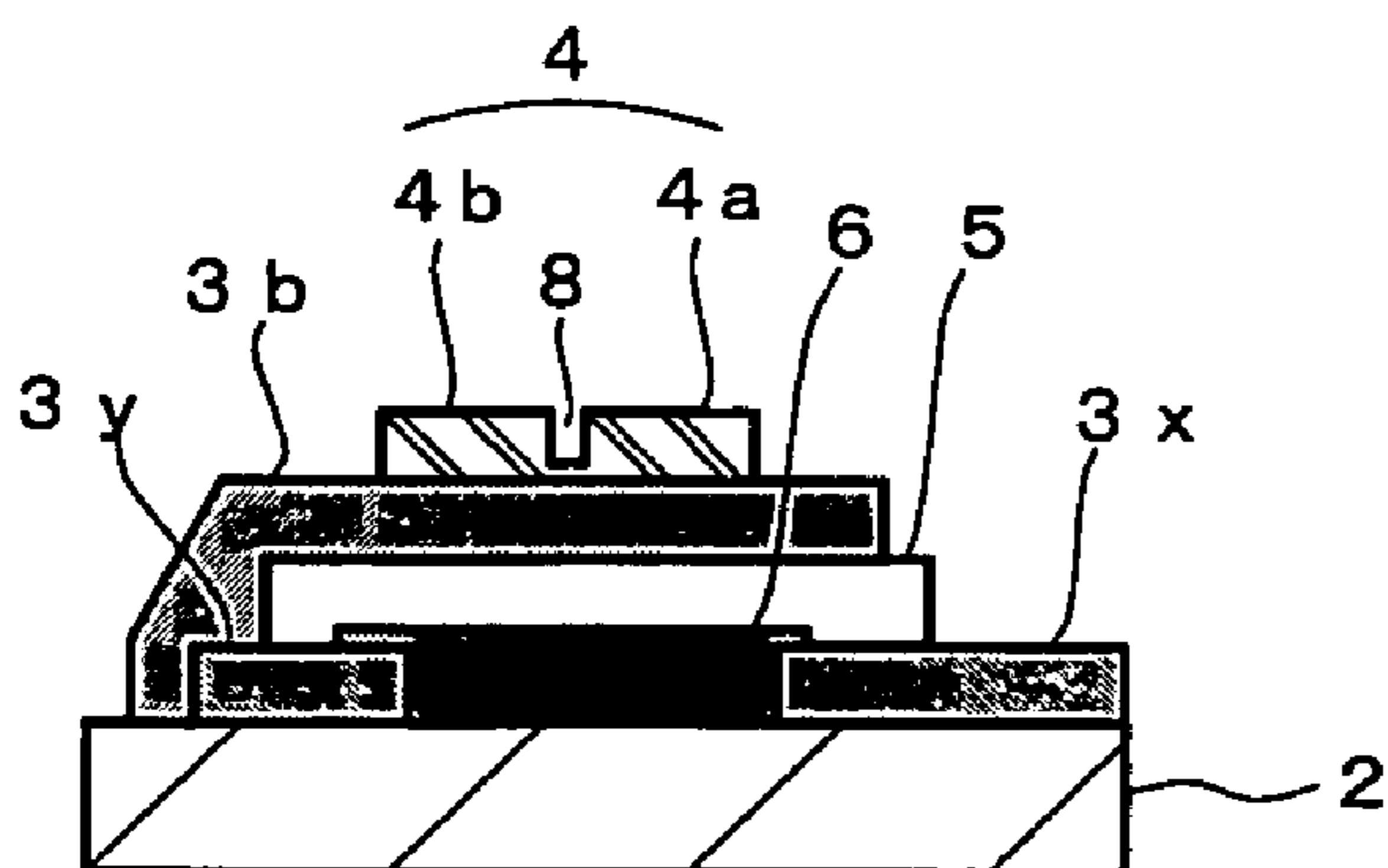
(y-y cross section)
