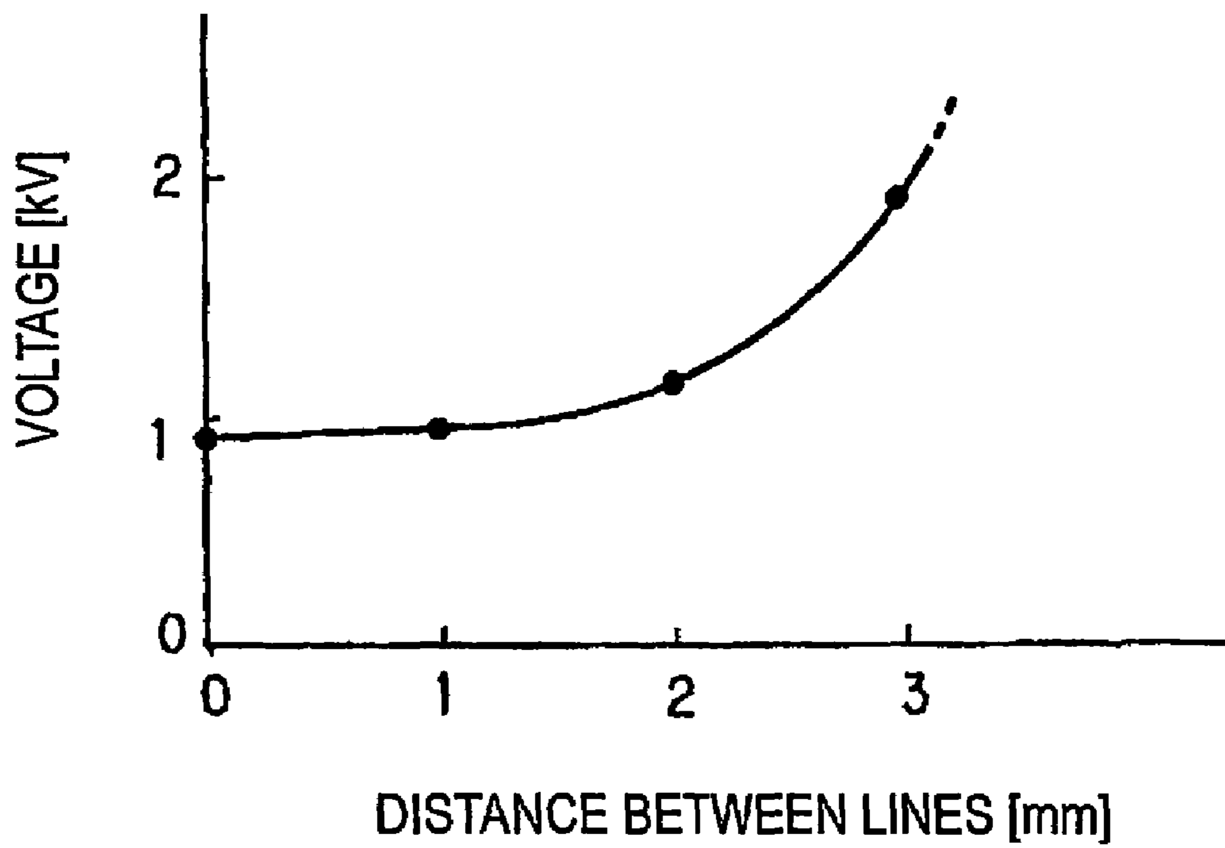
CORONA DISCHARGE OCCURRENCE VOLTAGE (AT. 180°C)
