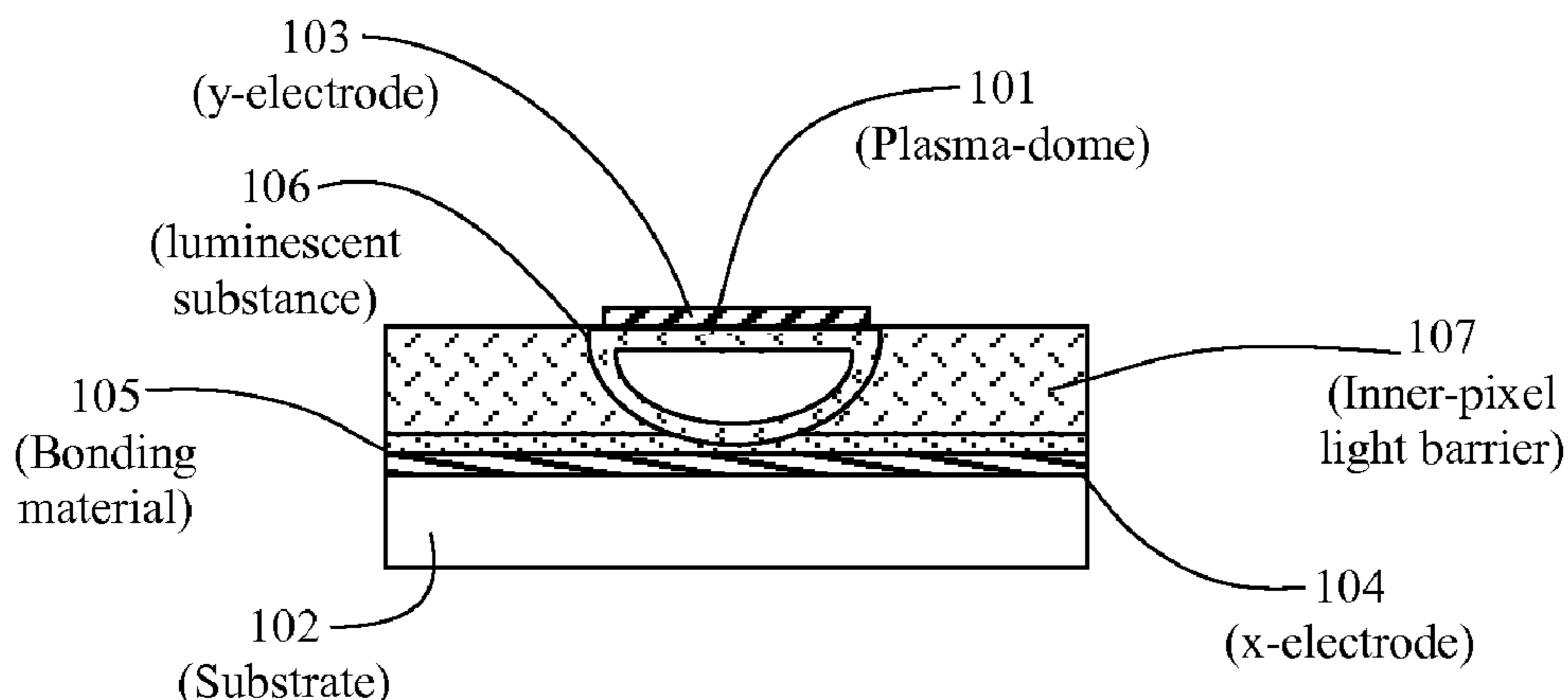
Section A-A View
