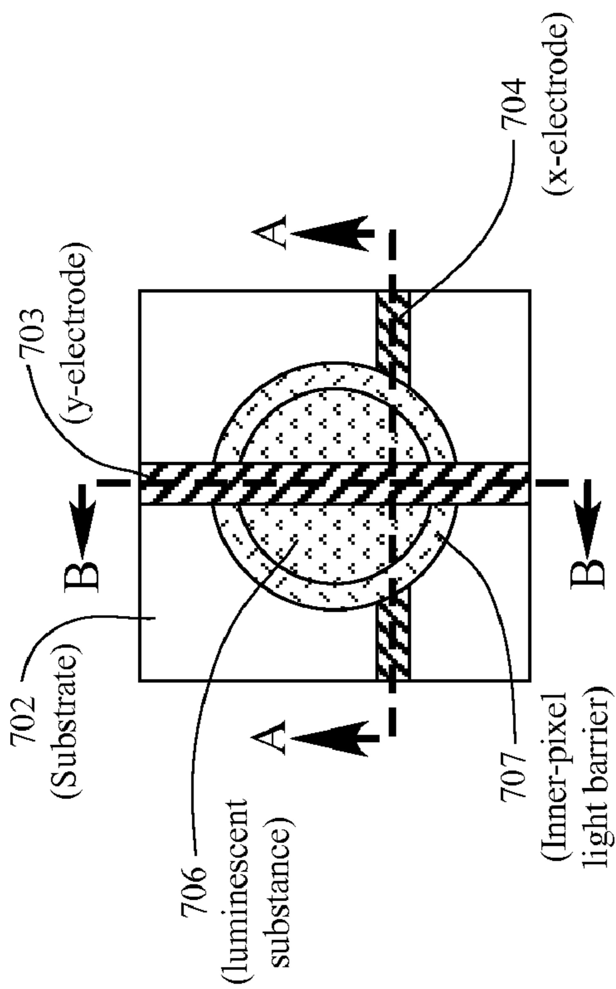
Figure 7 Two Electrodes Top View
