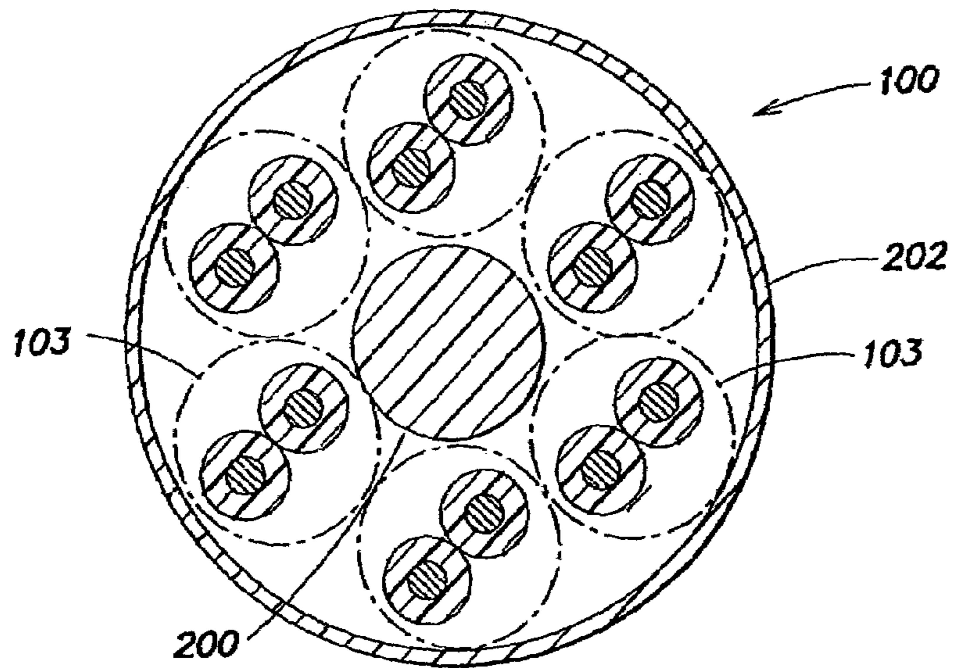
FIG. 1 PRIOR ART
