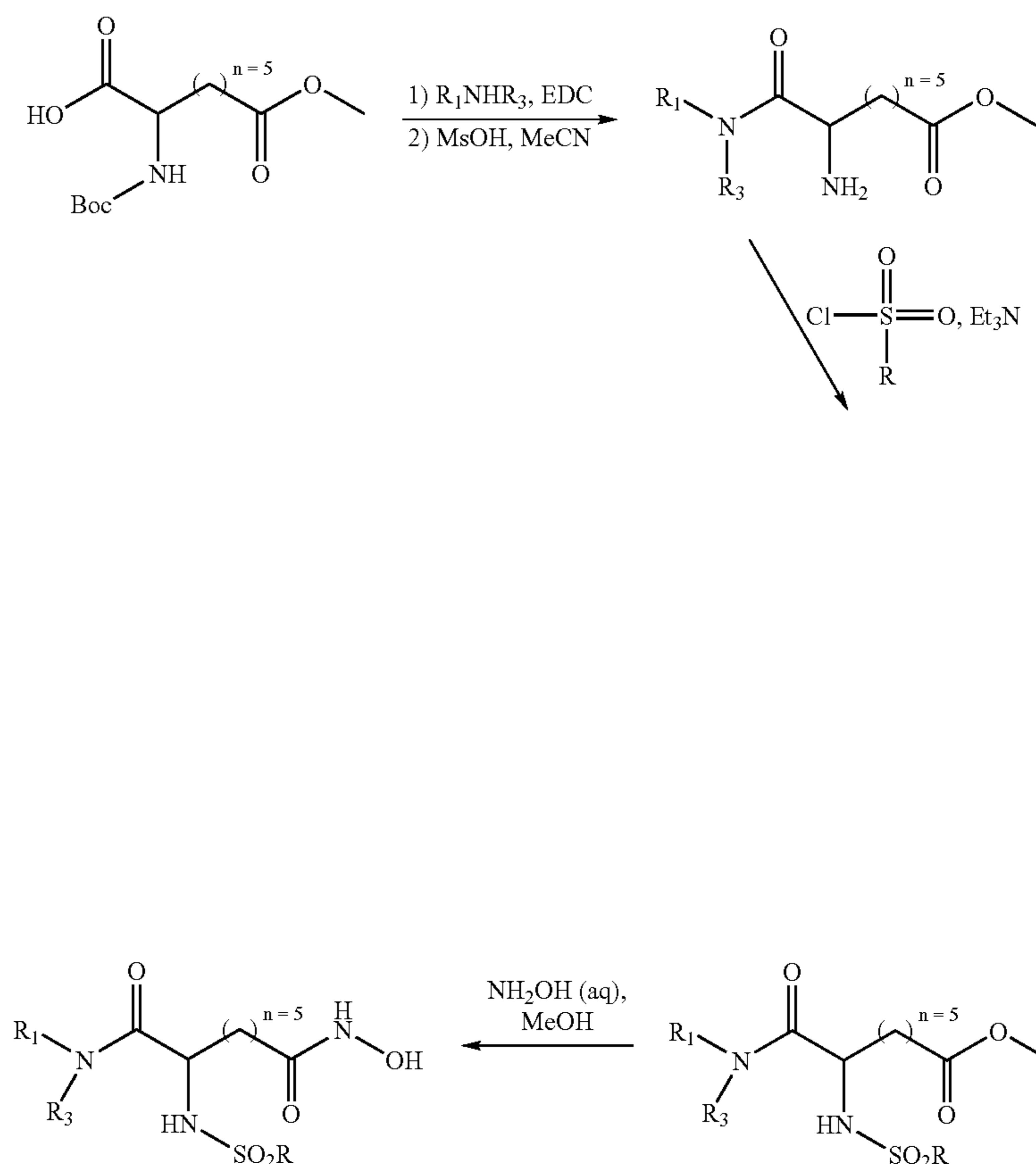
SCHEME 1
