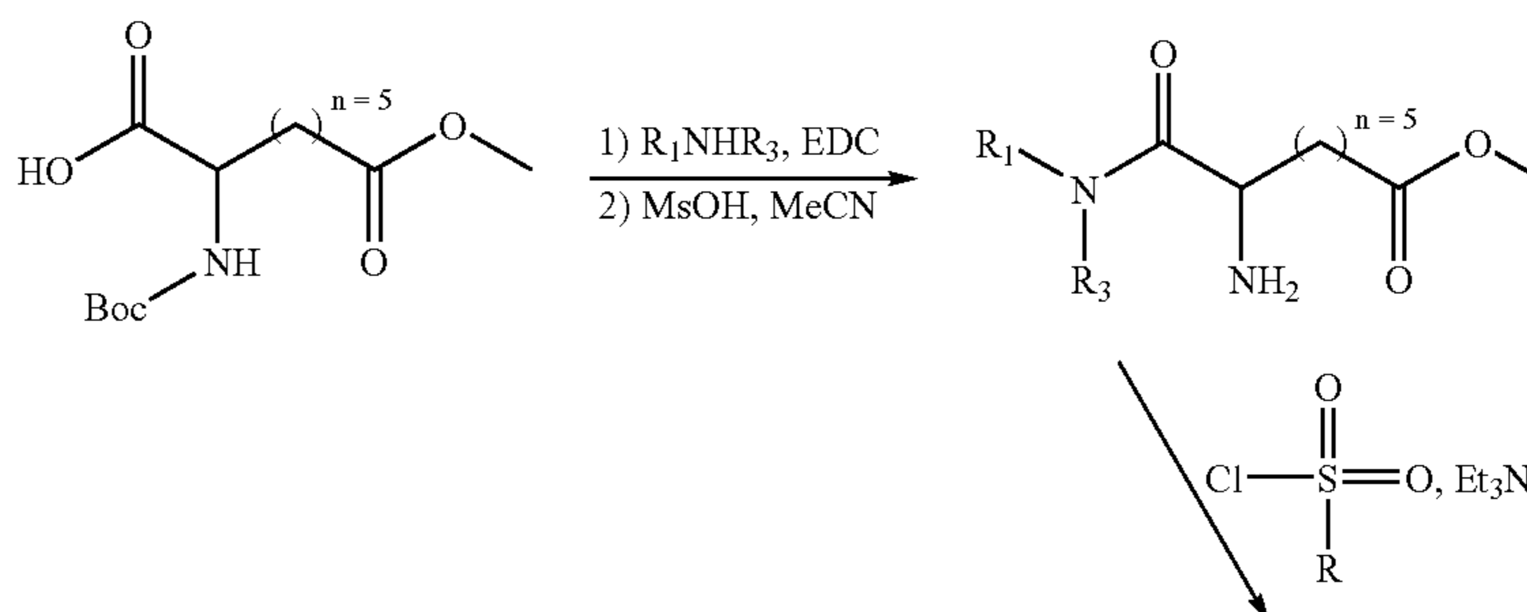
SCHEME 1
