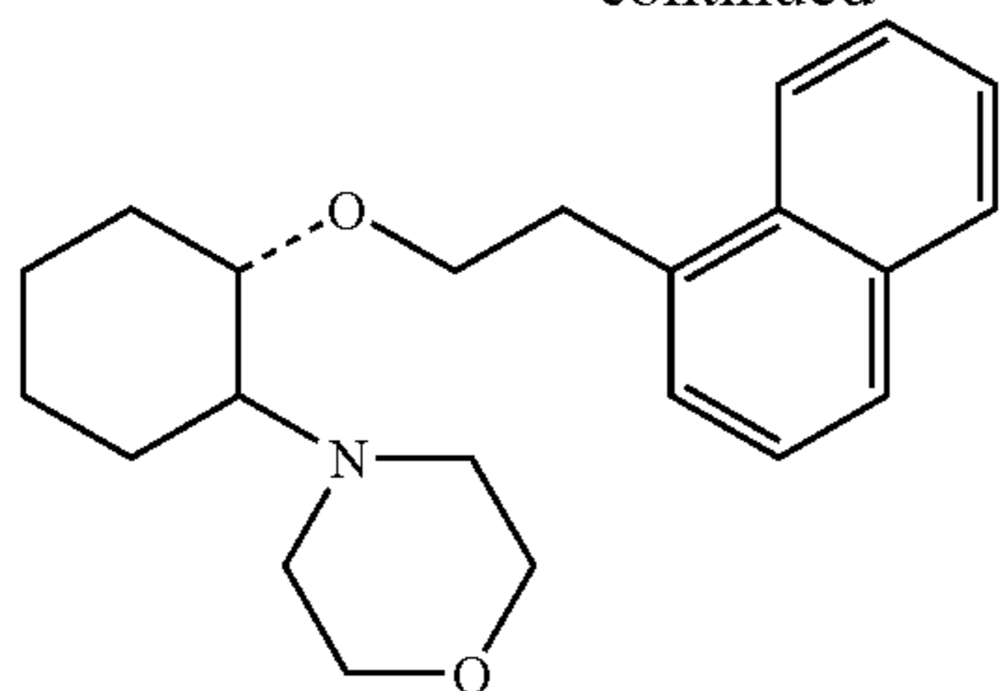
(1R,2R)/(1S,2S)-[2-(4-morpholinyl)-1-(1-naphthenethoxy)]cyclohexane
