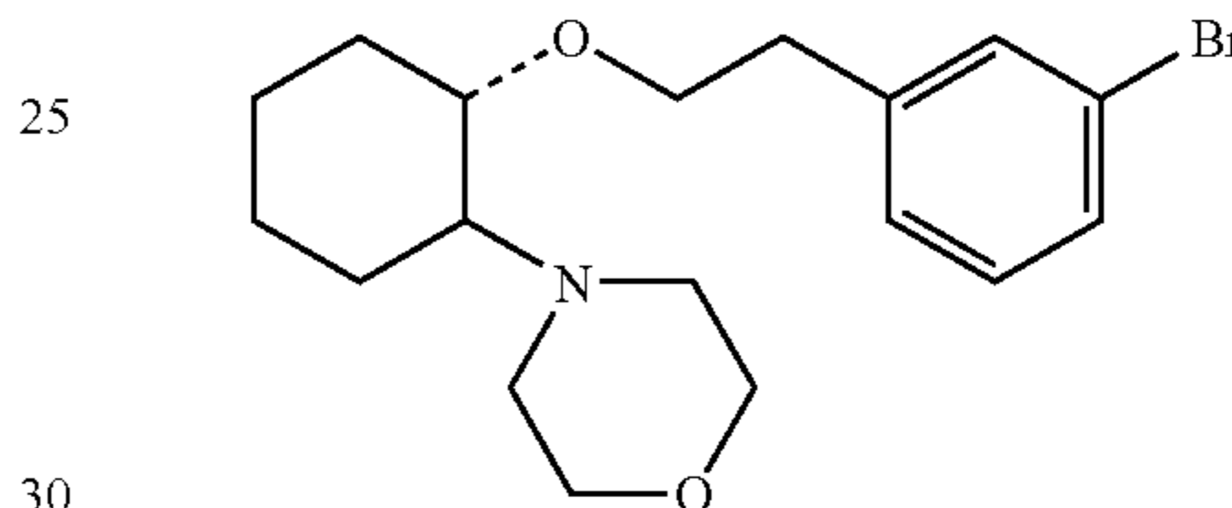
(1R,2R)/(1S,2S)-[2-(4-morpholinyl)-1-(3-bromophenethoxy)]cyclohexane
