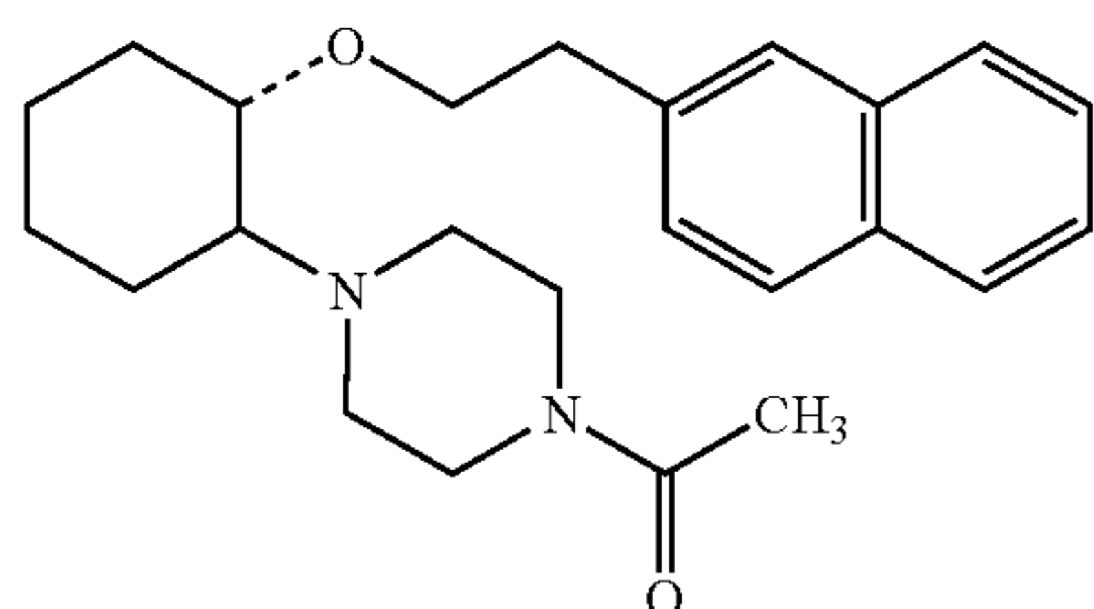
(1R,2R)/(1S,2S)-2-(1-acetylpiperazinyl)-1-(2-naphthenoxy)cyclohexane
