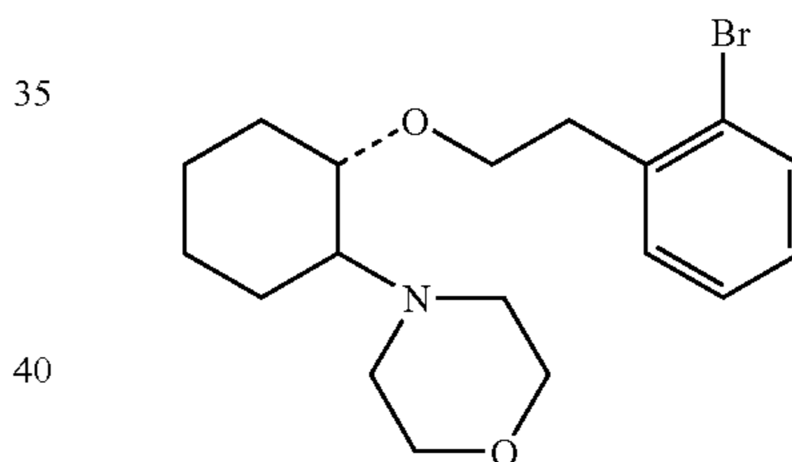
(1R,2R)/(1S,2S)-[2-(4-morpholinyl)-1-(2-bromophenethoxy)]cyclohexane
