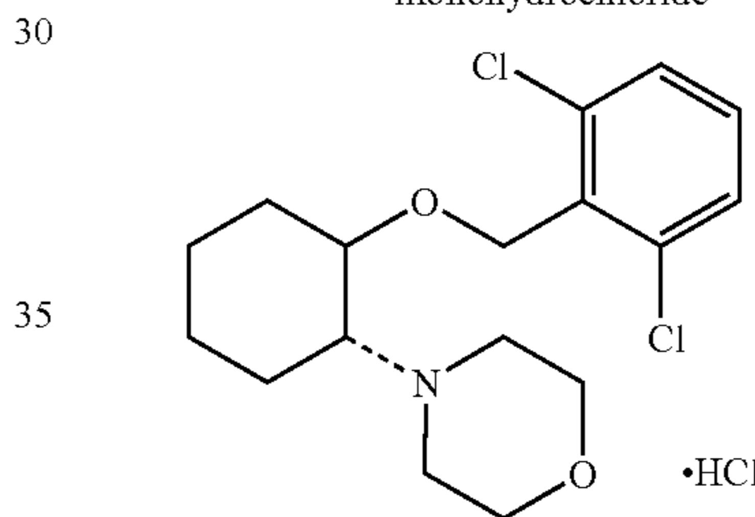
(1R,2R)/(1S,2S)-2-(4-morpholinyl)-1-[(2,6-dichlorophenyl)methoxy]cyclohexane monohydrochloride
