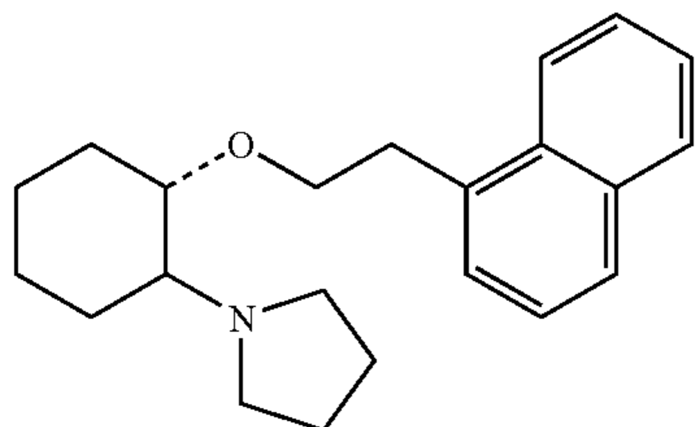
(1R,2R)/(1S,2S)-[2-(1-pyrrolidinyl)-1-(1-naphthenethoxy)]cyclohexane
