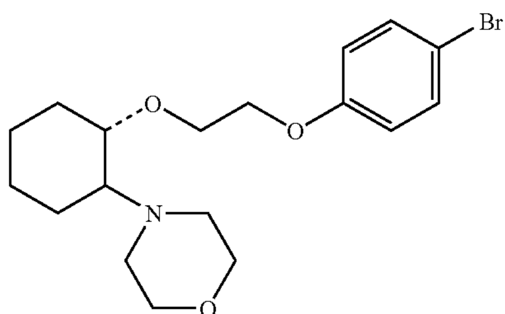
(1R,2R)/(1S,2S)-[2-(4-morpholinyl)-1-[2-(4-bromophenoxy)ethoxy]]cyclohexane
