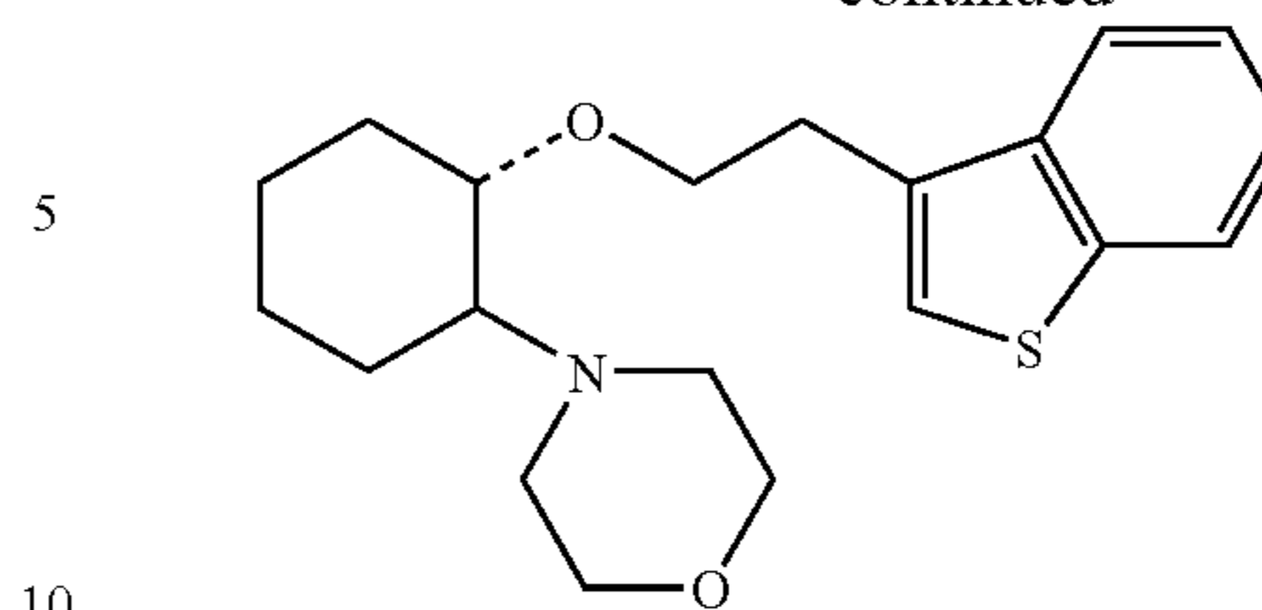
(1R,2R)/(1S,2S)-[2-(4-morpholinyl)-1-(2-(benzo[b]thiophen-3-yl))]cyclohexane
