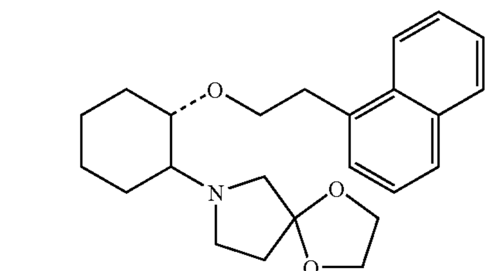
(1R,2R)/(1S,2S)-2-[1,4-dioxo-7-azaspiro[4.4]non-7-yl]-1-(1-naphthenoxy)cyclohexane
