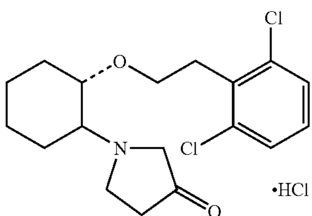
(1R,2R)/(1S,2S)-2-(3-ketopyrrolidinyl)-1-(2,6-dichlorophenoxy)cyclohexane
