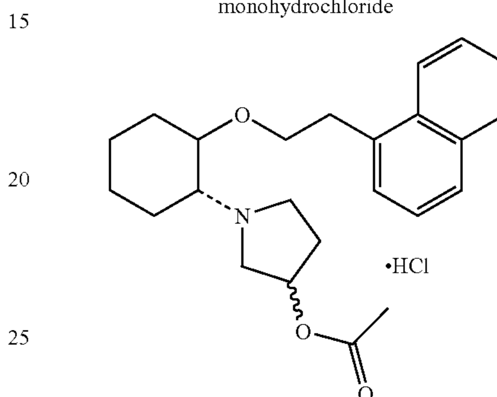
(1R,2R)/(1S,2S)-2-(3-acetoxypyrrrolidinyl)-1-(1-naphthenoxy)cyclohexane monohydrochloride
