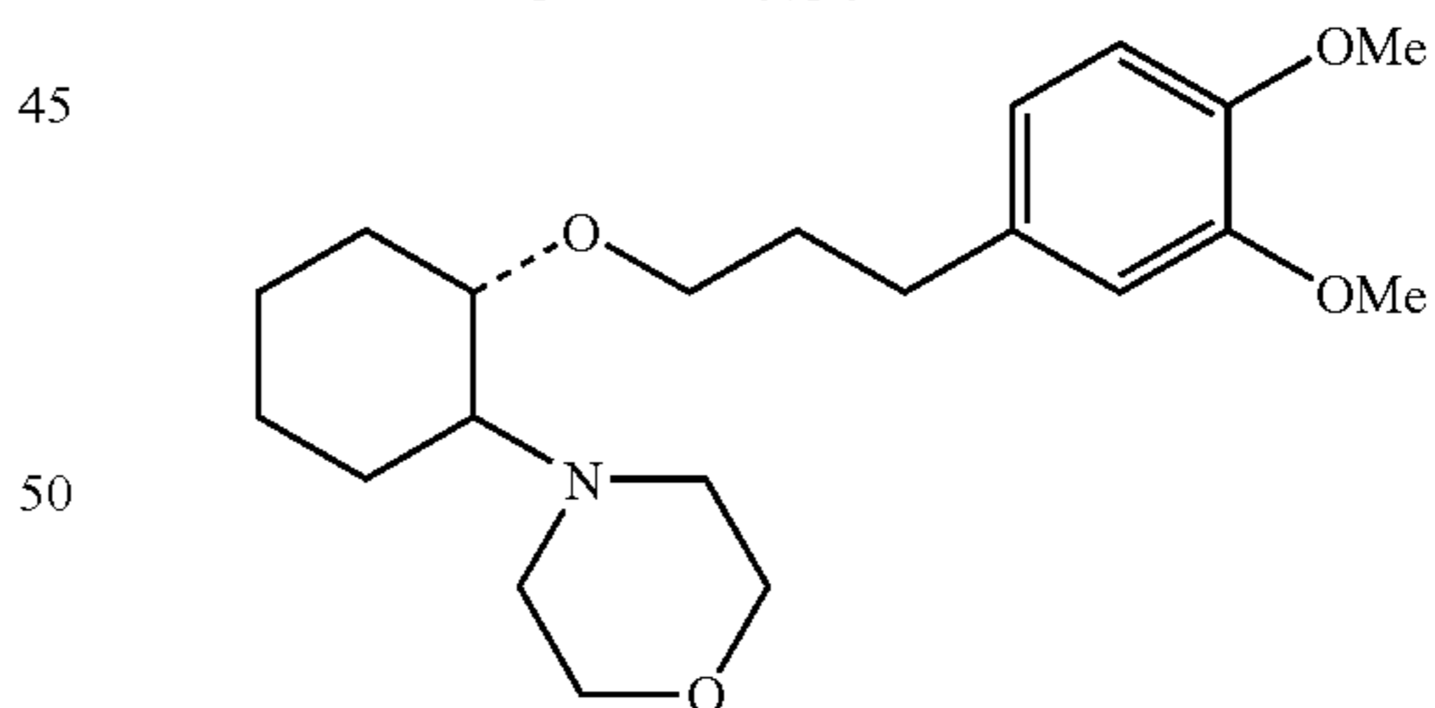
(1R,2R)/(1S,2S)-[2-(4-morpholinyl)-1-(3-(3,4-dimethoxyphenyl)propoxy)]cyclohexane
