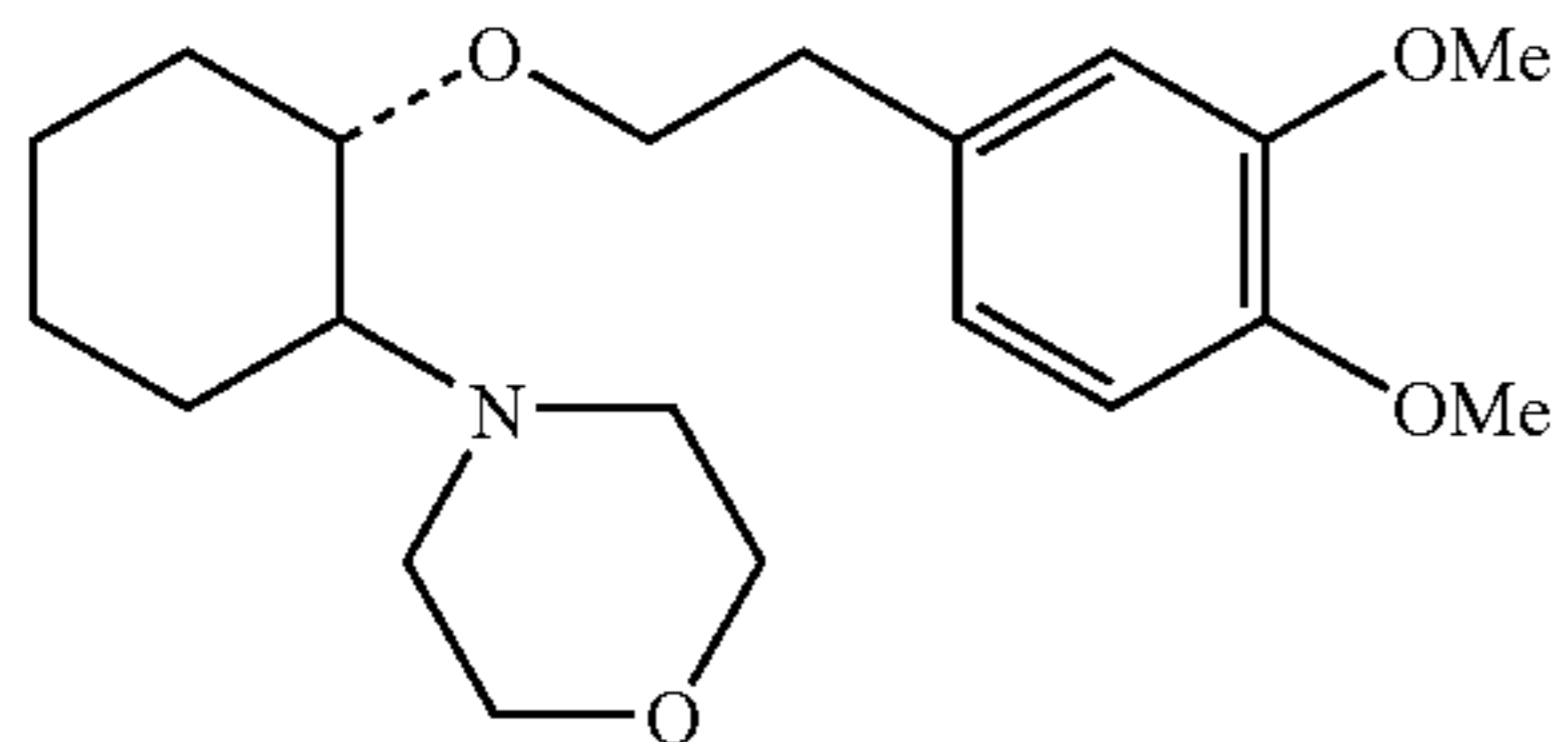
(1R,2R)/(1S,2S)-[2-(4-morpholinyl)-1-(3,4-dimethoxyphenethoxy)]cyclohexane
