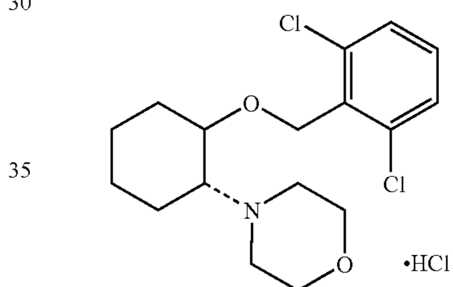
(1R,2R)/(1S,2S)-2-(4-morpholinyl)-1-[(2,6-dichlorophenyl)methoxy]cyclohexane monohydrochloride
