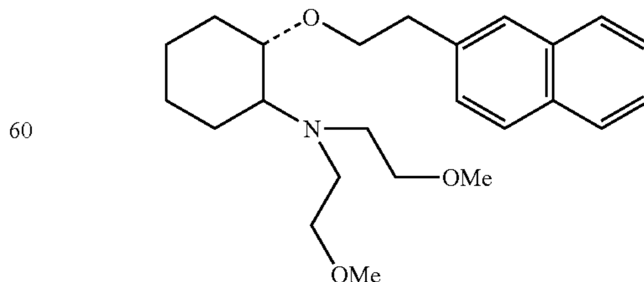
(1R,2R)/(1S,2S)-[2-[bis(2-methoxyethyl)aminy]-1-(2-naphthenethoxy)]cyclohexane
