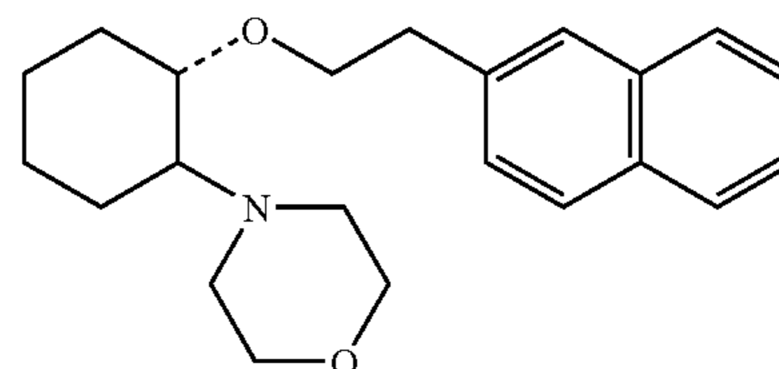
(1R,2R)/(1S,2S)-[2-(4-morpholinyl)-1-(2-naphthenethoxy)]cyclohexane
