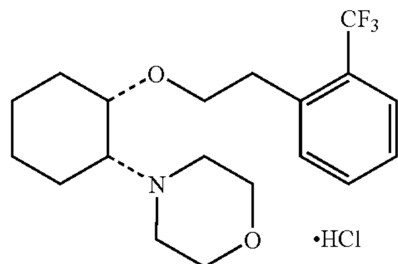
(1R,2S)/(1S,2R)-2-(4-morpholinyl)-1-[(2-trifluoromethyl)phenoxy]cyclohexane monohydrochloride
