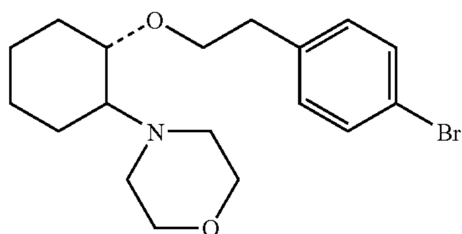
(1R,2R)/(1S,2S)-[2-(4-morpholinyl)-1-(4-bromophenethoxy)]cyclohexane
