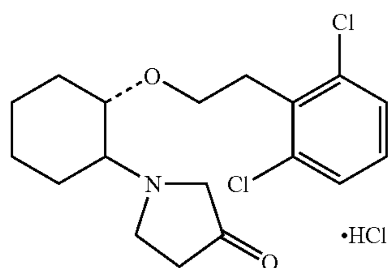
(1R,2R)/(1S,2S)-2-(3-ketopyrrolidinyl)-1-(2,6-dichlorophenoxy)cyclohexane
