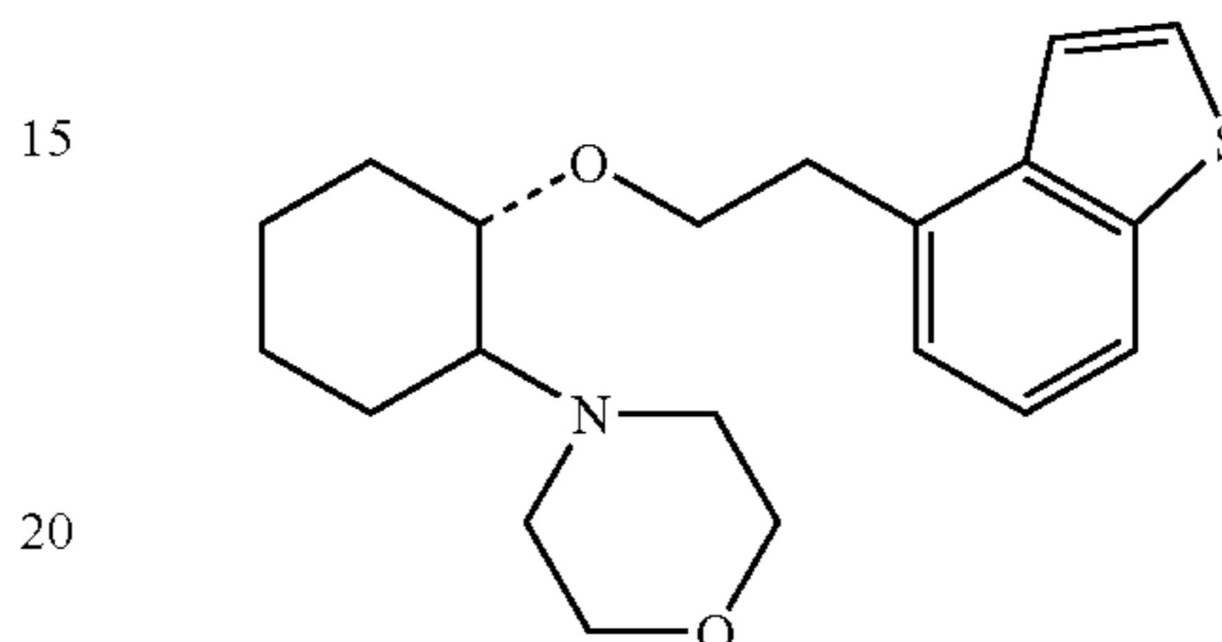
(1R,2R)/(1S,2S)-[2-(4-morpholinyl)-1-(2-(benzo[b]thiophen-4-yl))]cyclohexane
