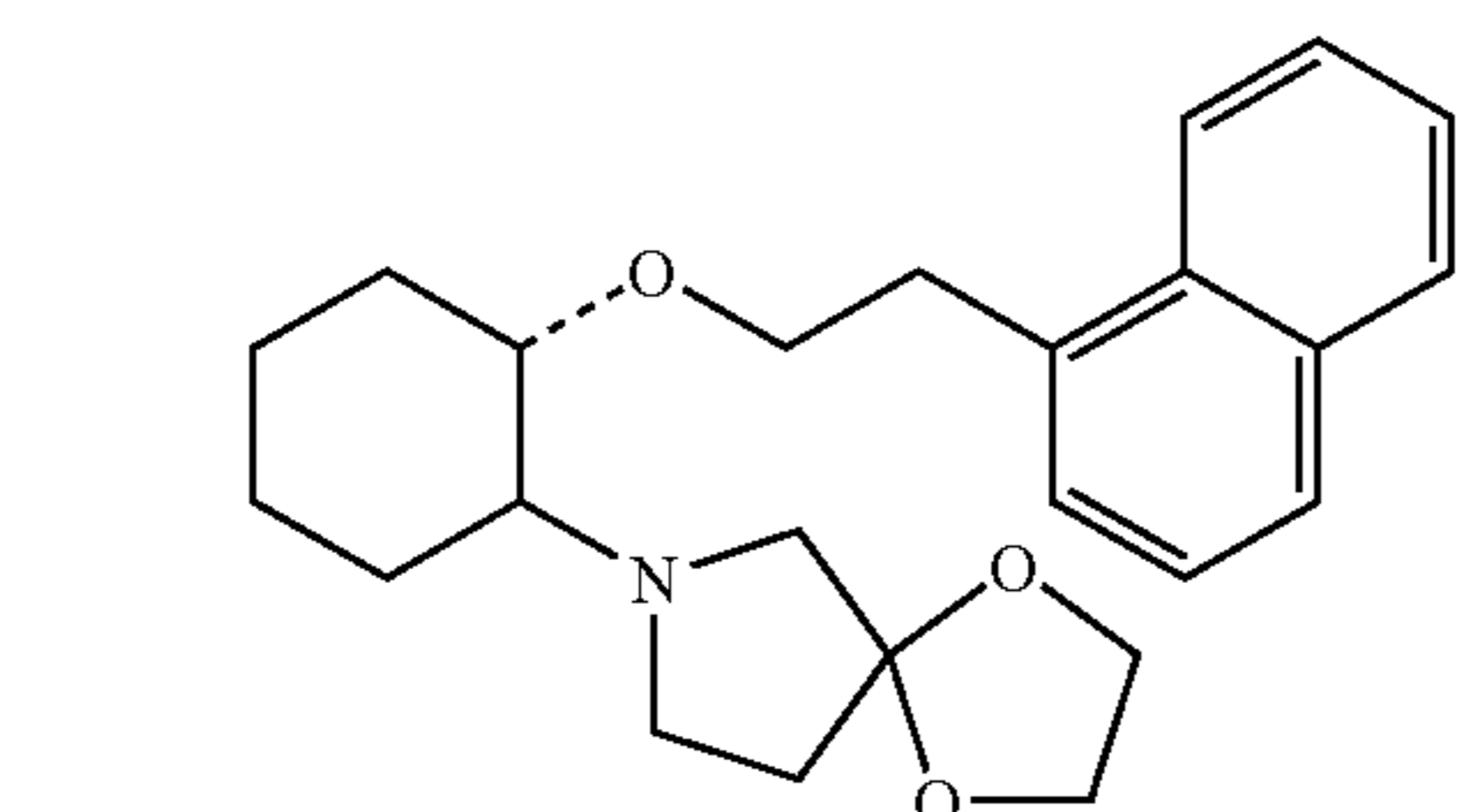
(1R,2R)/(1S,2S)-2-[1,4-dioxo-7-azaspiro[4.4]non-7-yl]-1-(1-naphthenoxy)cyclohexane
