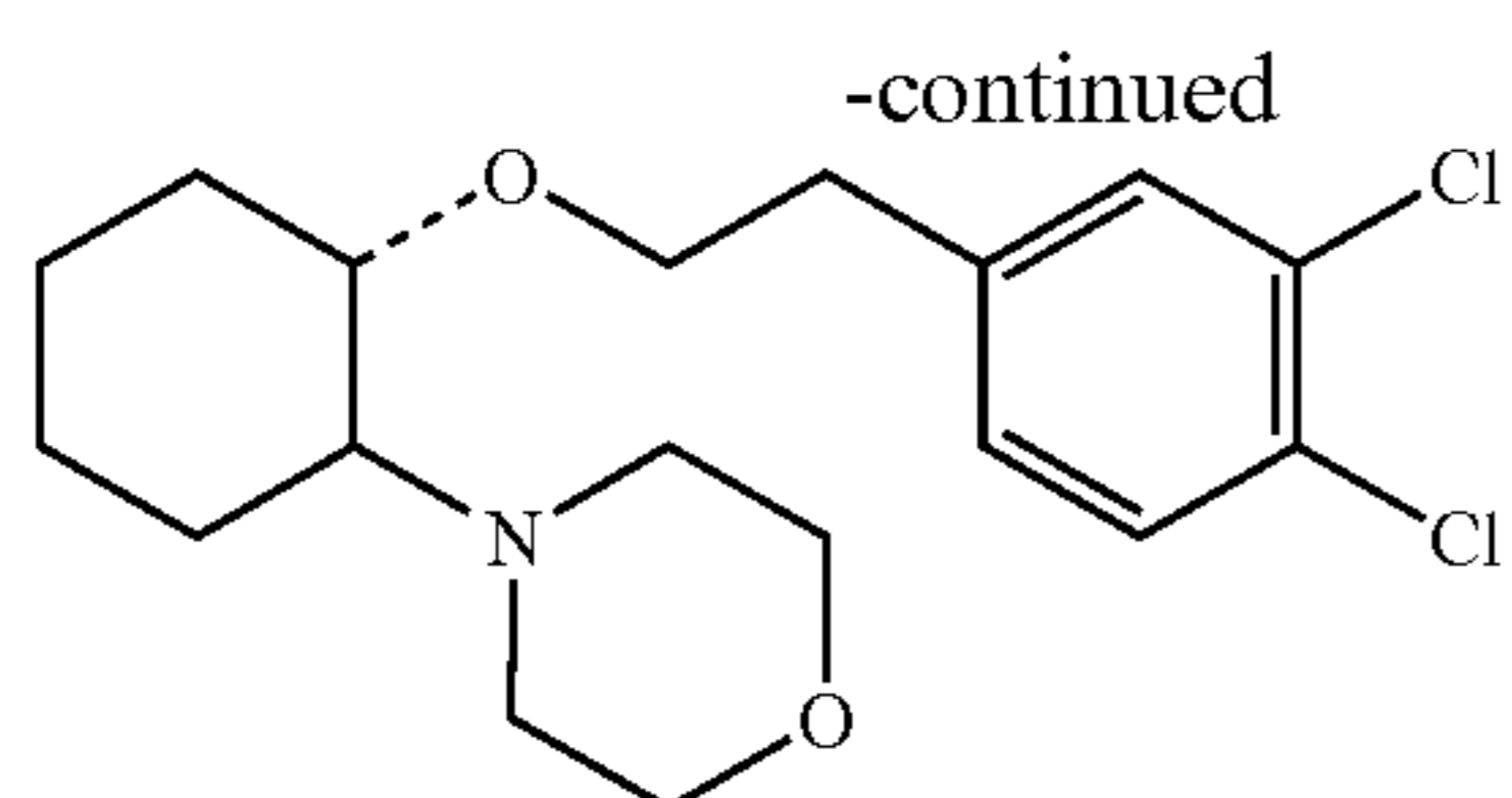
(1R,2R)/(1S,2S)-[2-(4-morpholinyl)-1-(3,4-dichlorophenoxy)cyclohexane
