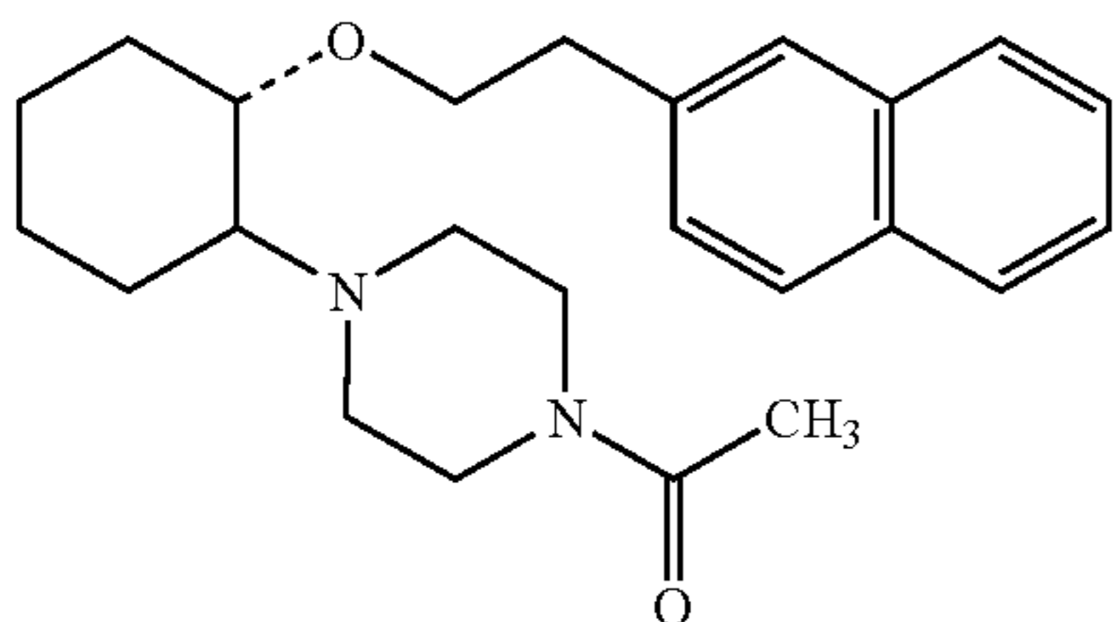
(1R,2R)/(1S,2S)-2-(1-acetylpiperazinyl)-1-(2-naphthenoxy)cyclohexane
