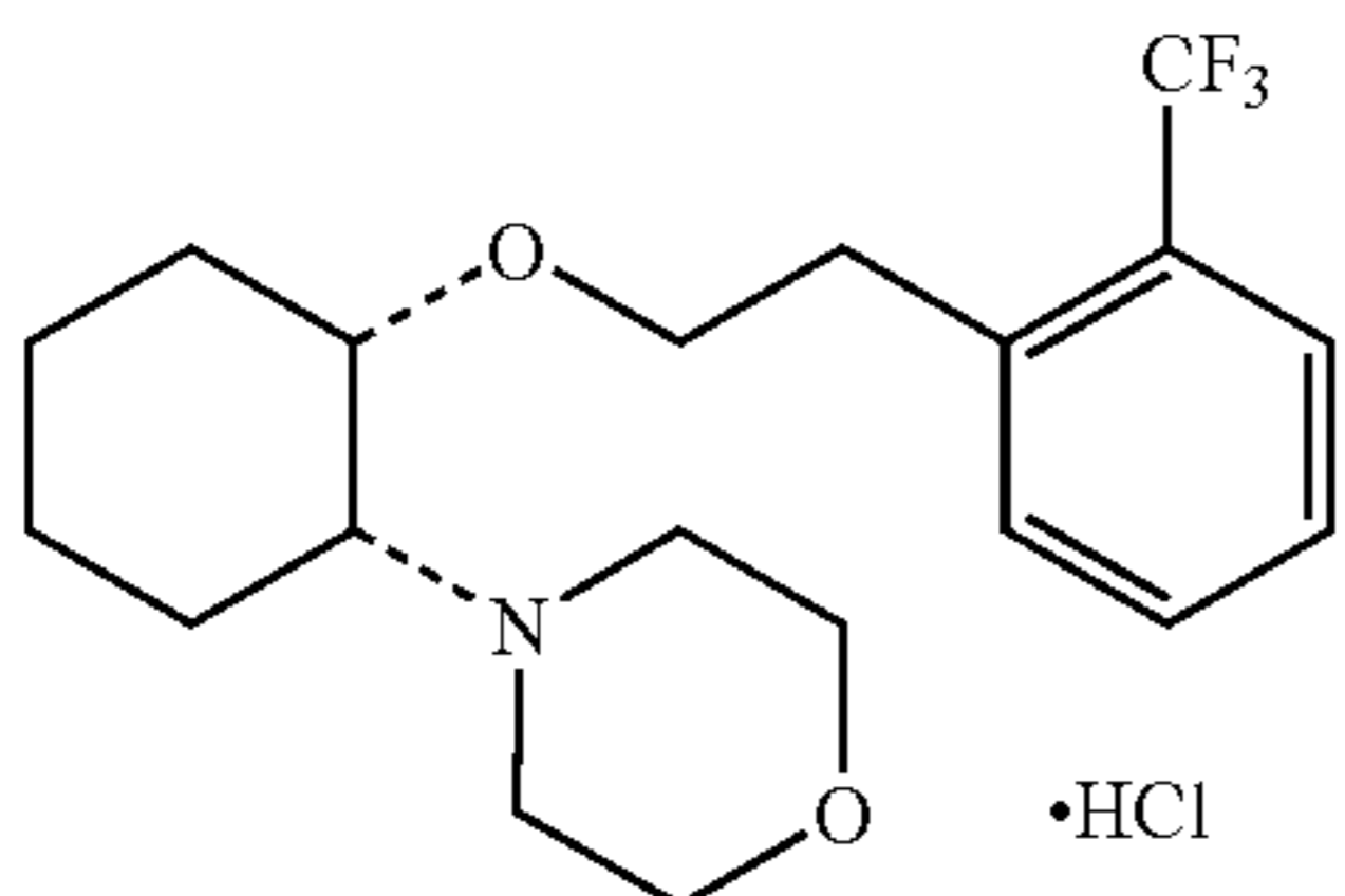
(1R,2S)/(1S,2R)-2-(4-morpholinyl)-1-[(2-trifluoromethyl)phenoxy]cyclohexane monohydrochloride
