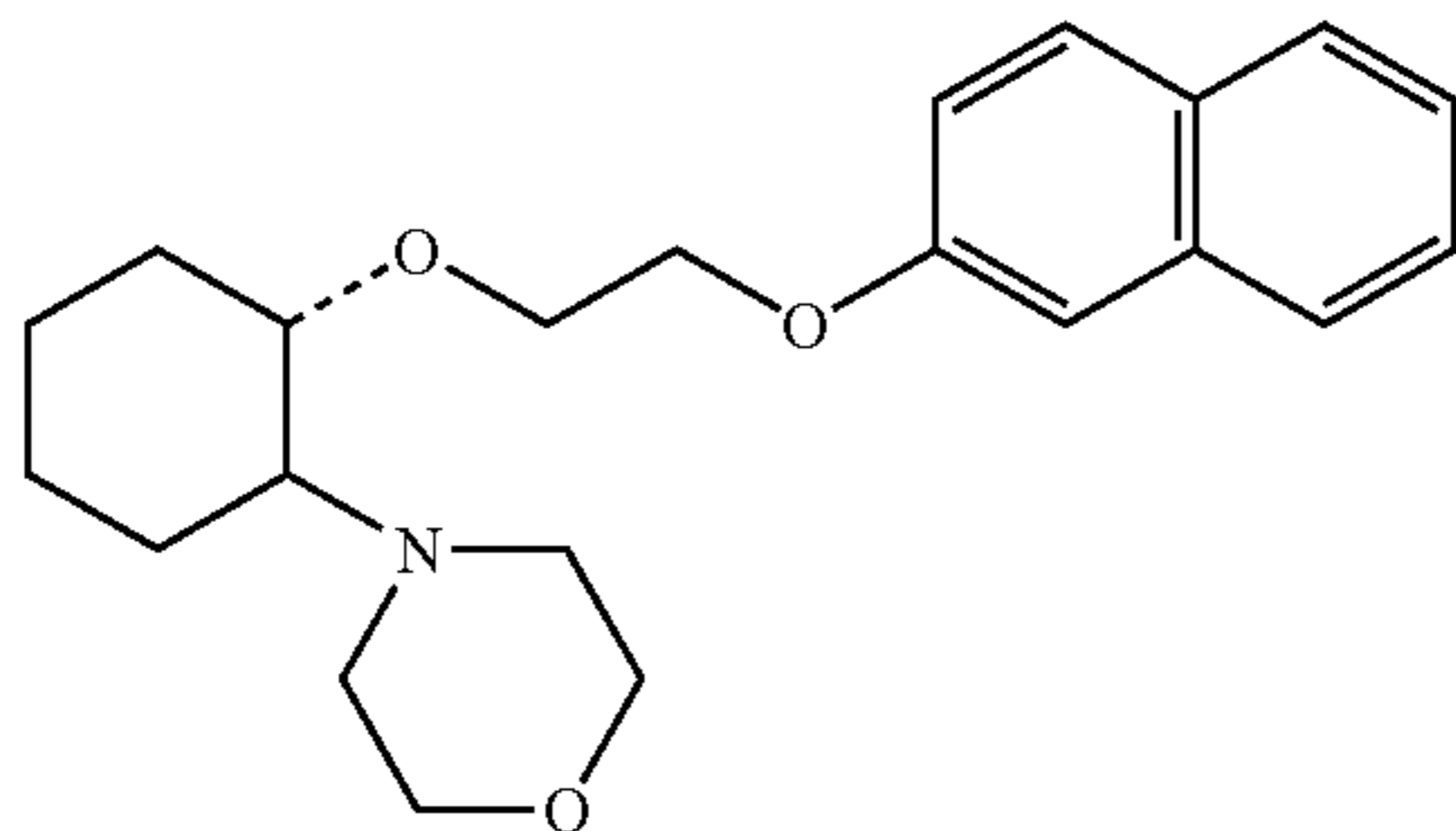
(1R,2R)/(1S,2S)-[2-(4-morpholinyl)-1-[2-(2-naphthoxy)ethoxy]]cyclohexane
