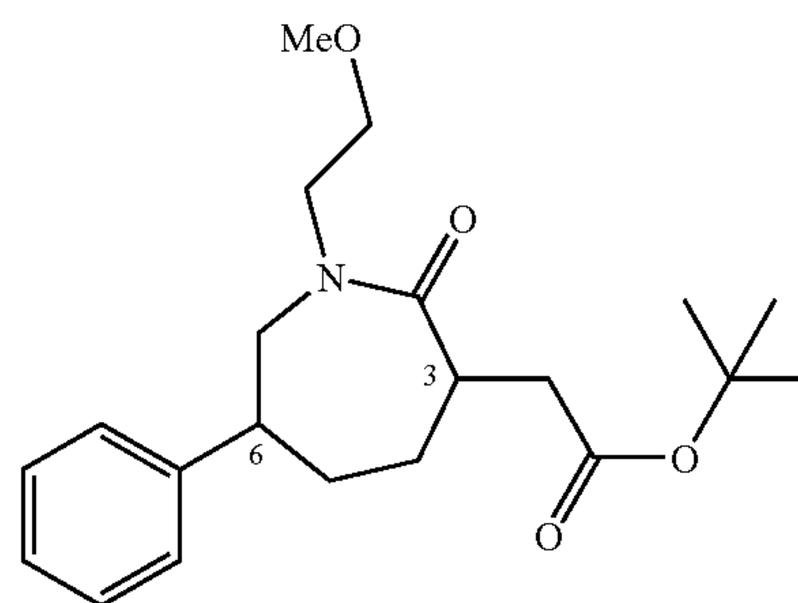
tert-Butyl[1-(2-methoxyethyl)-2-oxo-6-phenylazepan-3-yl]acetate
