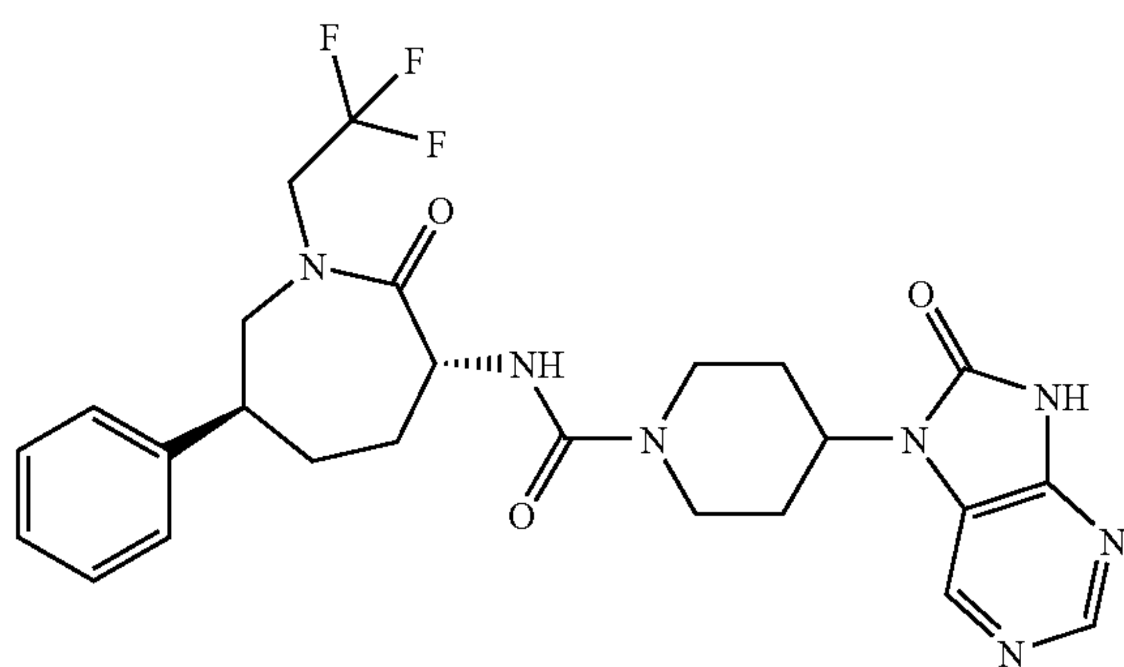
N-[(3R,6S)-6-Phenyl-2-oxo-1-(2,2,2-trifluoroethyl)azepan-3-yl]-4-(8-oxo-8,9-dihydro-7H-purin-7-yl)piperidine-1-carboxamide
