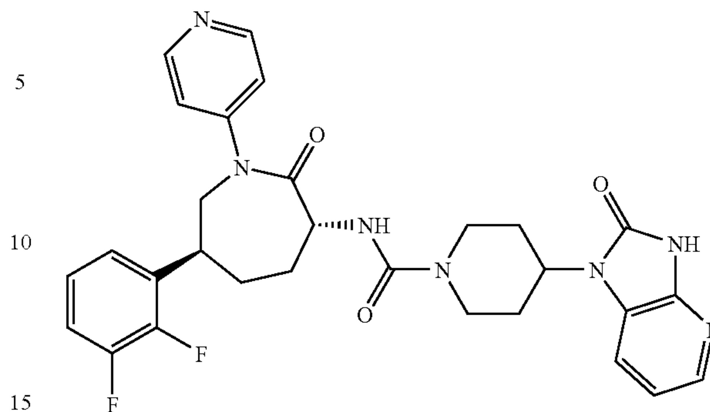
N-[(3R,6S)-6-(2,3-Difluorophenyl)-2-oxo-1-pyridin-4-ylazepan-3-yl]-4-(2-oxo-2,3-dihydro-1H-imidazo[4,5-b]pyridin-1-yl)piperidine-1-carboxamide
