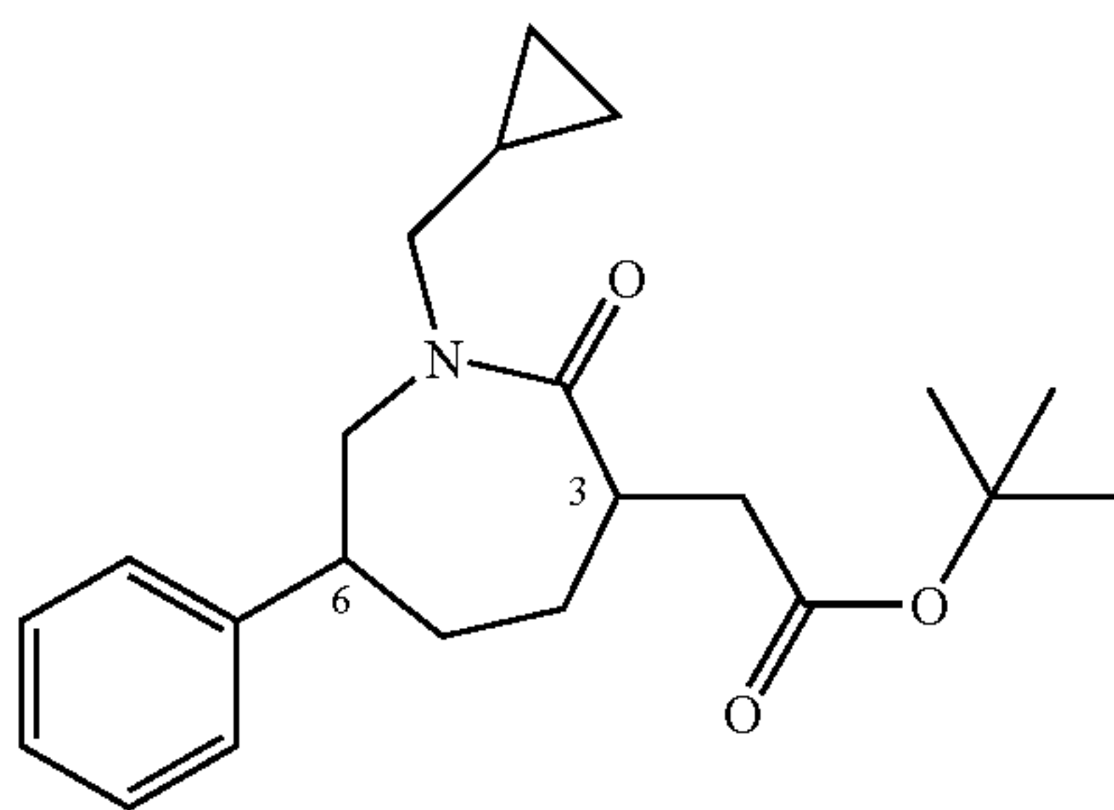
INTERMEDIATE 67
