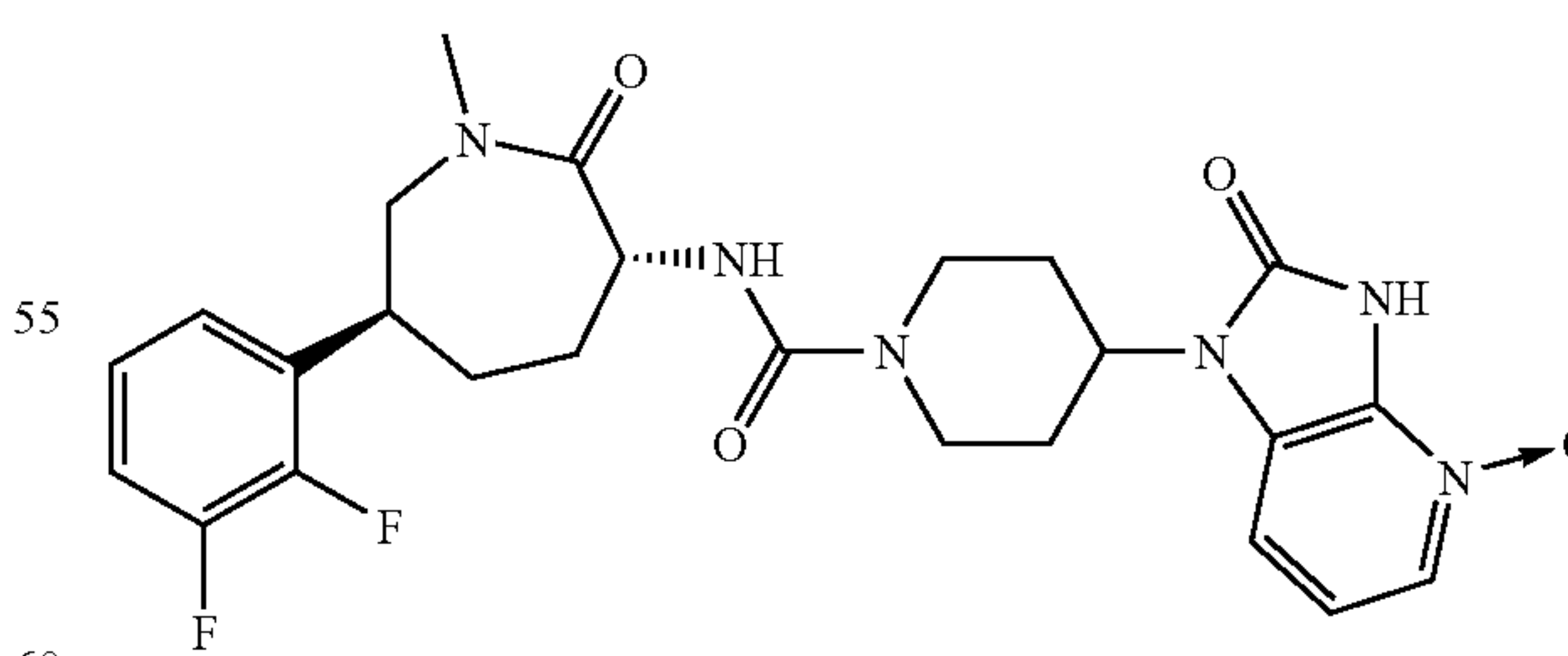
N-[(3R,6S)-6-(2,3-Difluorophenyl)-1-methyl-2-oxazepan-3-yl]-4-(4-oxido-2-oxo-2,3-dihydro-1H-imidazo[4,5-b]pyridin-1-yl)piperidine-1-carboxamide
