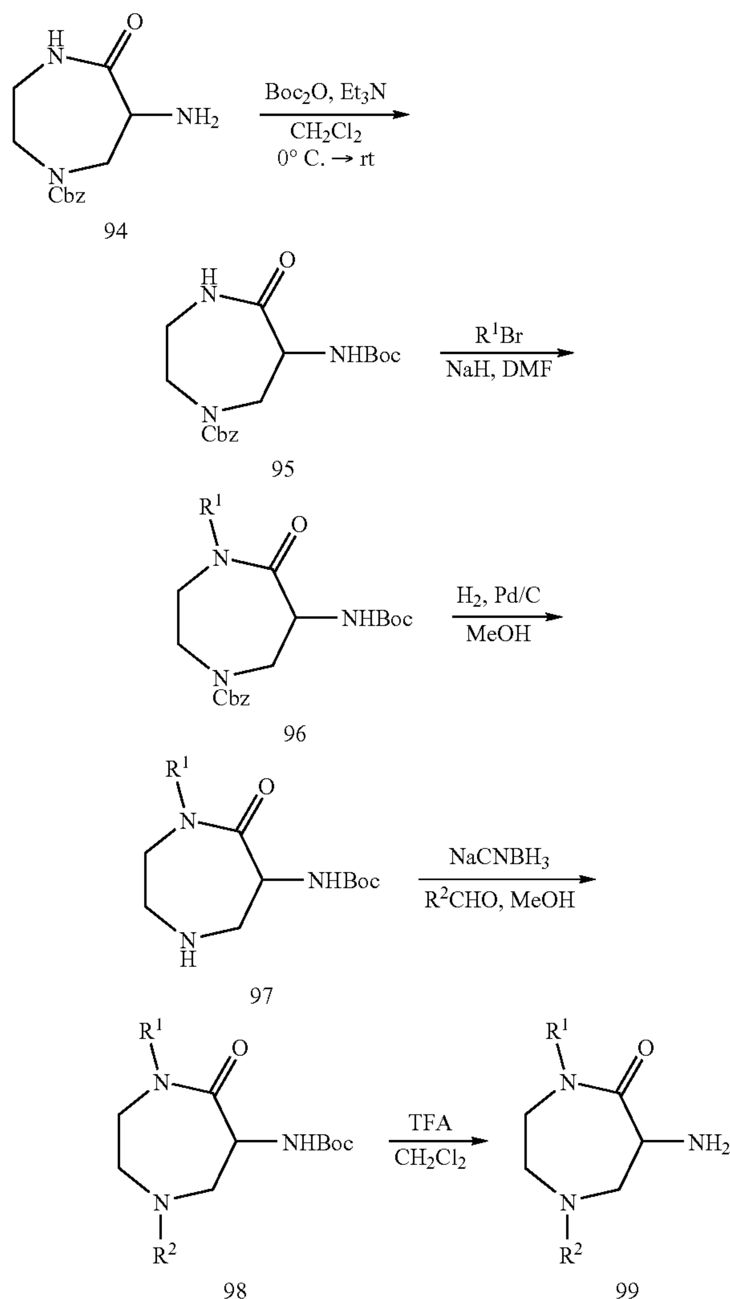
SCHEME 16
