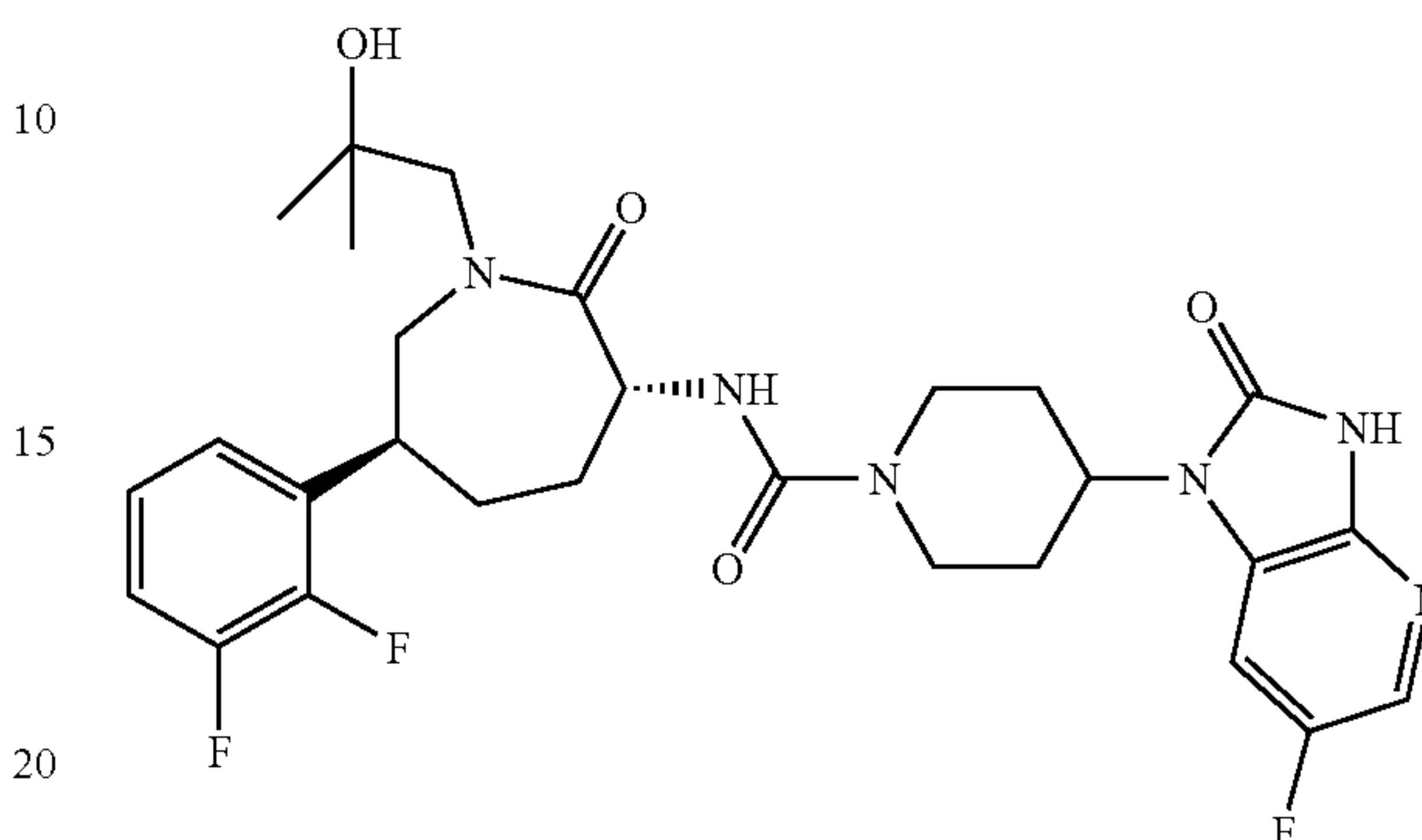
N-[(3R,6S)-6-(2,3-Difluorophenyl)-1-(2-hydroxy-2-methylpropyl)-2-oxazepan-3-yl]-4-(6-fluoro-2-oxo-2,3-dihydro-1H-imidazo[4,5-b]pyridin-1-yl)piperidine-1-carboxamide
