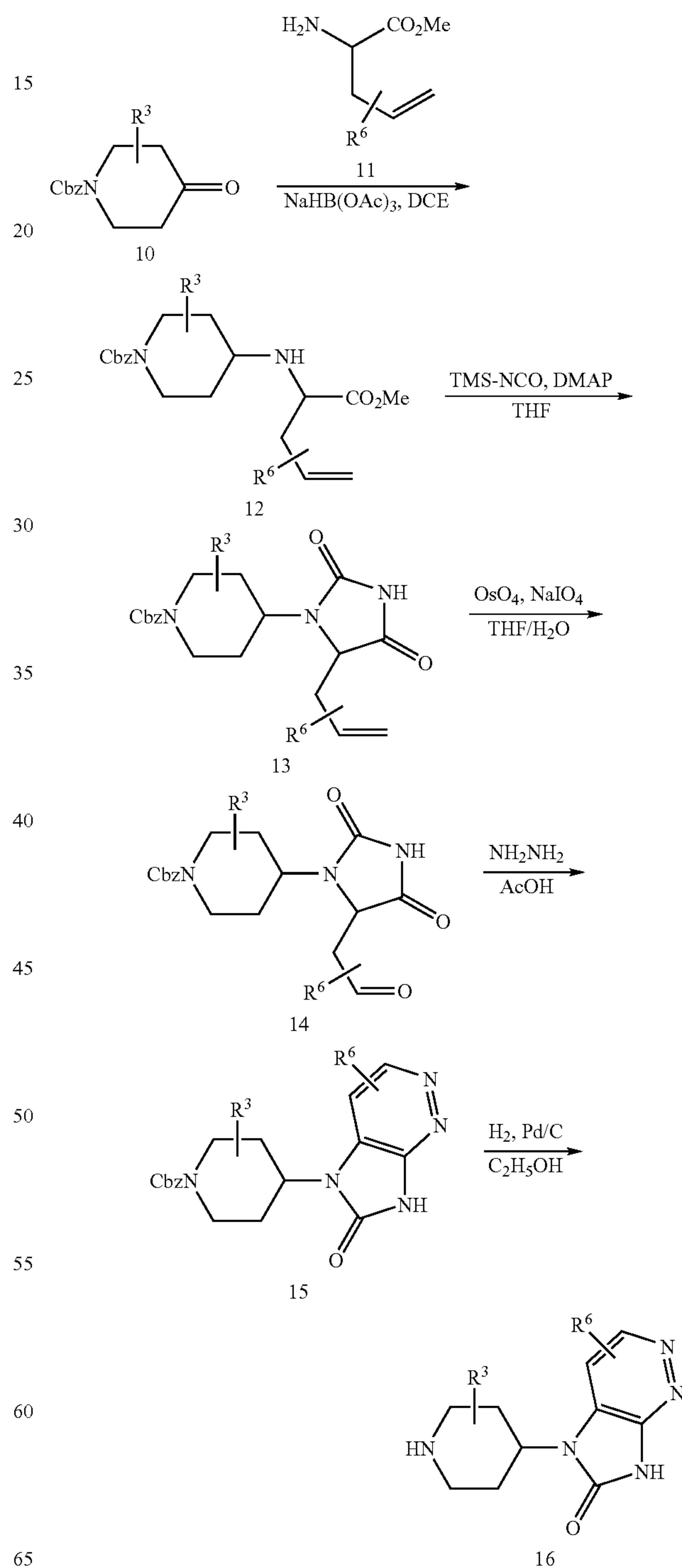
SCHEME 3
