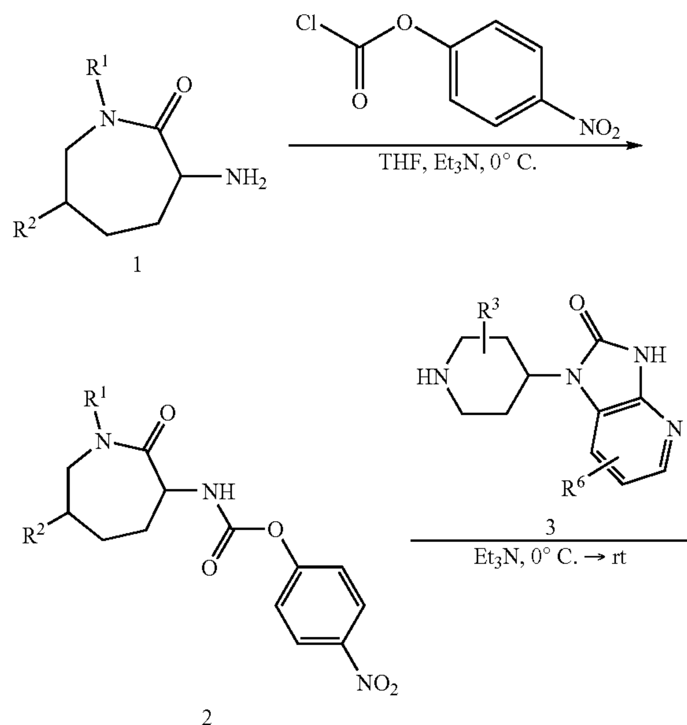
SCHEME 1
