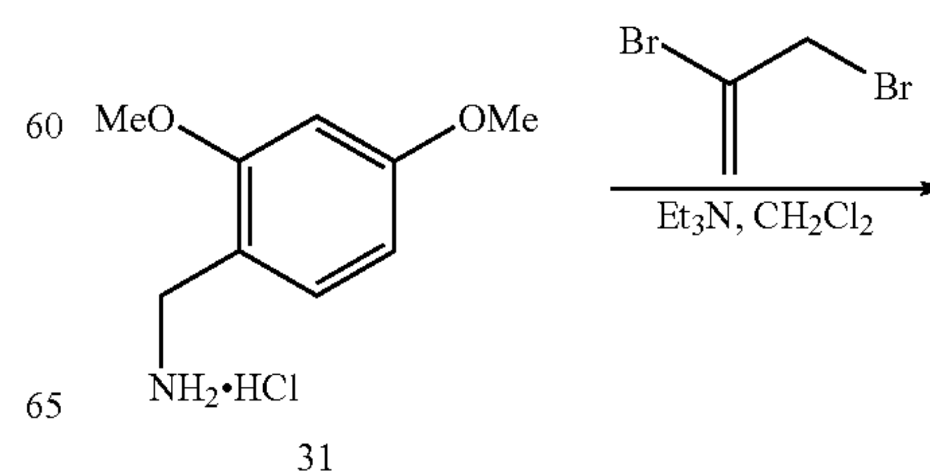
SCHEME 7
