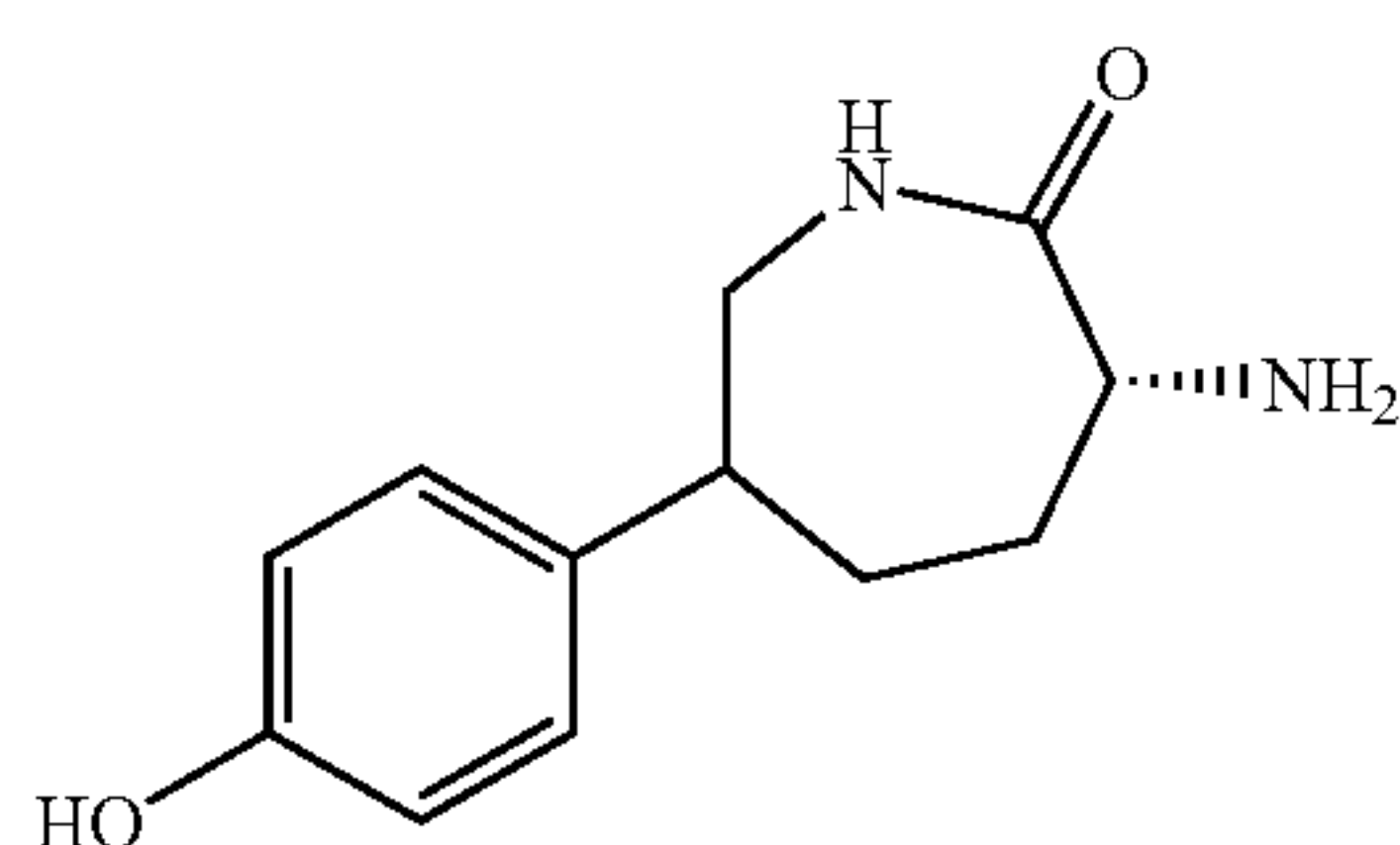
(3R)-3-Amino-6-(4-hydroxyphenyl)azepan-2-one
