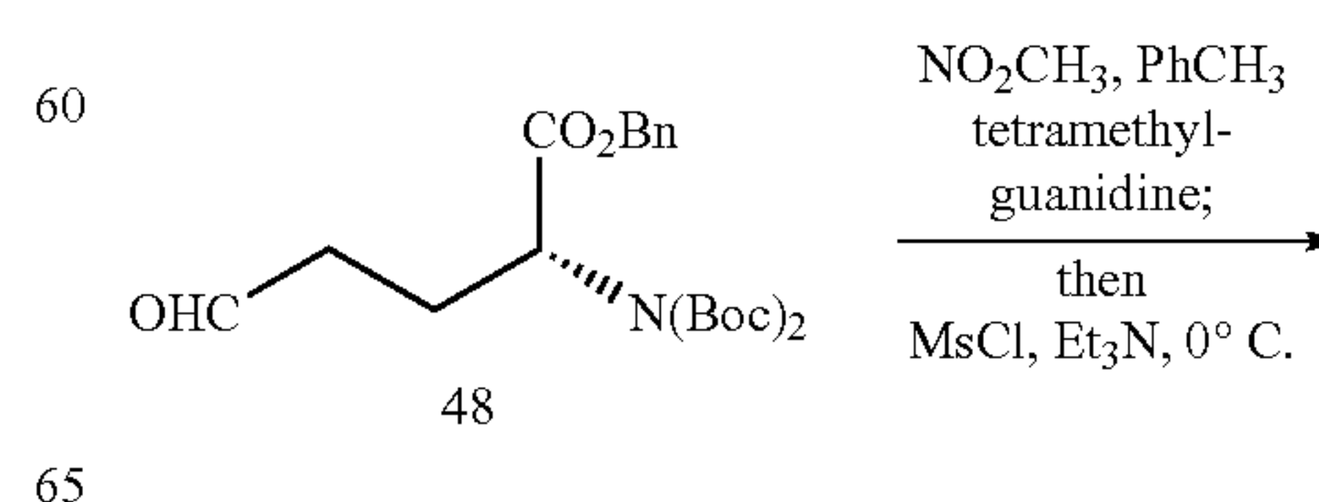
SCHEME 8
