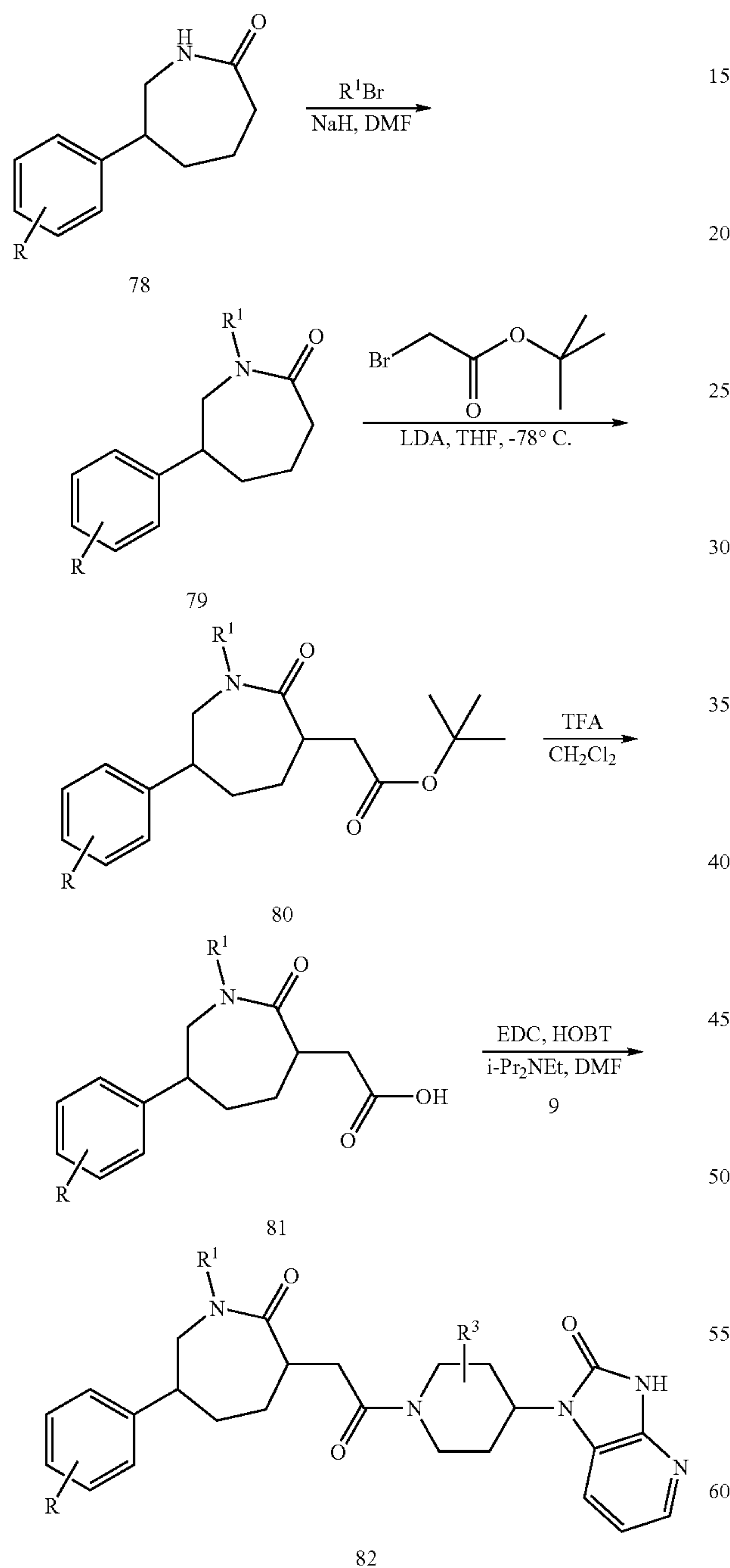
SCHEME 14
