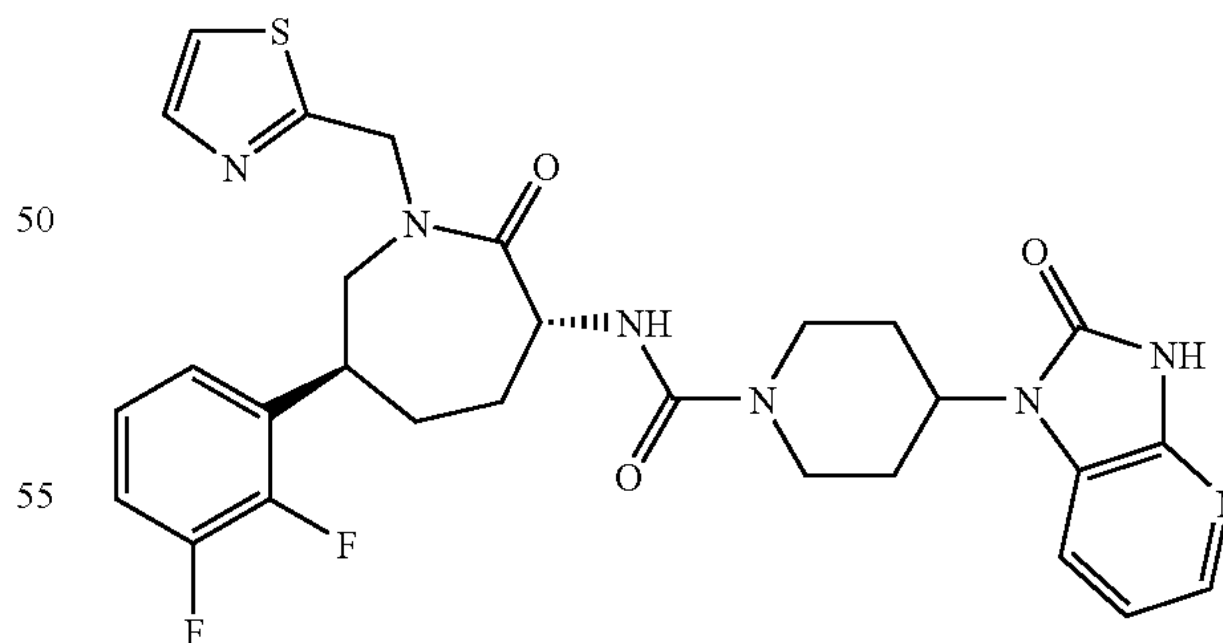
N-[(3R,6S)-6-(2,3-Difluorophenyl)-2-oxo-1-(1,3-thiazol-2-ylmethyl)azepan-3-yl]-4-(2-oxo-2,3-dihydro-1H-imidazo[4,5-b]pyridin-1-yl)piperidine-1-carboxamide
