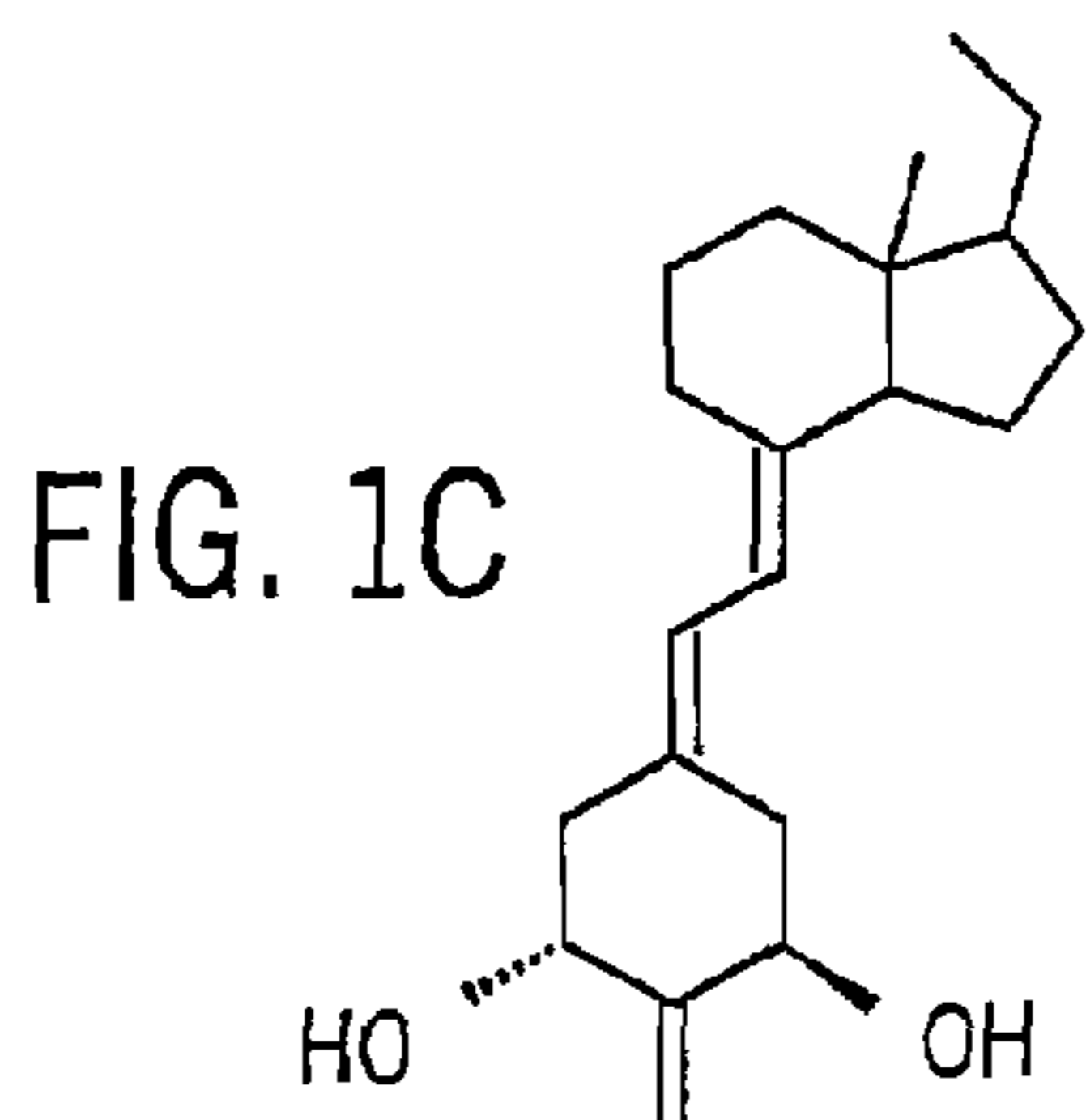
1 \alpha -HYDROXY-2-METHYLENE-19-NOR-PREGNACALCIFEROL A.K.A 2-Mpregna
