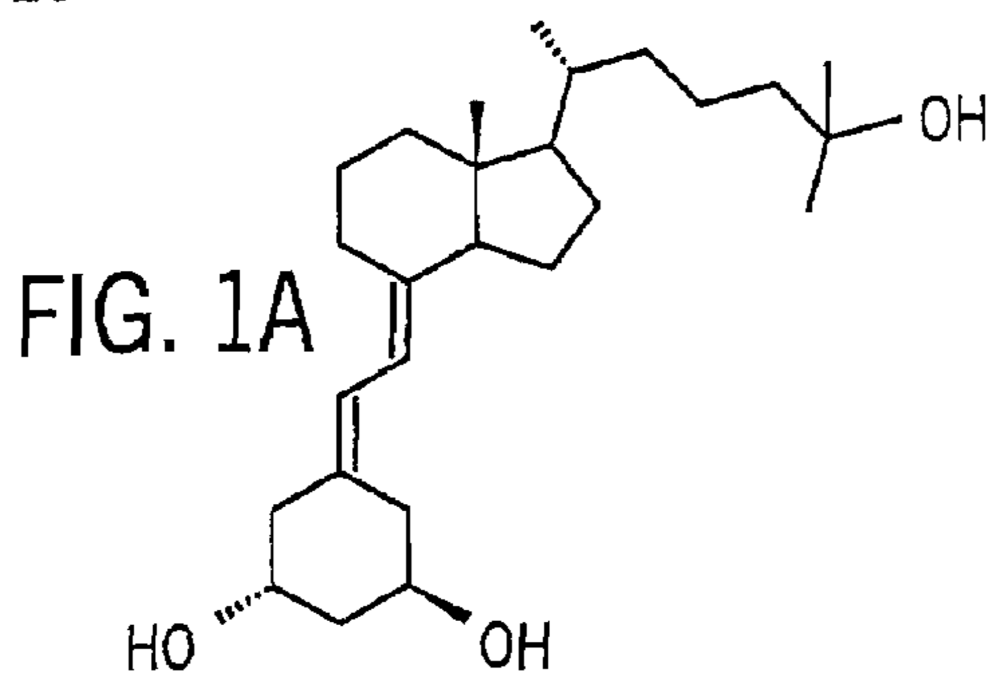
1 \alpha , 25-DIHYDROXY-19-NORVITAMIN D3
