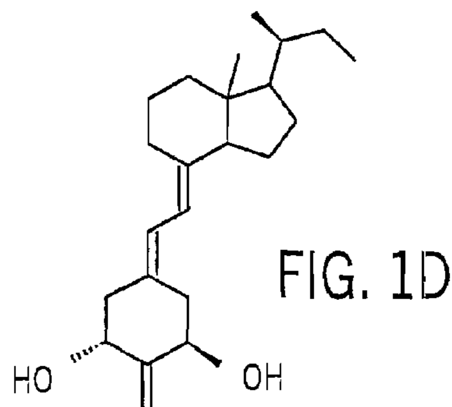
(20S)-1 \alpha -HYDROXY-2-METHYLENE-19-NOR-BISHOMOPREGNACALCIFEROL A.K.A 2-MbisP
