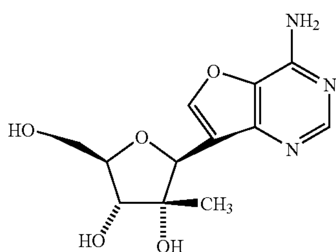
4-Amino-7-(2-C-methyl-β-D-ribofuranosyl)-furo[3,2-d]pyrimidine
