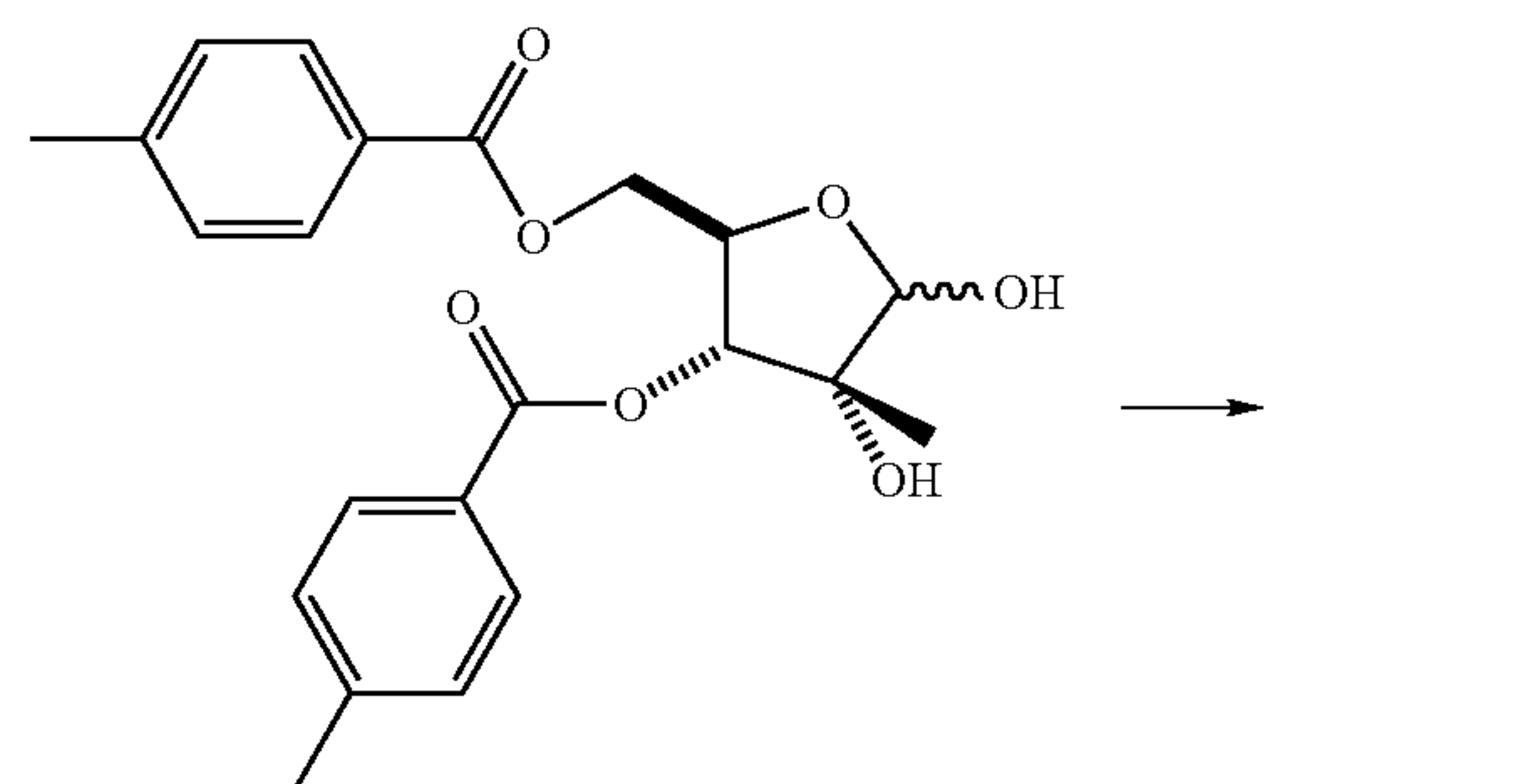
Scheme 4C
