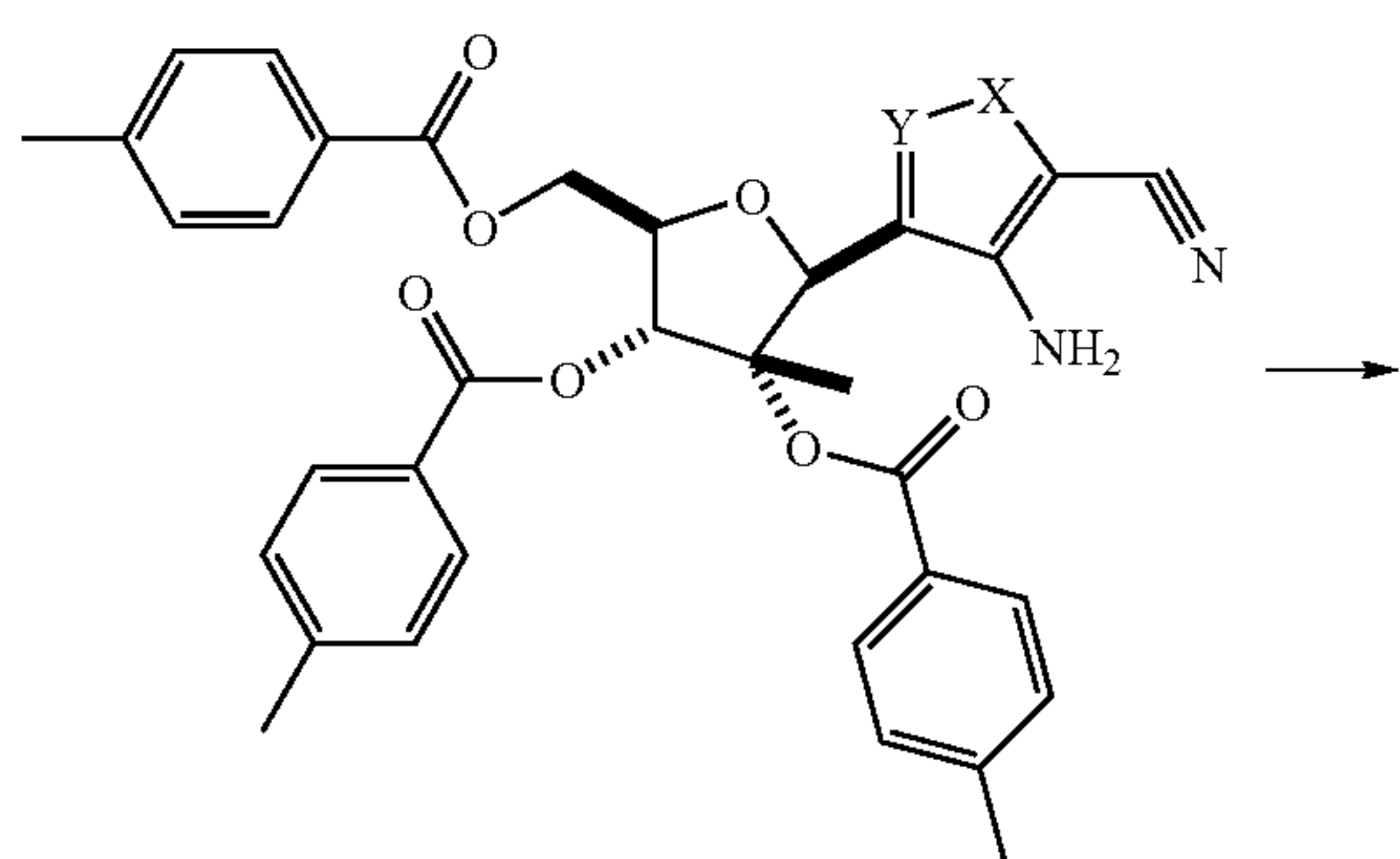
Scheme 7B
