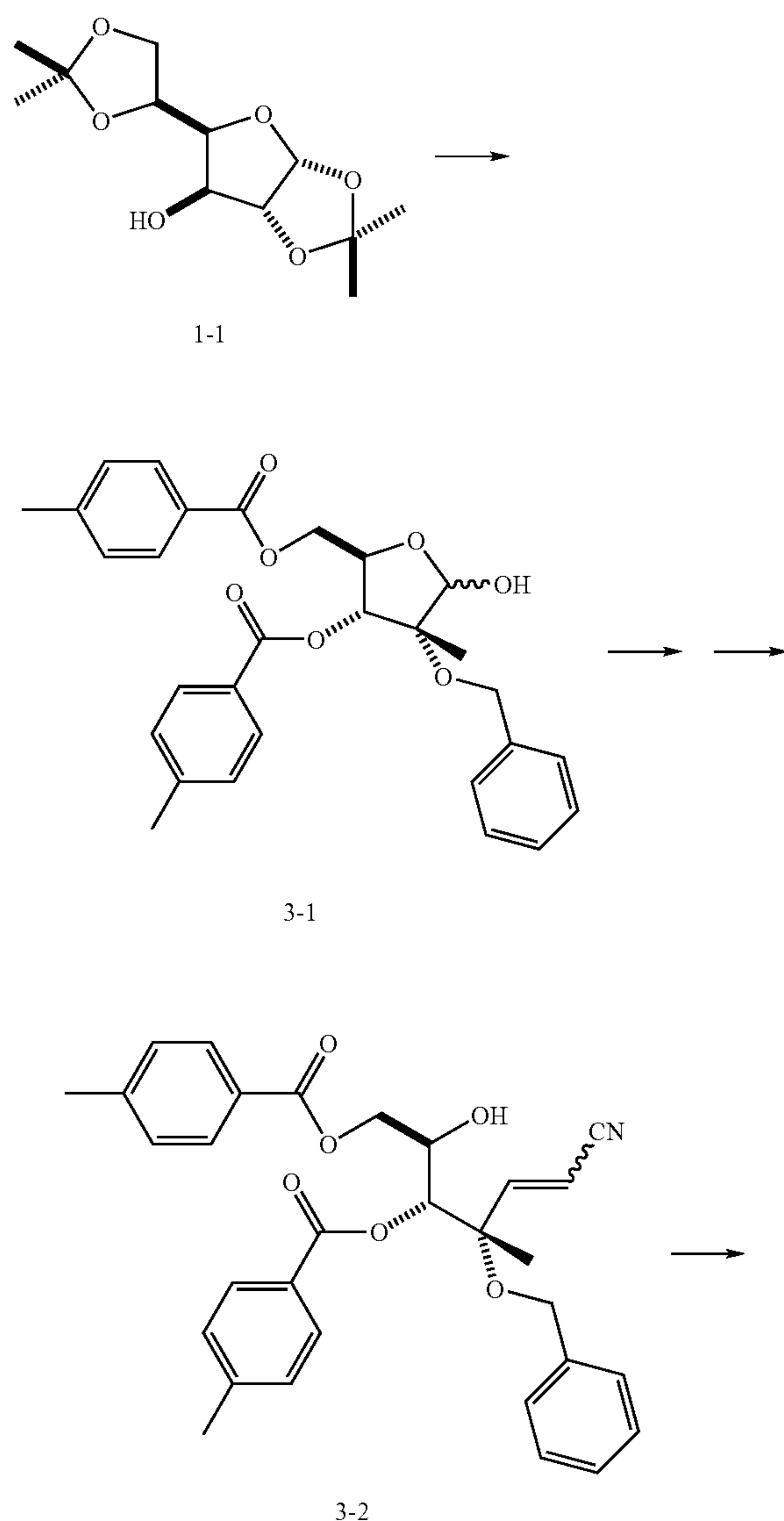
SCHEME 3
