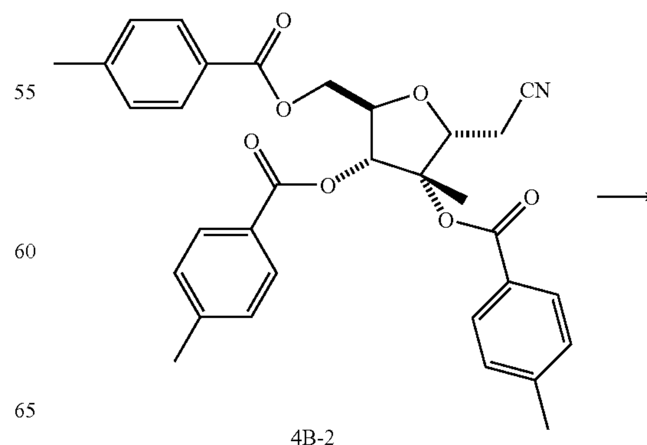
Scheme 5B
