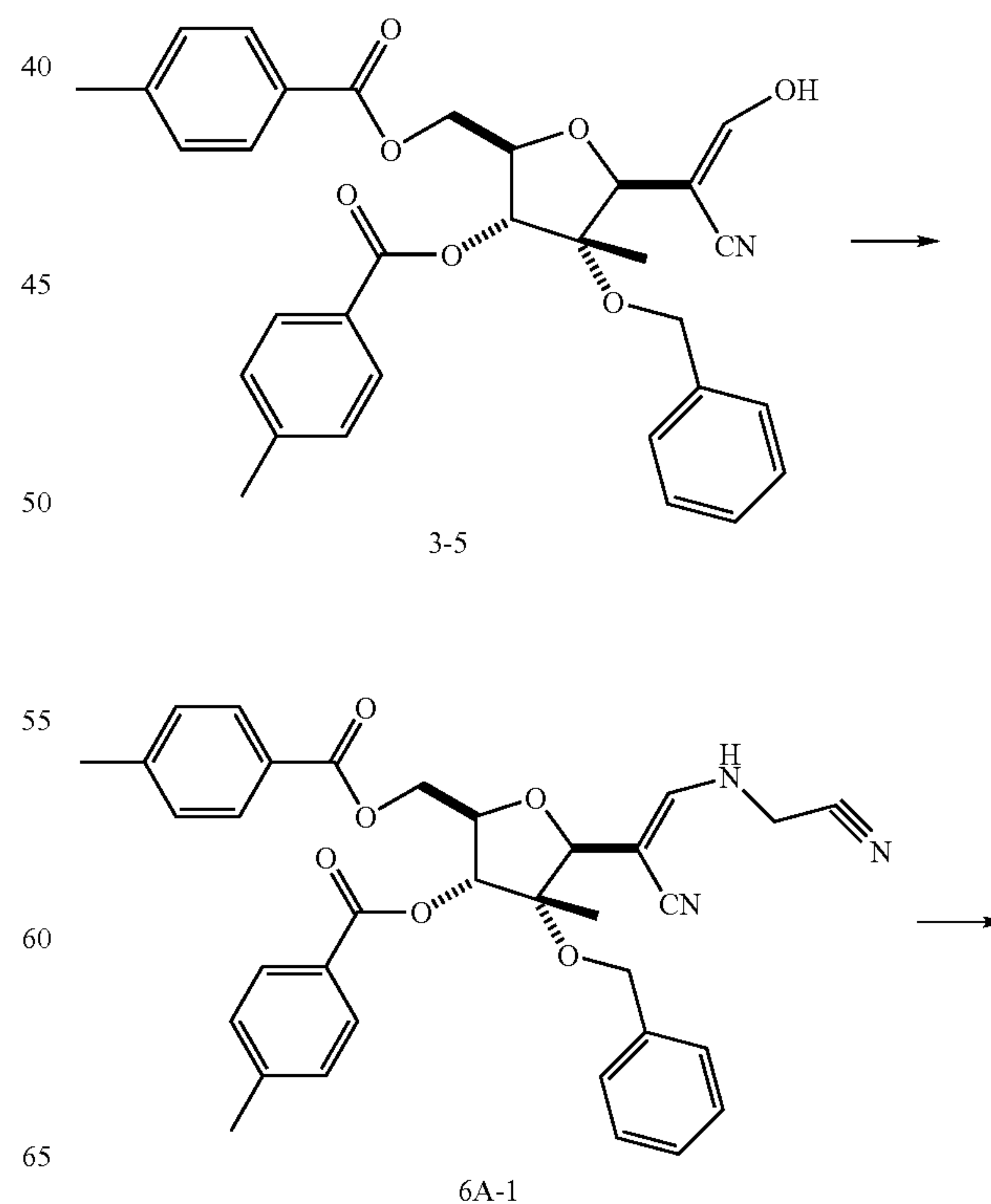
SCHEME 6A
