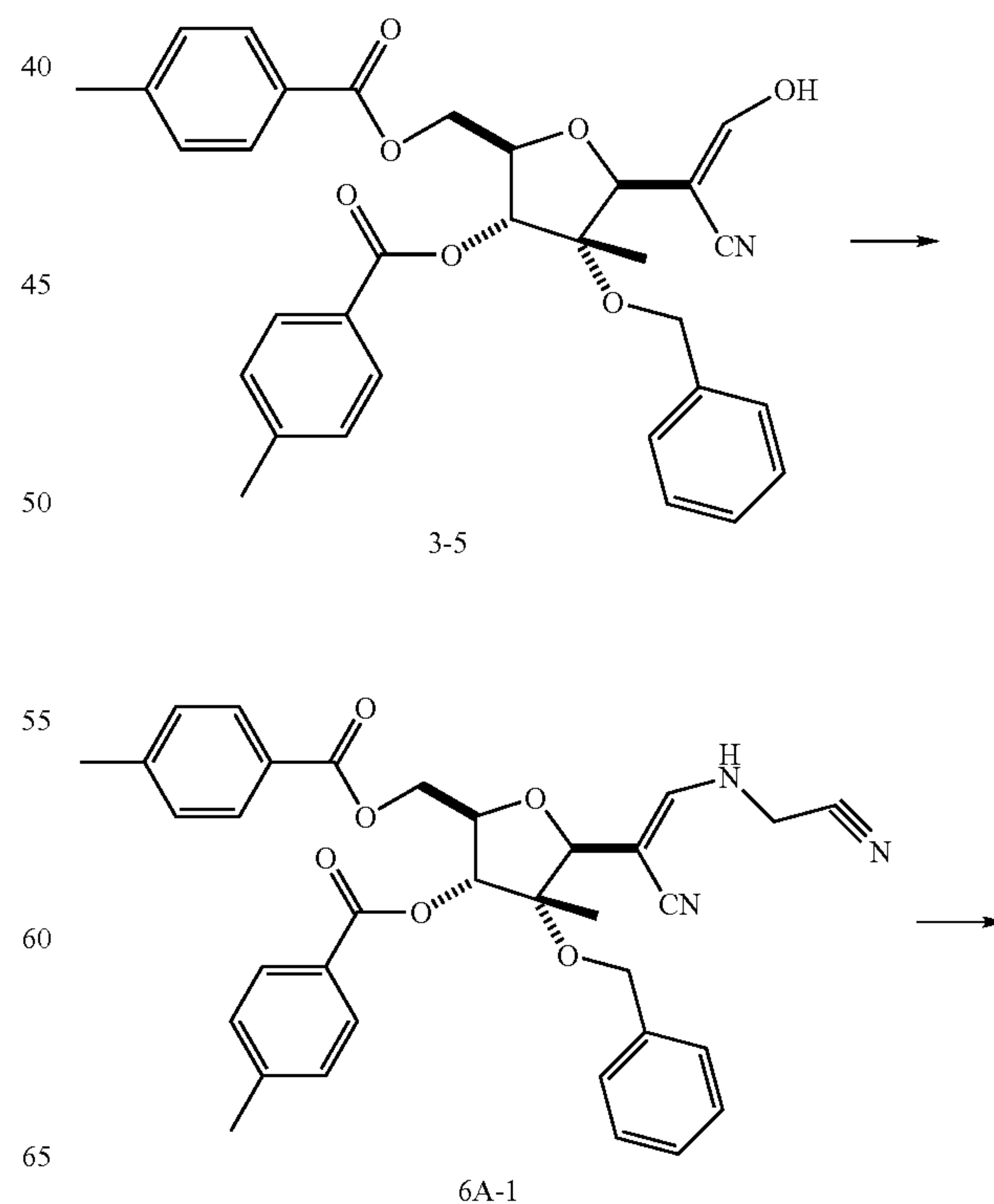
SCHEME 6A
