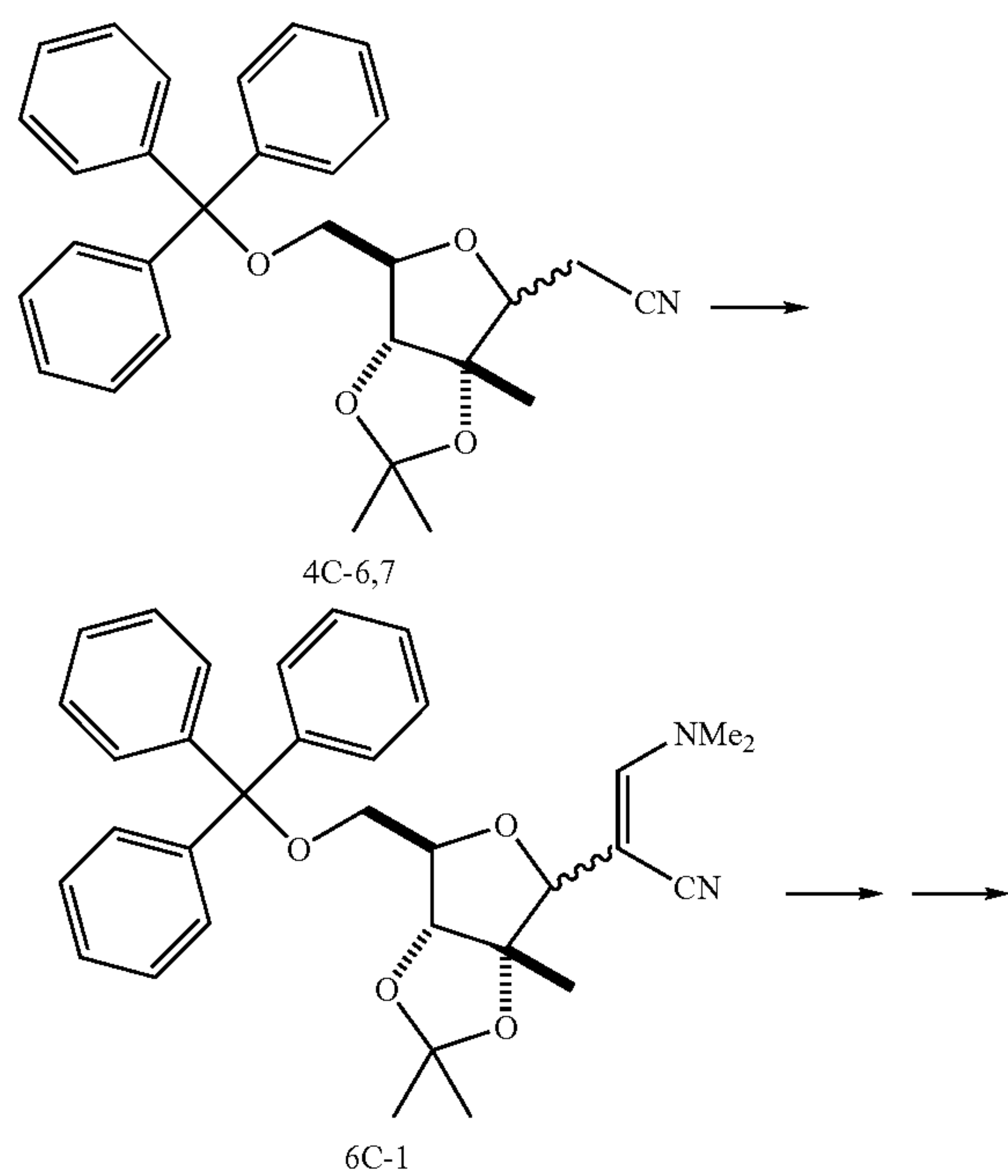
Scheme 6C
