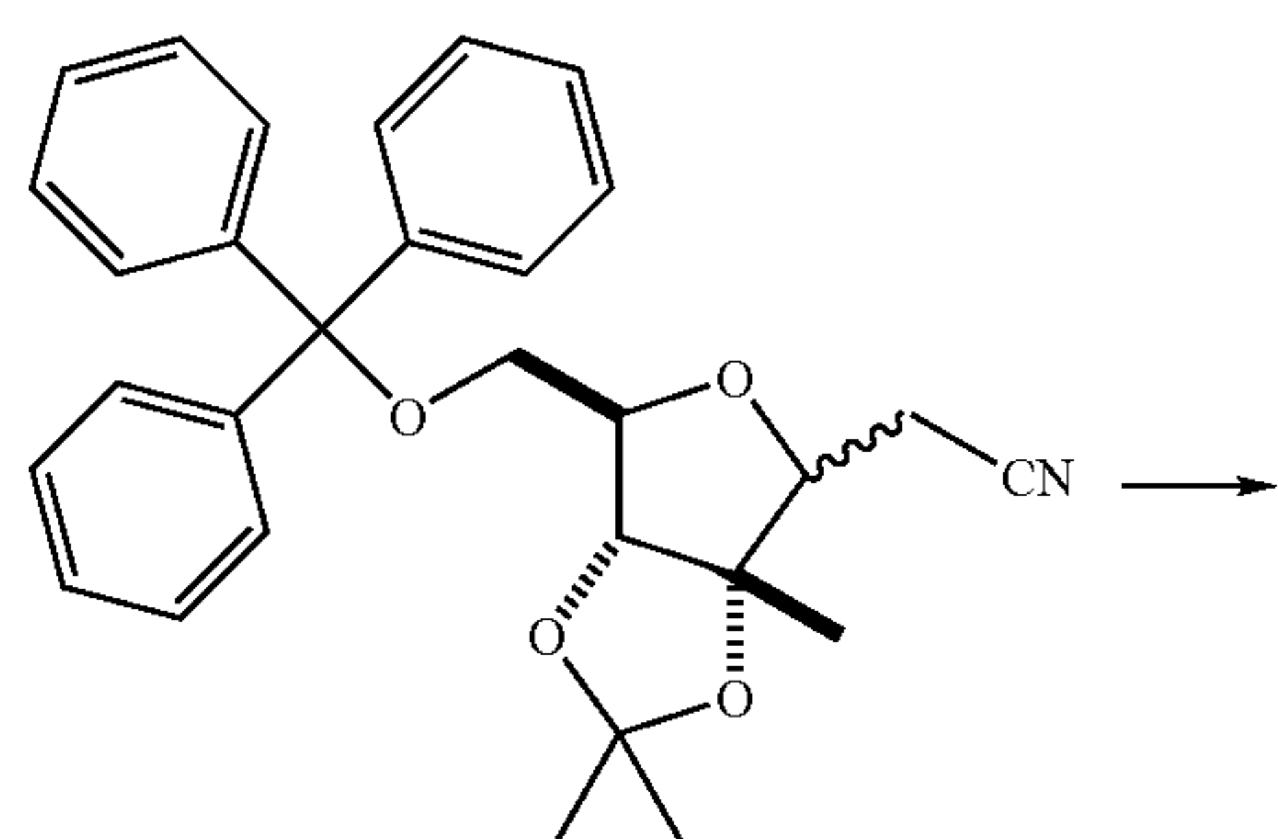
Scheme 6C
