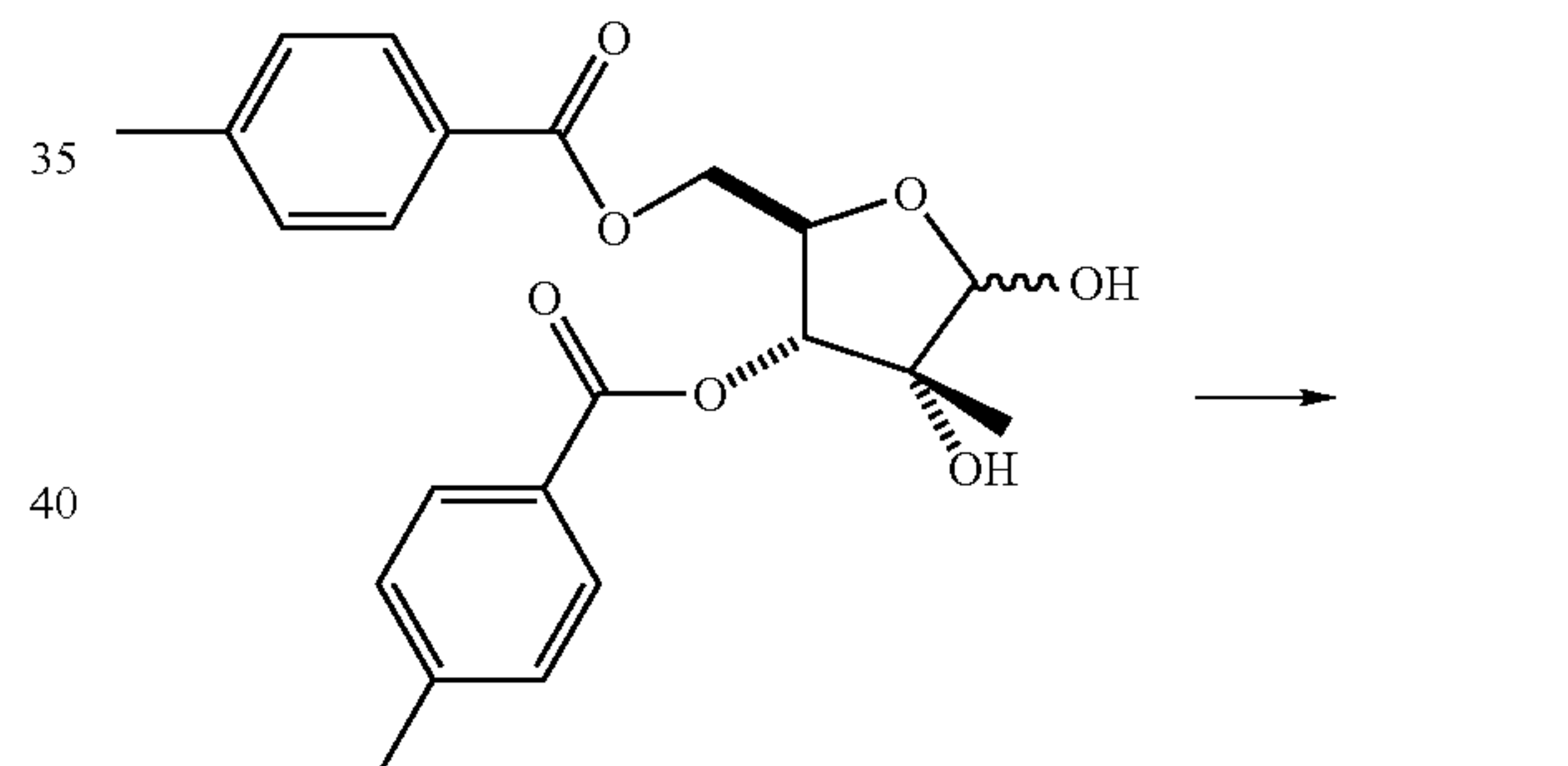
Scheme 4C
