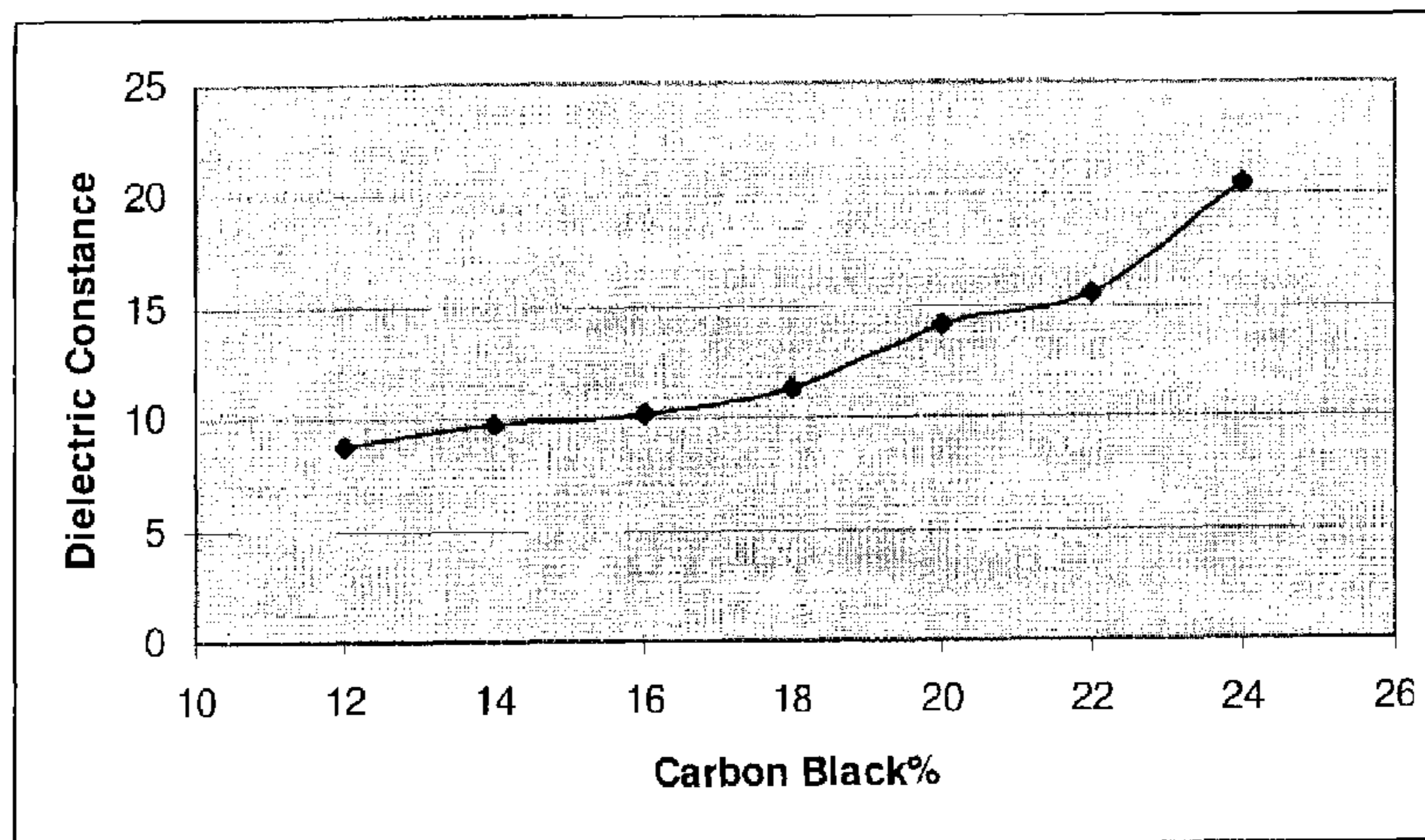
Dielectric Constance vs. Carbon Black Percent
