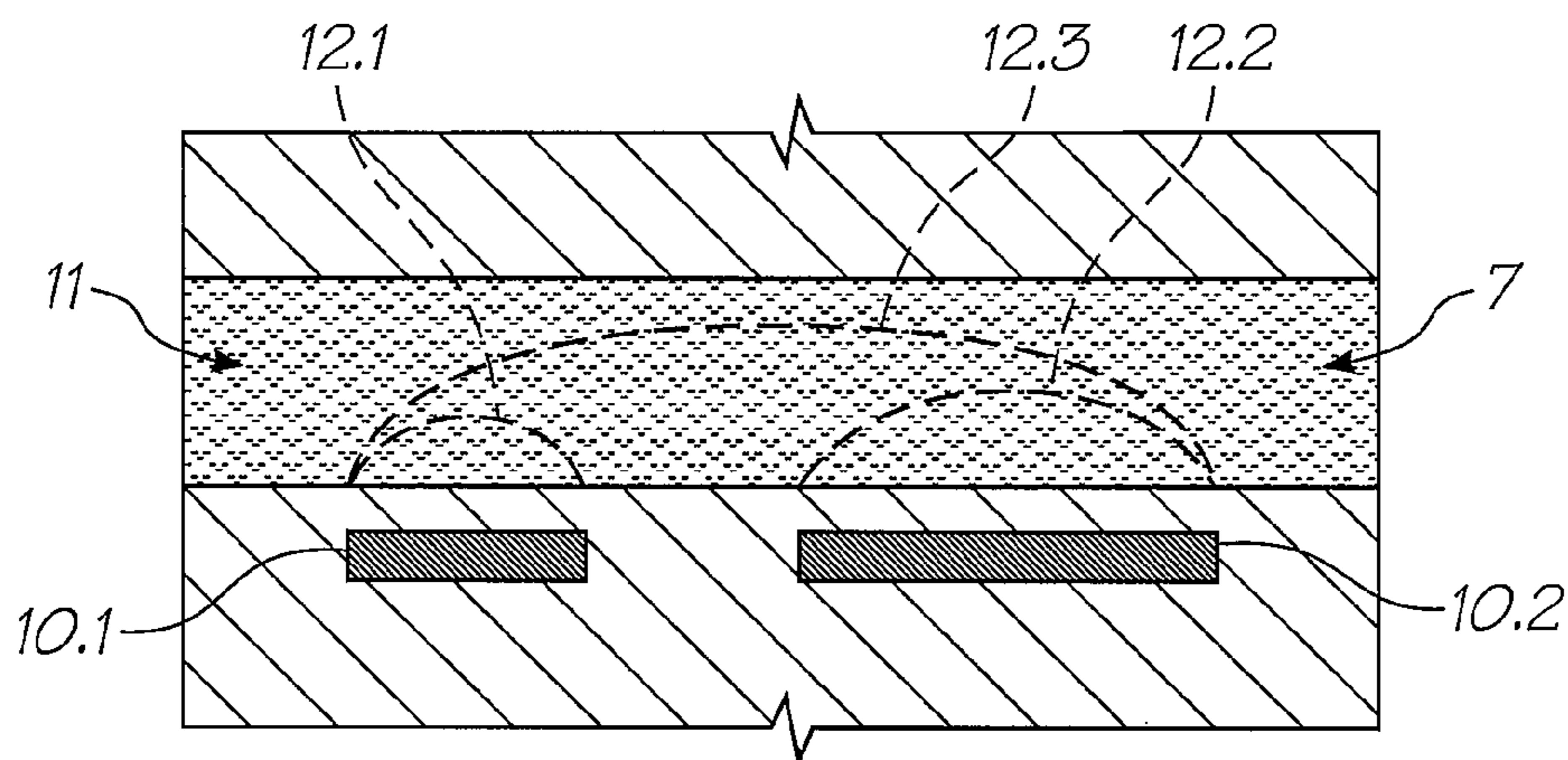
FIG. 52 (PRIOR ART)
