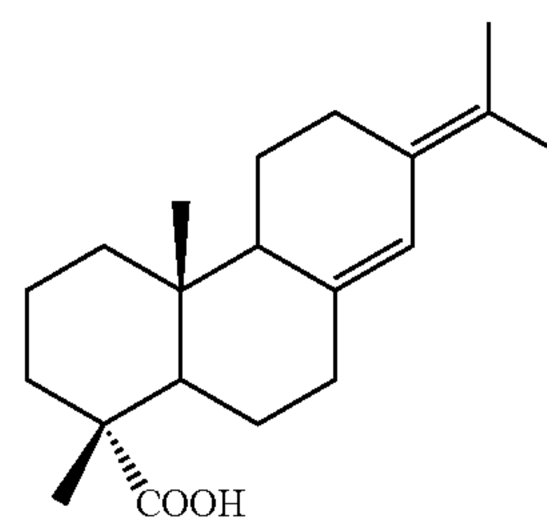
Neo-abietic acid
