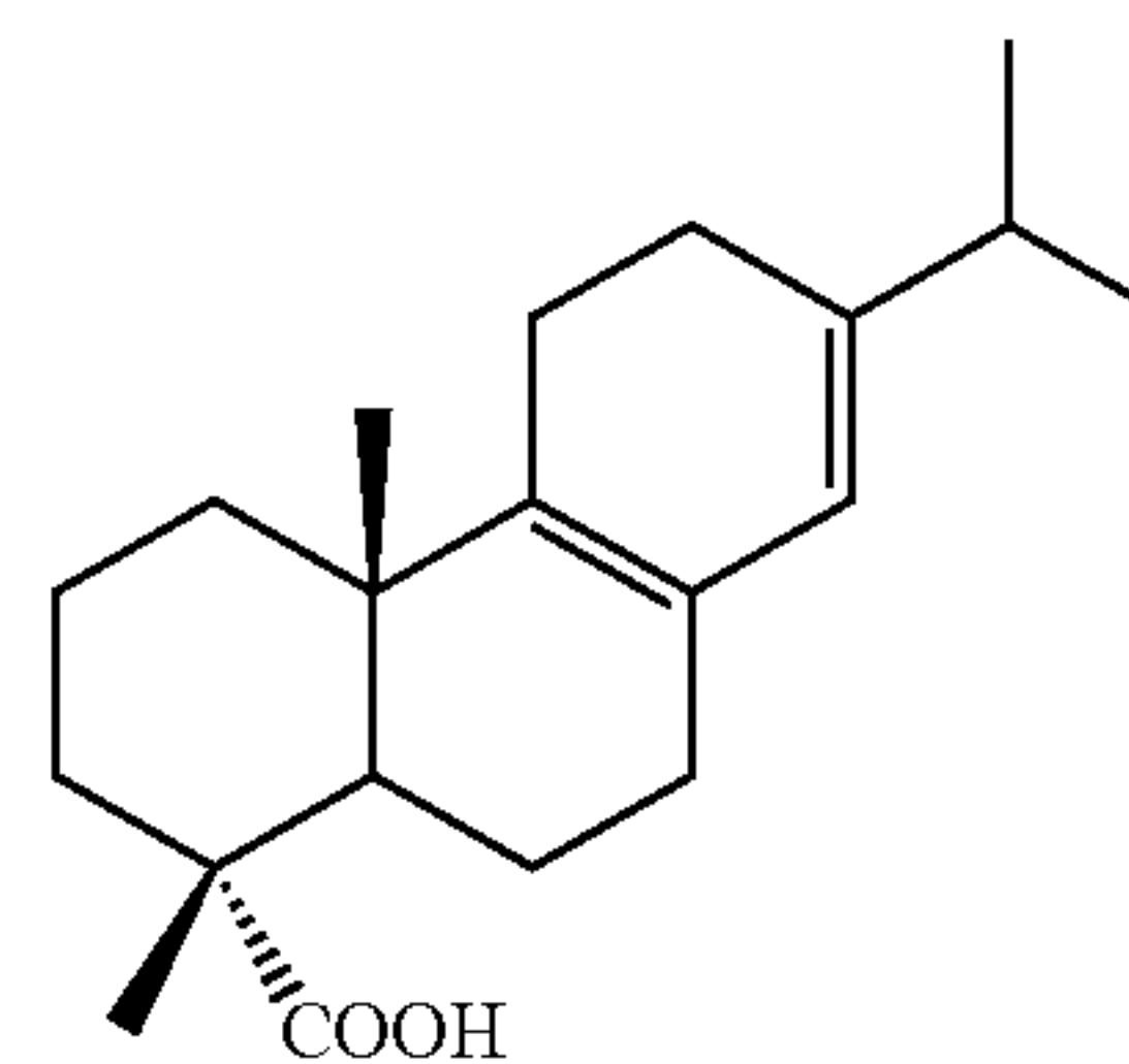
Palustric acid
