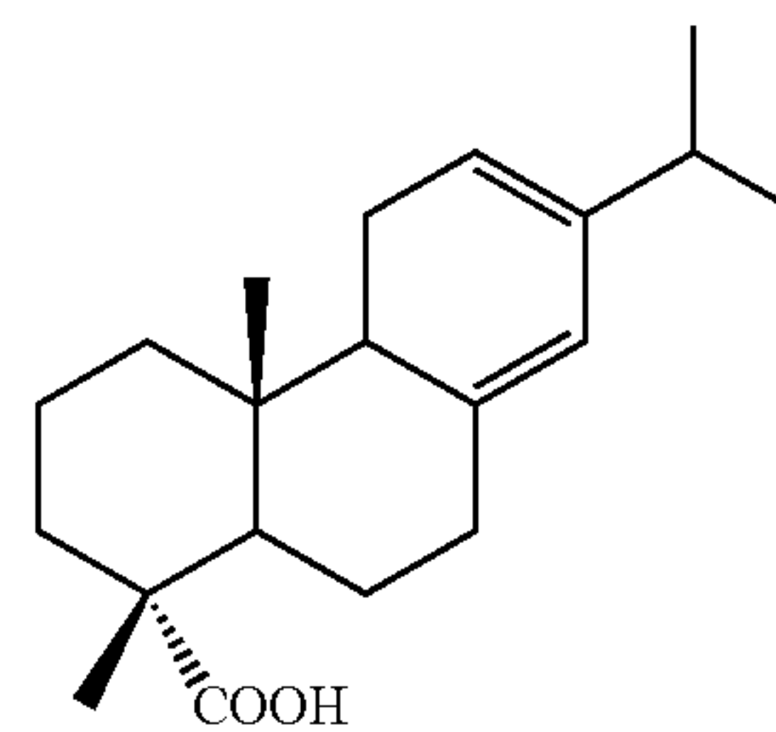
Levopimaric acid
