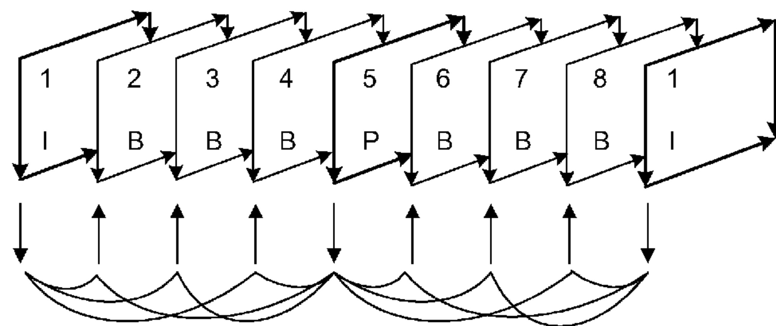
Bidirectional Prediction Figure 3b (Prior Art)
