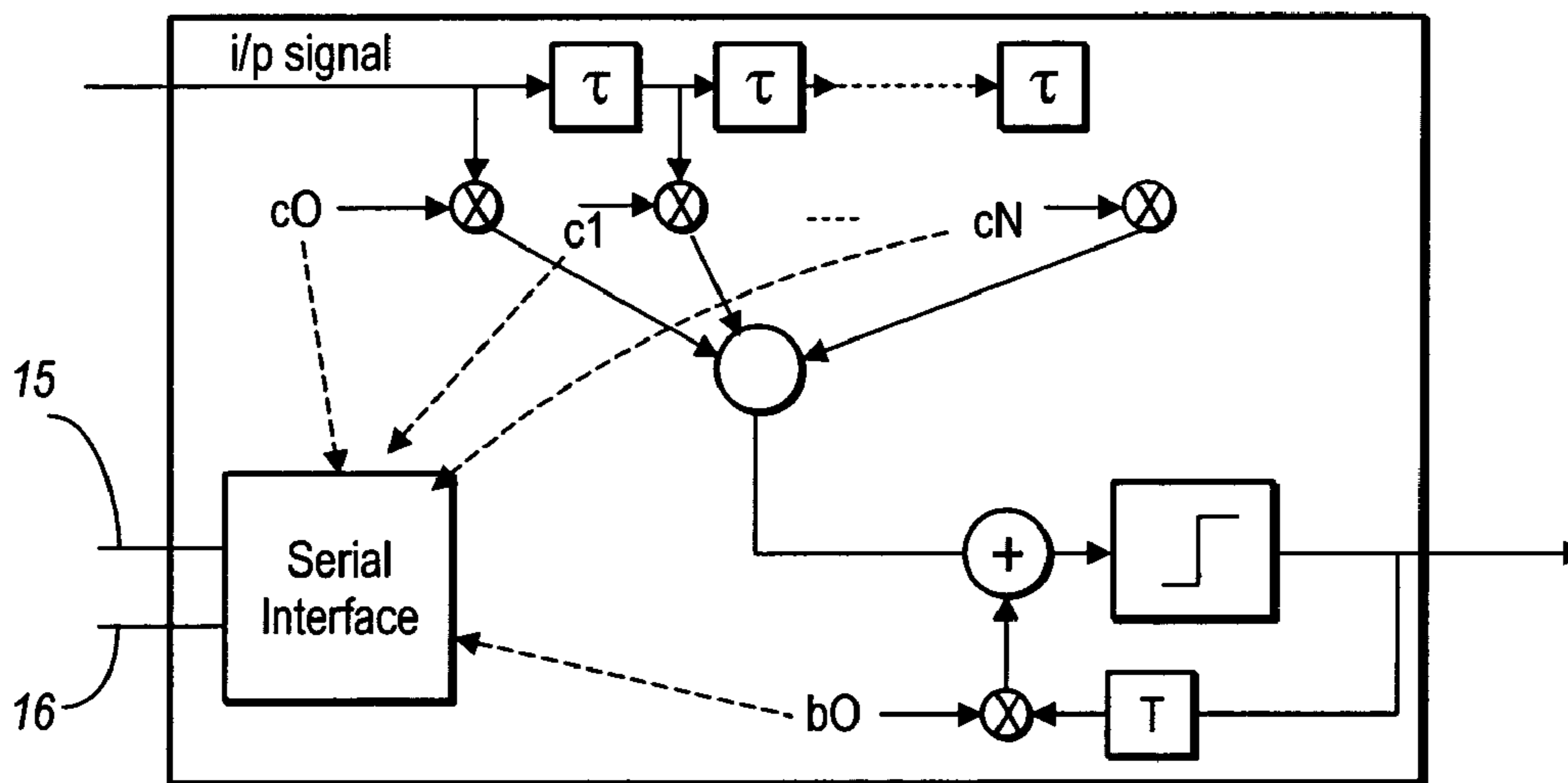
Fig. 2 (Prior Art)
