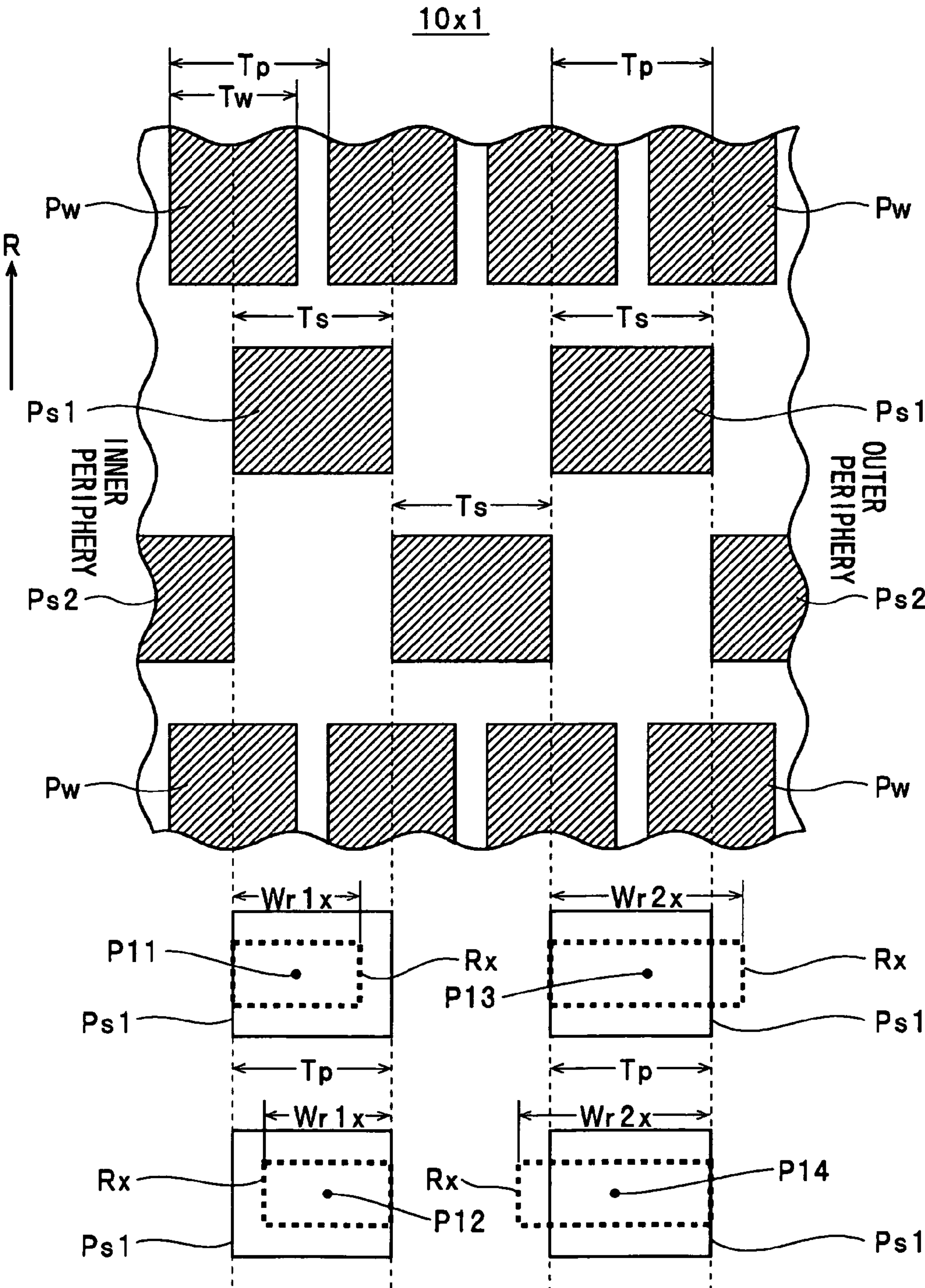
F I G . 2 2 RELATED ART
