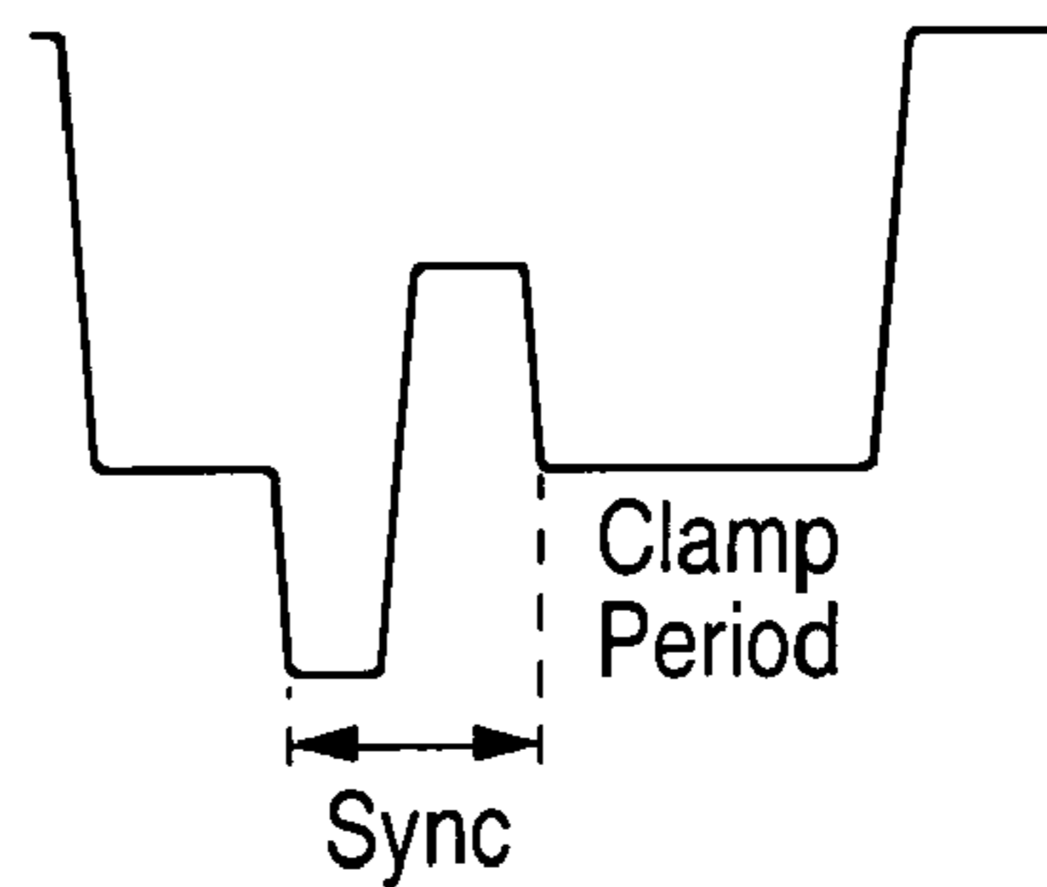
FIG. 5 (PRIOR ART)
