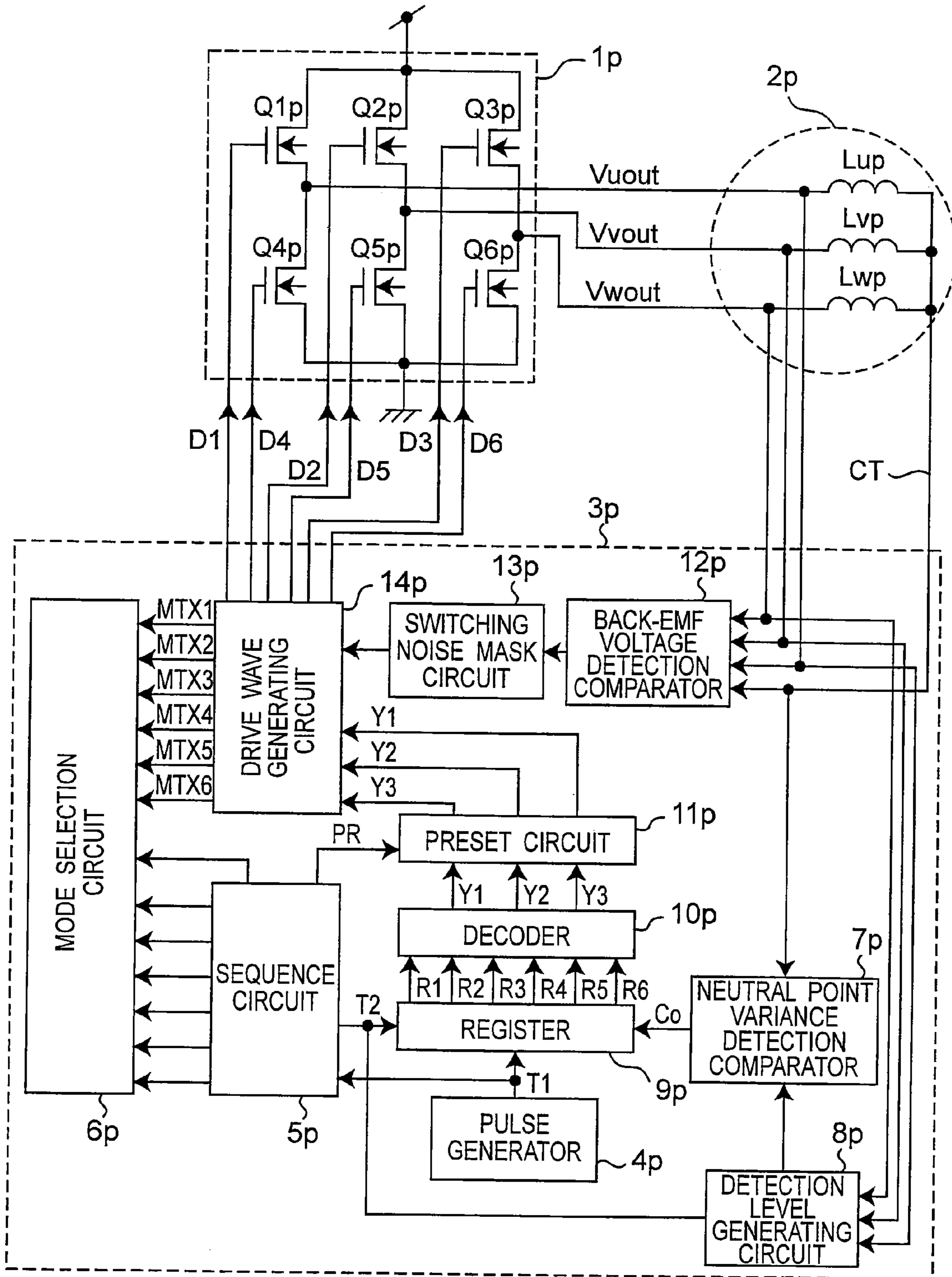
Fig.35 PRIOR ART
