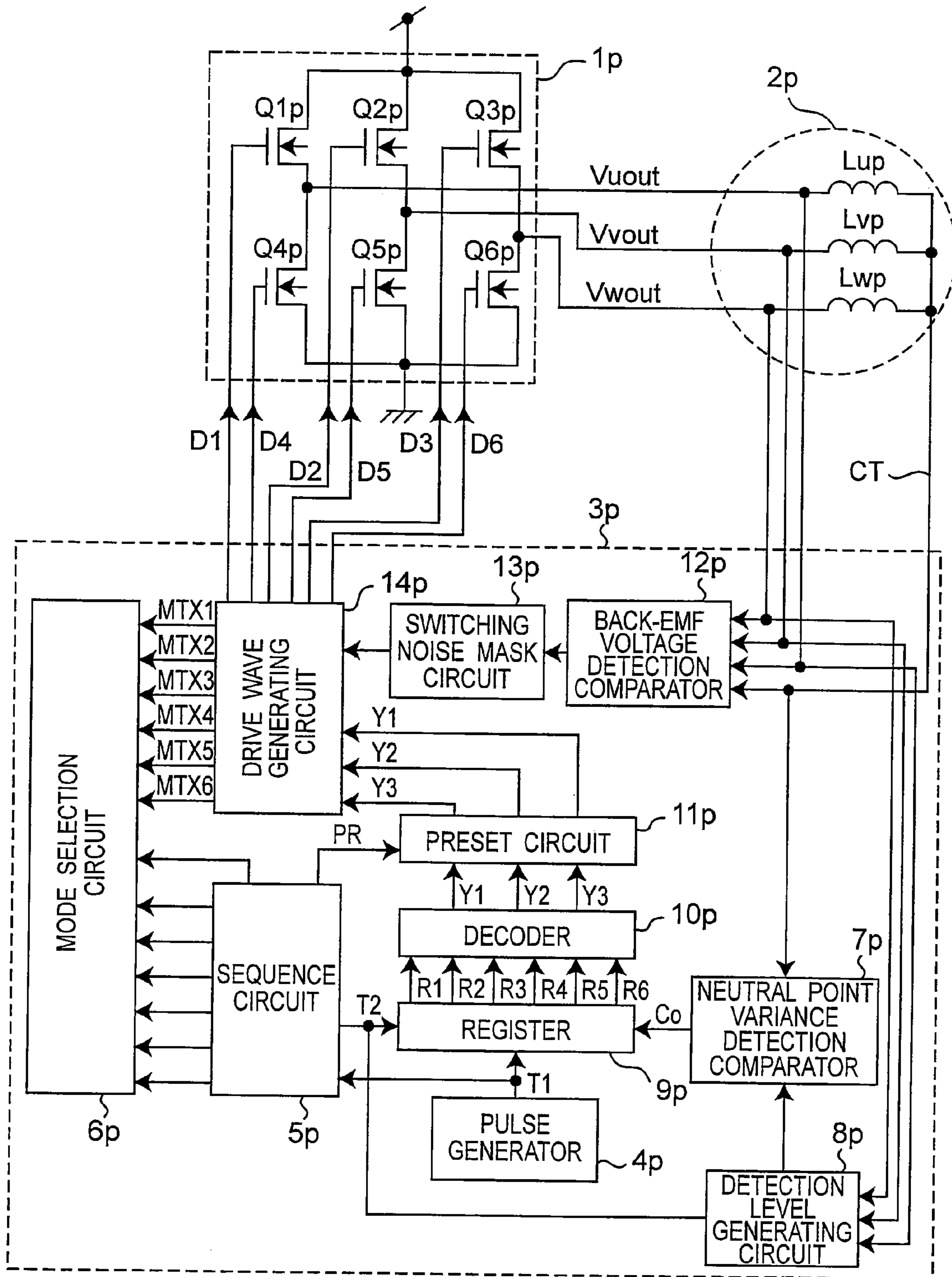
Fig.35 PRIOR ART
