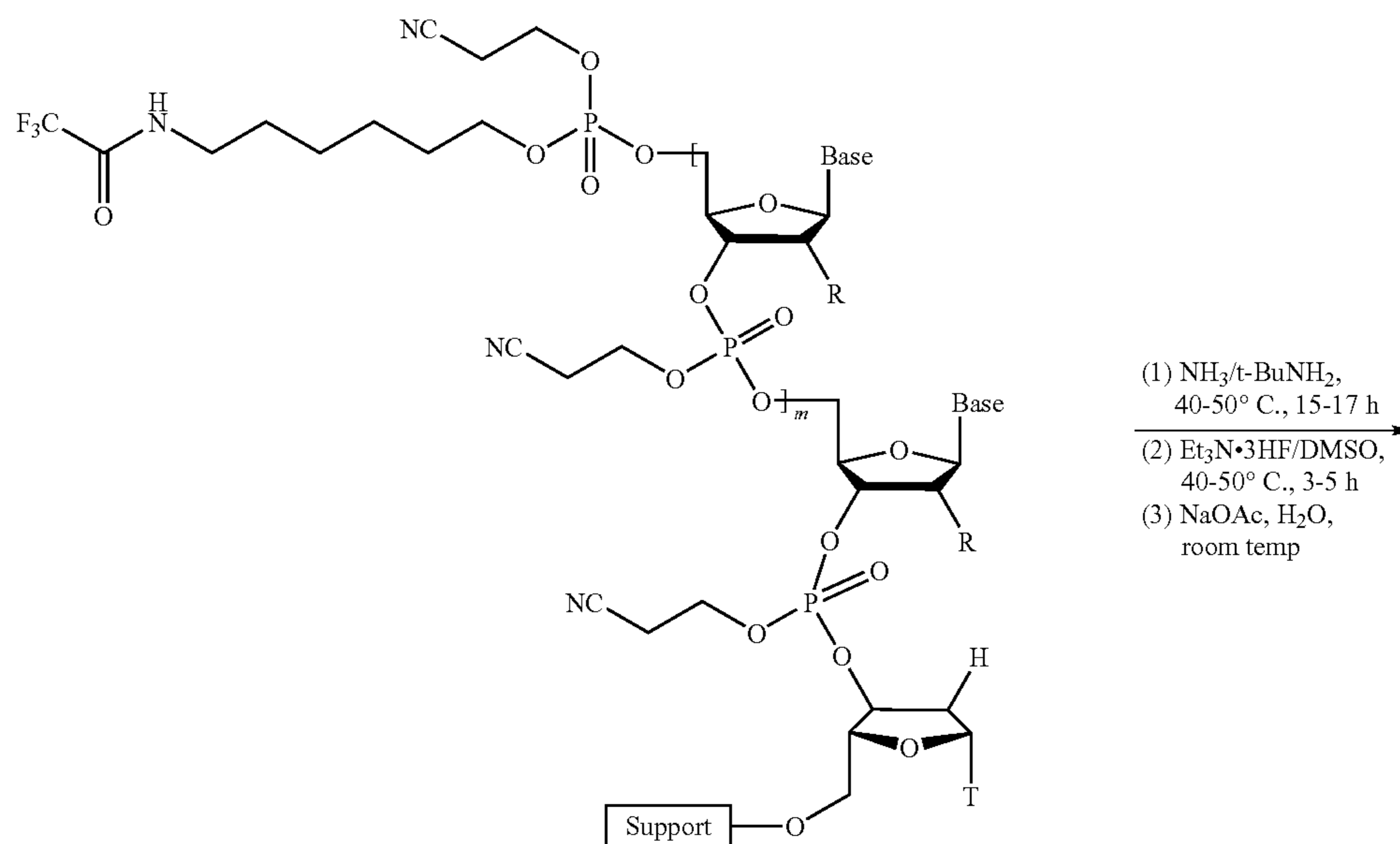
Scheme 1. (continued)
