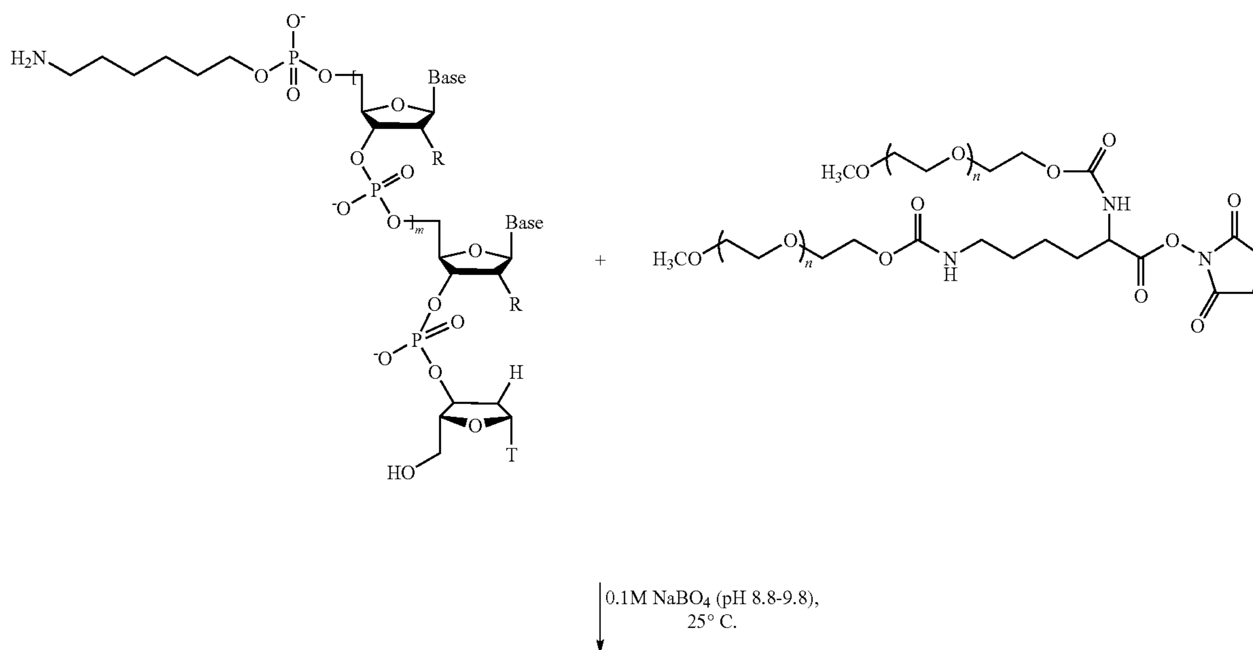
Scheme 2. PEGylation
