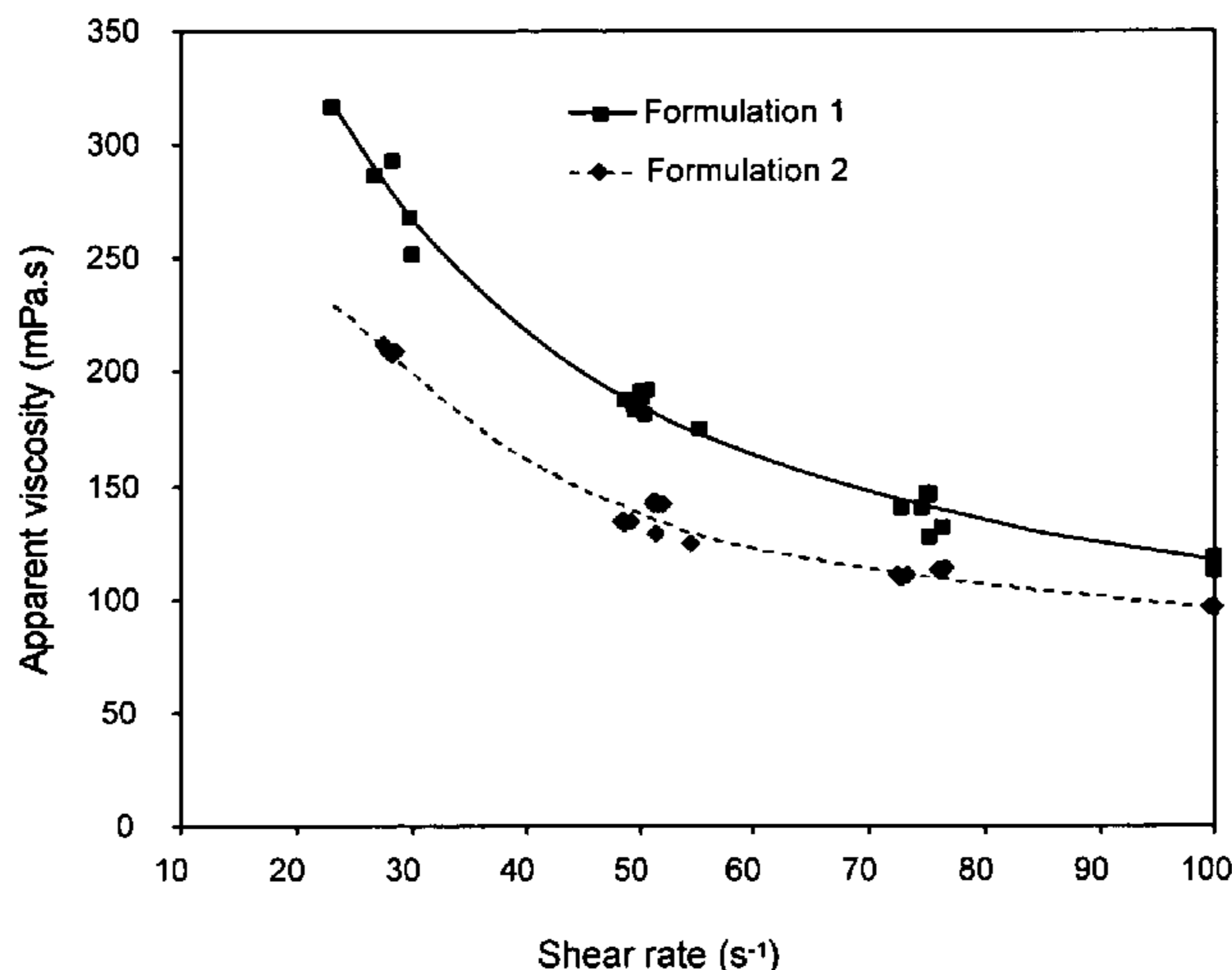
Viscosity vs Shear Rate for Diutan Strains
