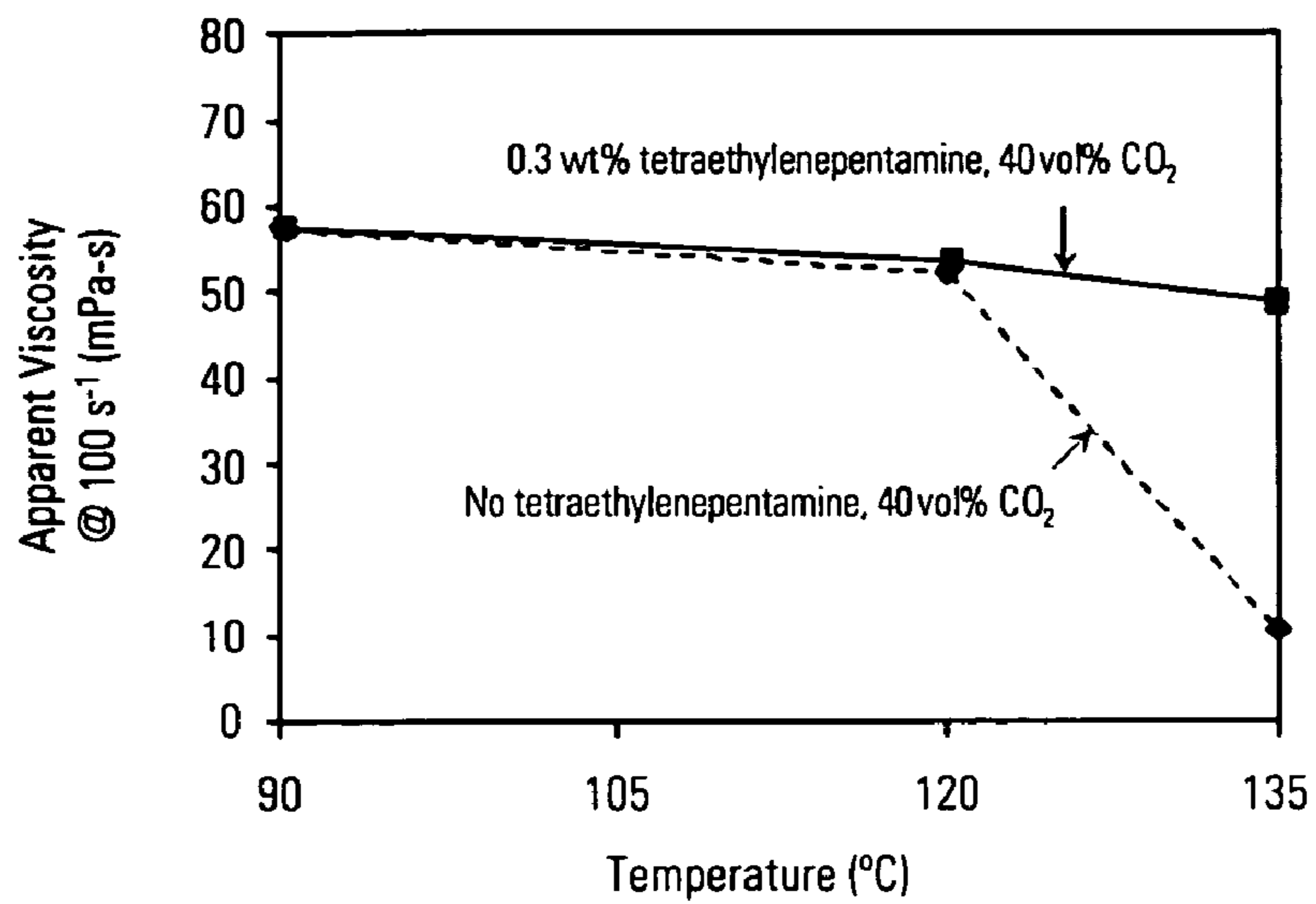
FIG. 3a Effect of tetraethylenamine on viscosity
