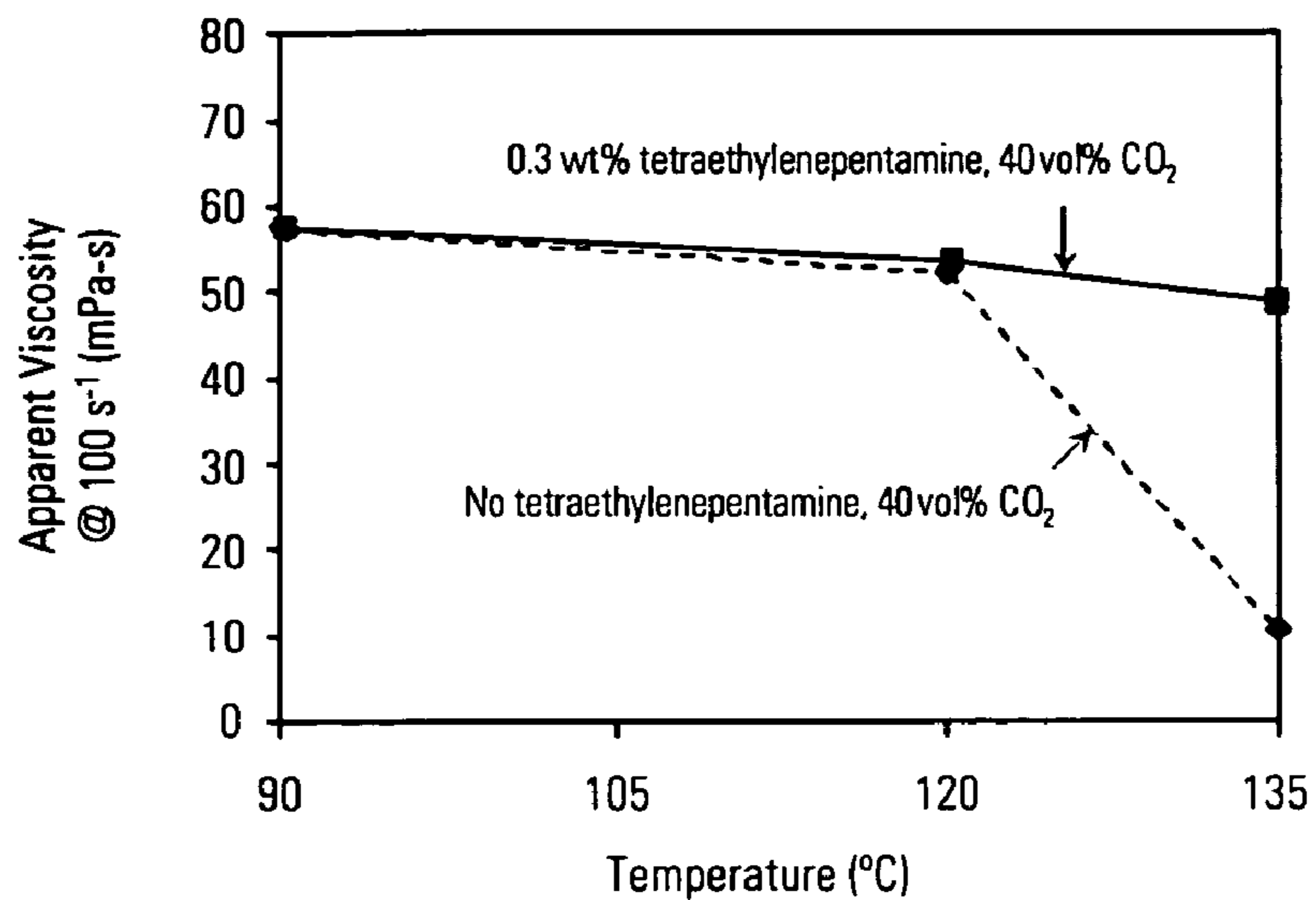
FIG. 3a Effect of tetraethylenamine on viscosity
