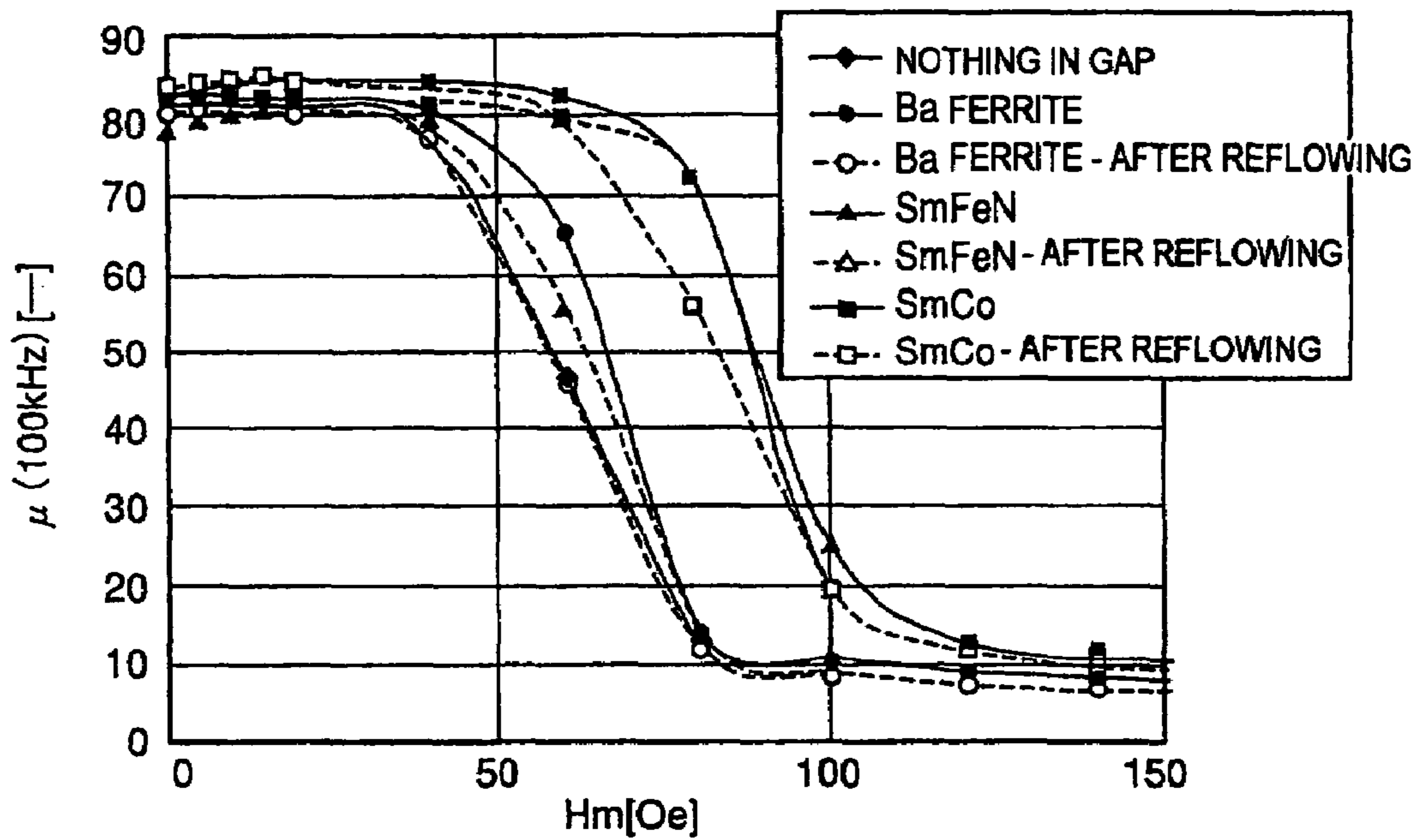
DC SUPERPOSED CHARACTERISTIC
