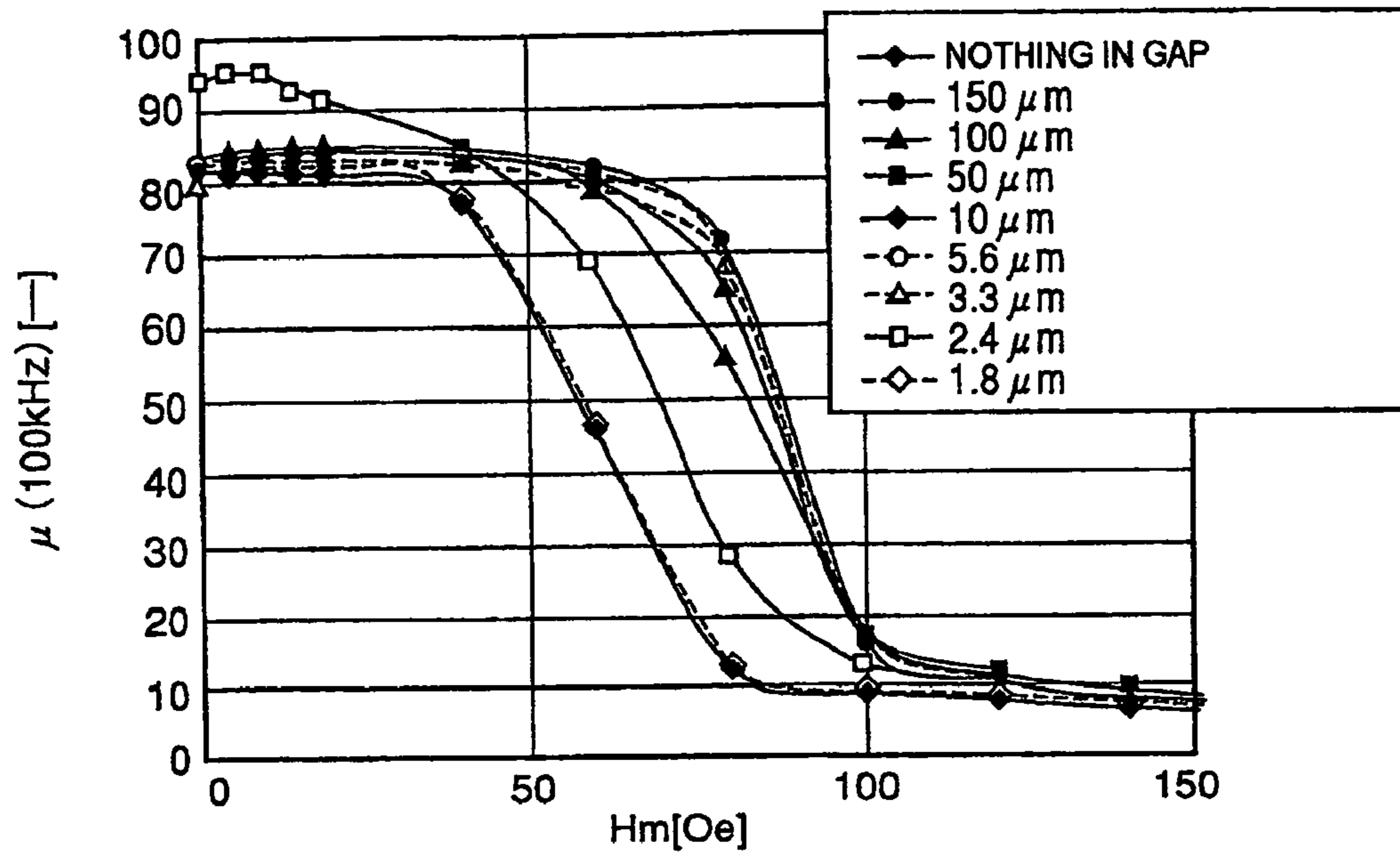
DC SUPERPOSED CHARACTERISTIC
