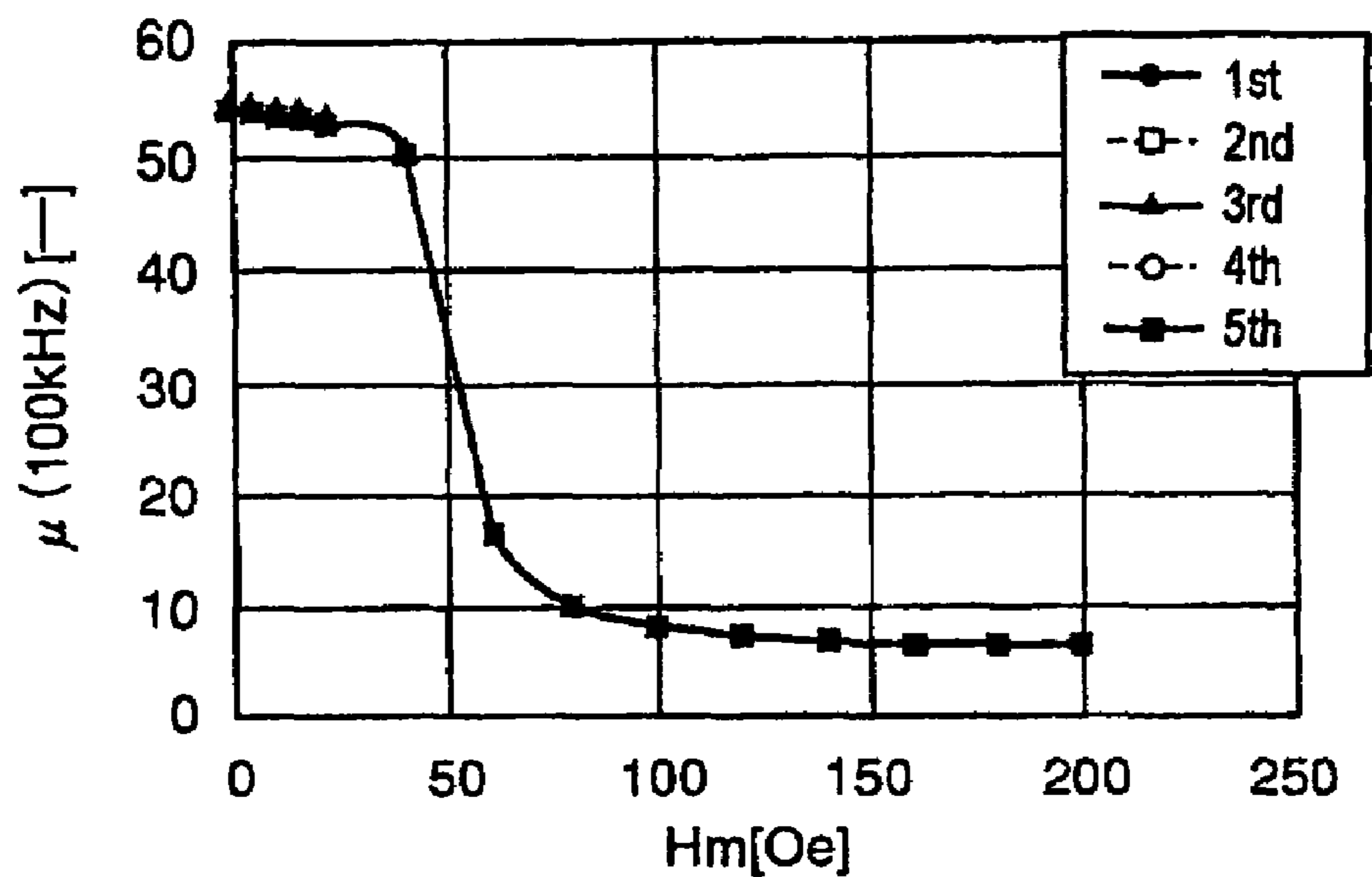
DC SUPERPOSED CHARACTERISTIC (GaP)
