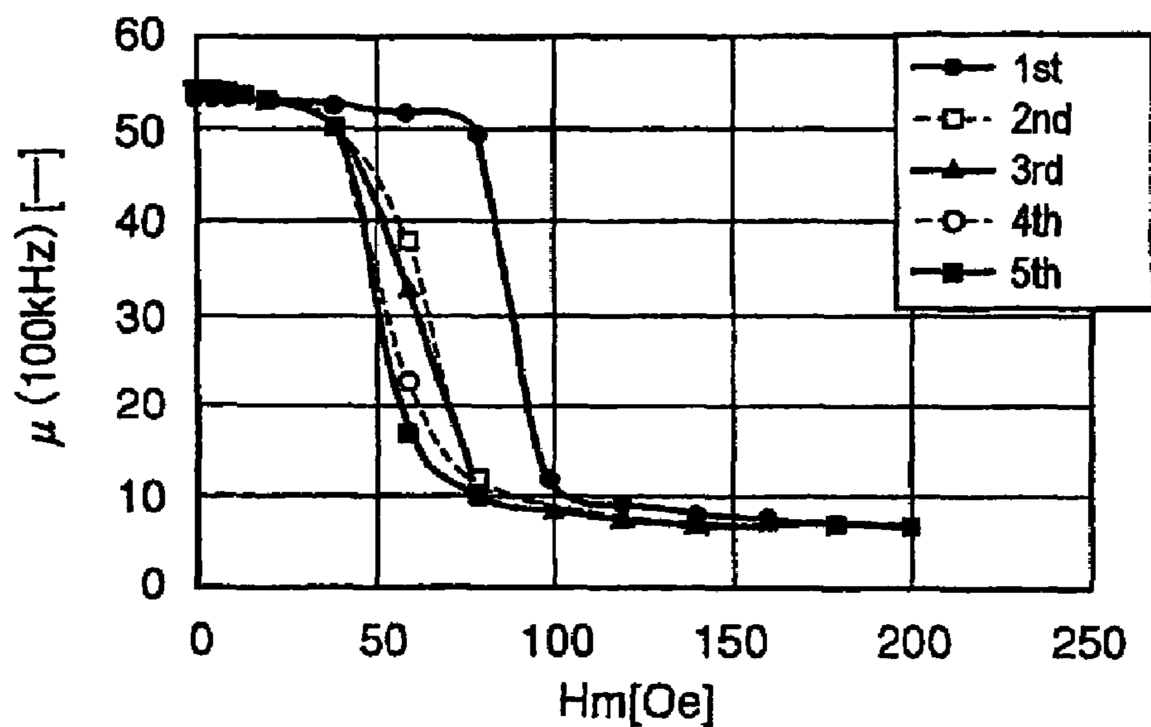
DC SUPERPOSED CHARACTERISTIC (Hc:4.0kOe)
