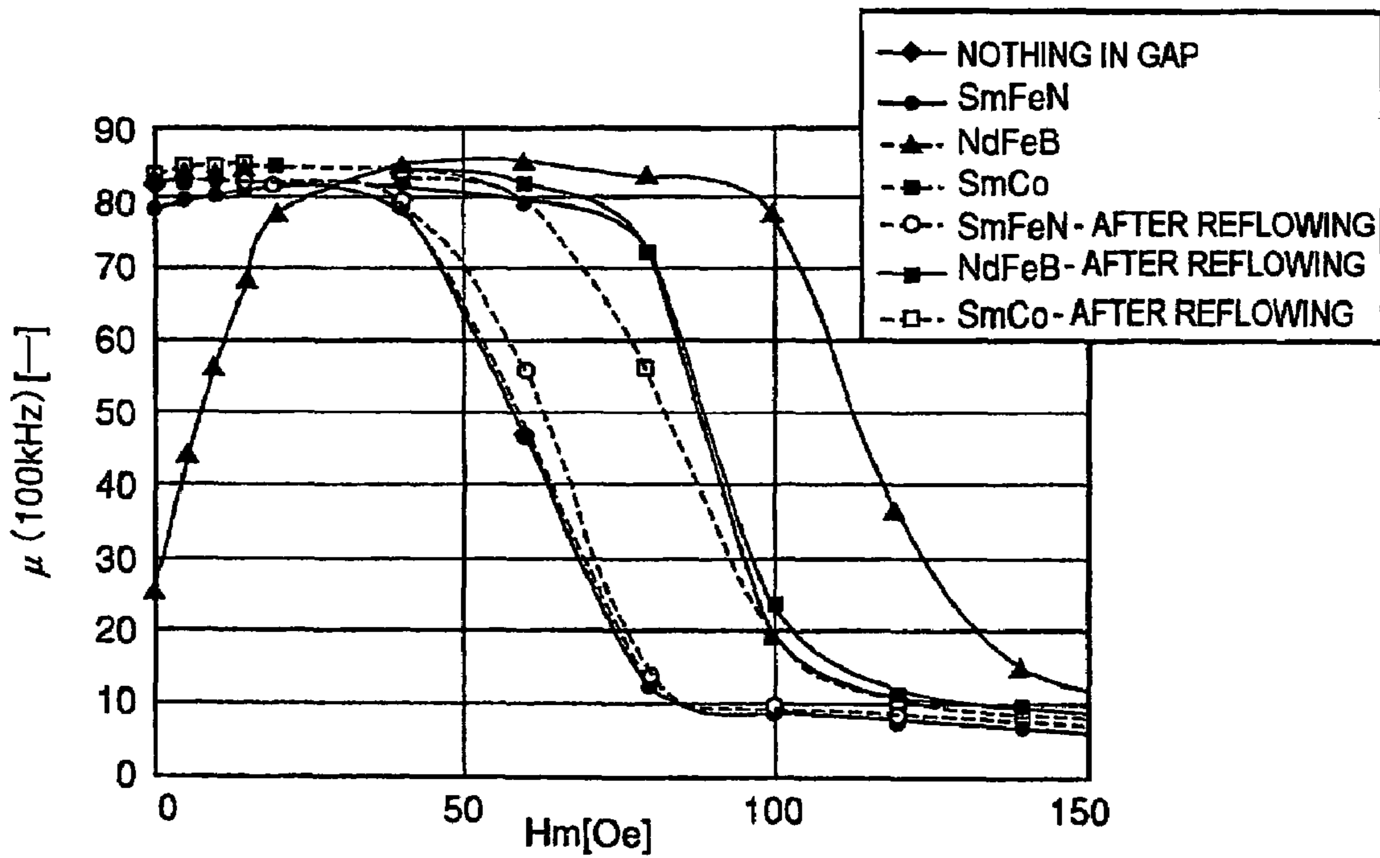
DC SUPERPOSED CHARACTERISTIC
