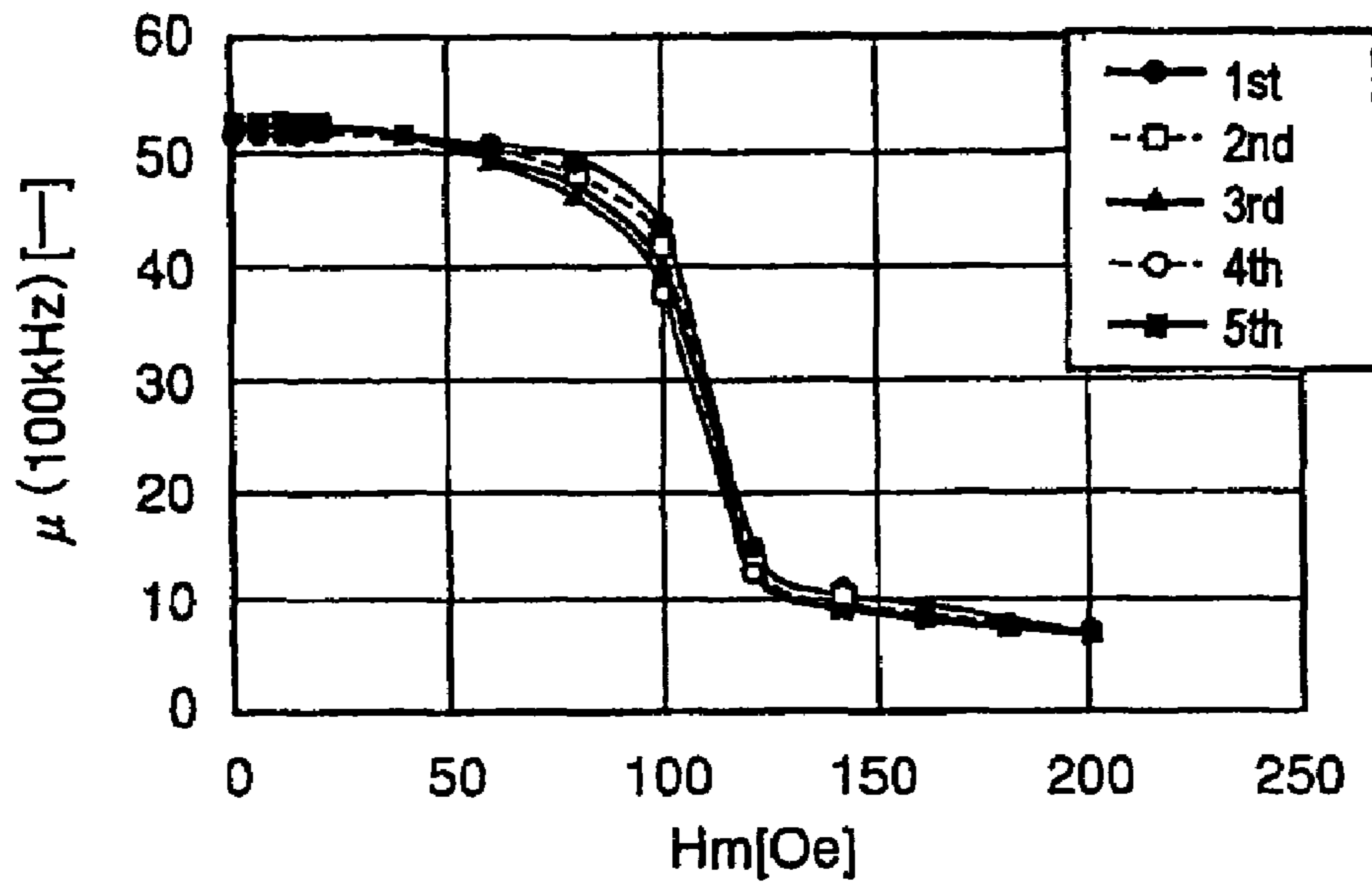
DC SUPERPOSED CHARACTERISTIC ( H_c:5.0\text{kOe} )
