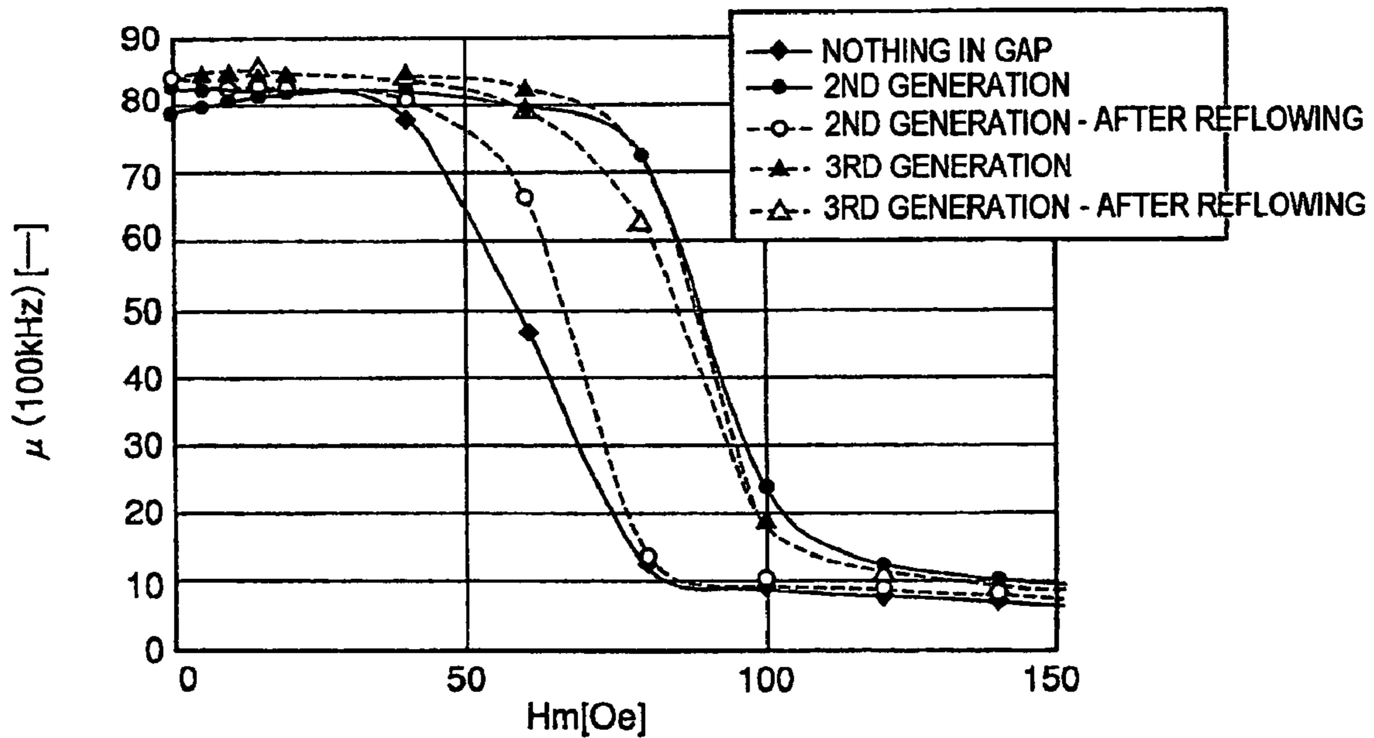
DC SUPERPOSED CHARACTERISTIC
