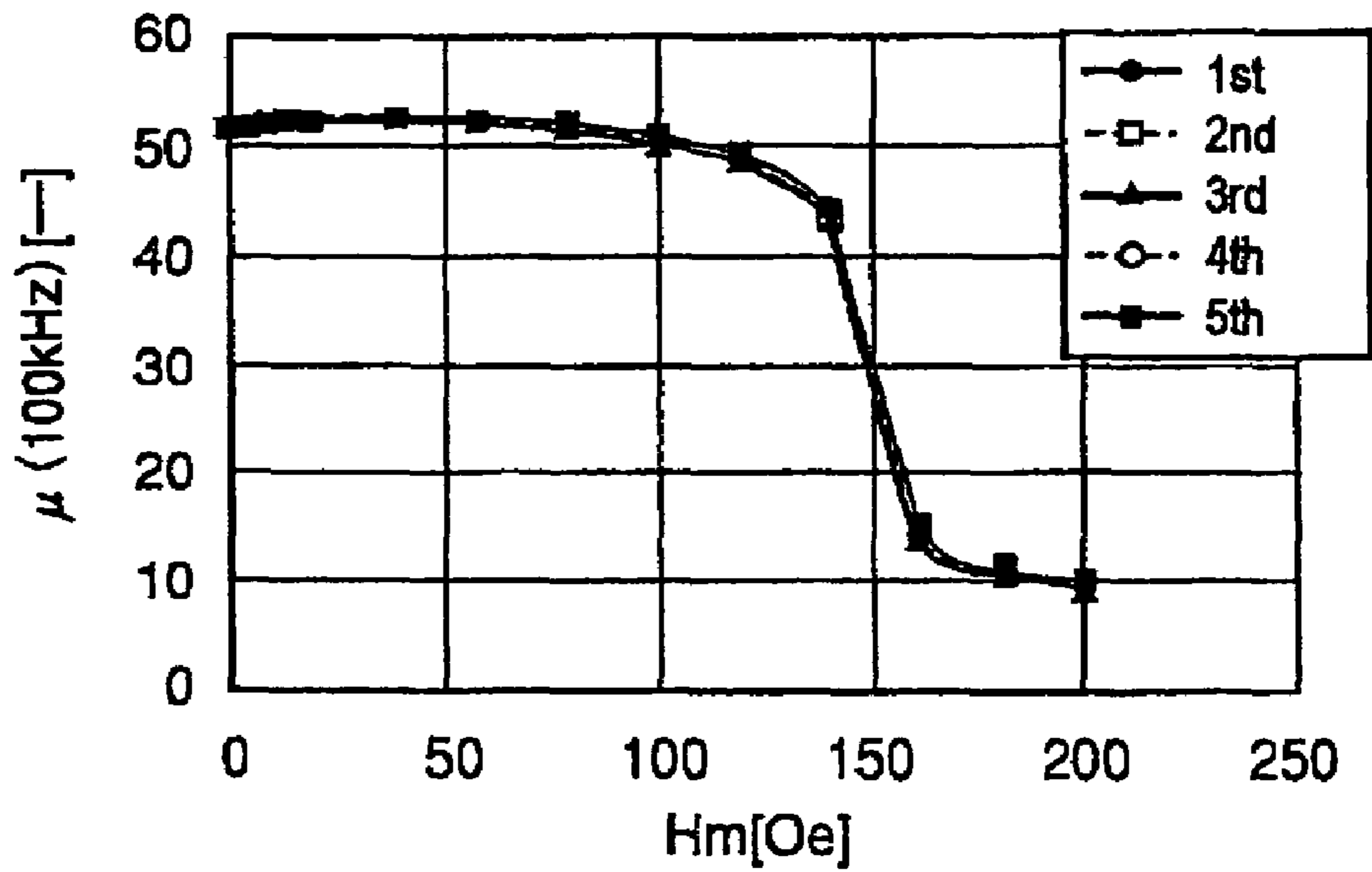
DC SUPERPOSED CHARACTERISTIC ( H_c:10\text{kOe} )
