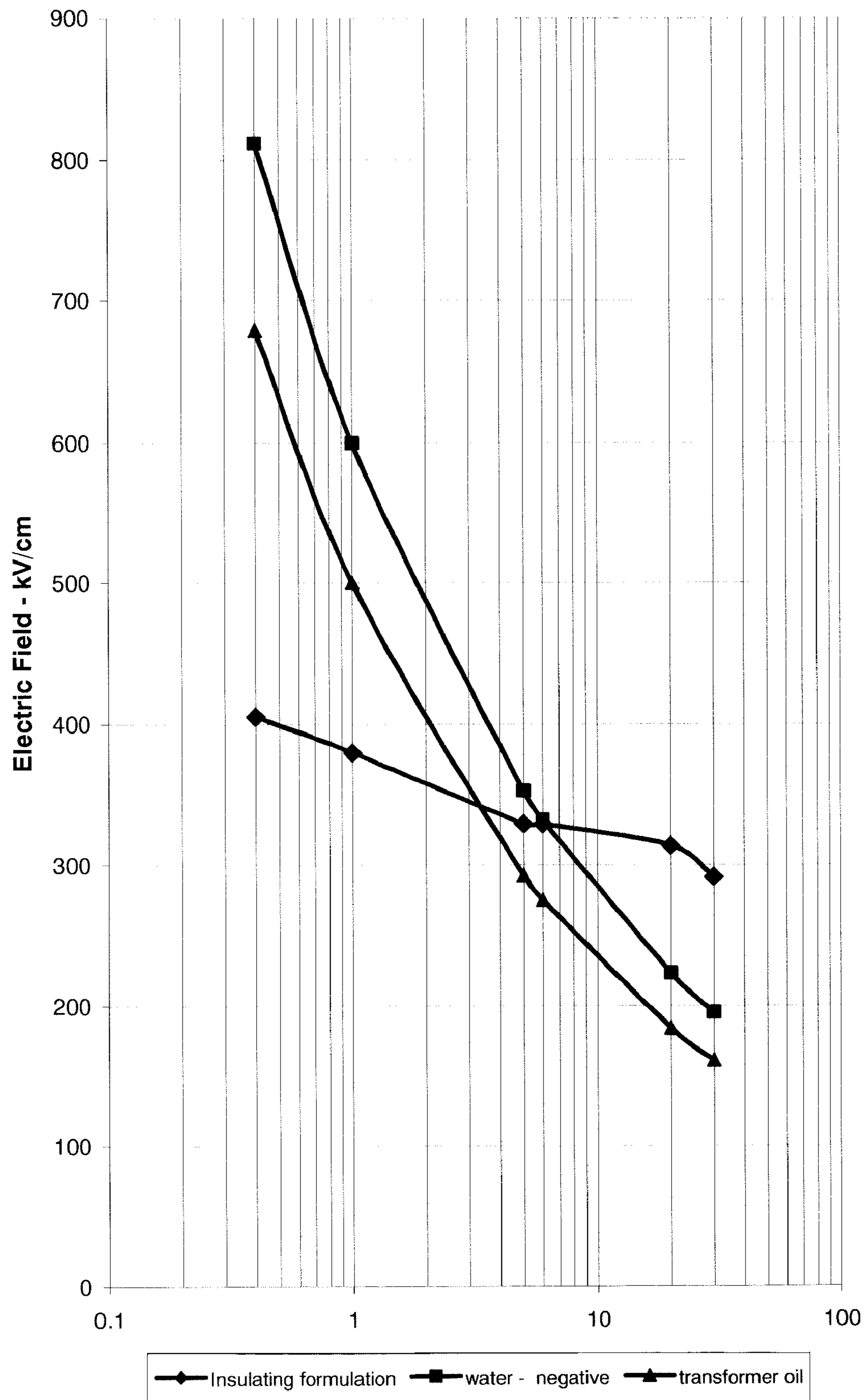
Dielectric Strength vs. Delay To Breakdown Figure 32
