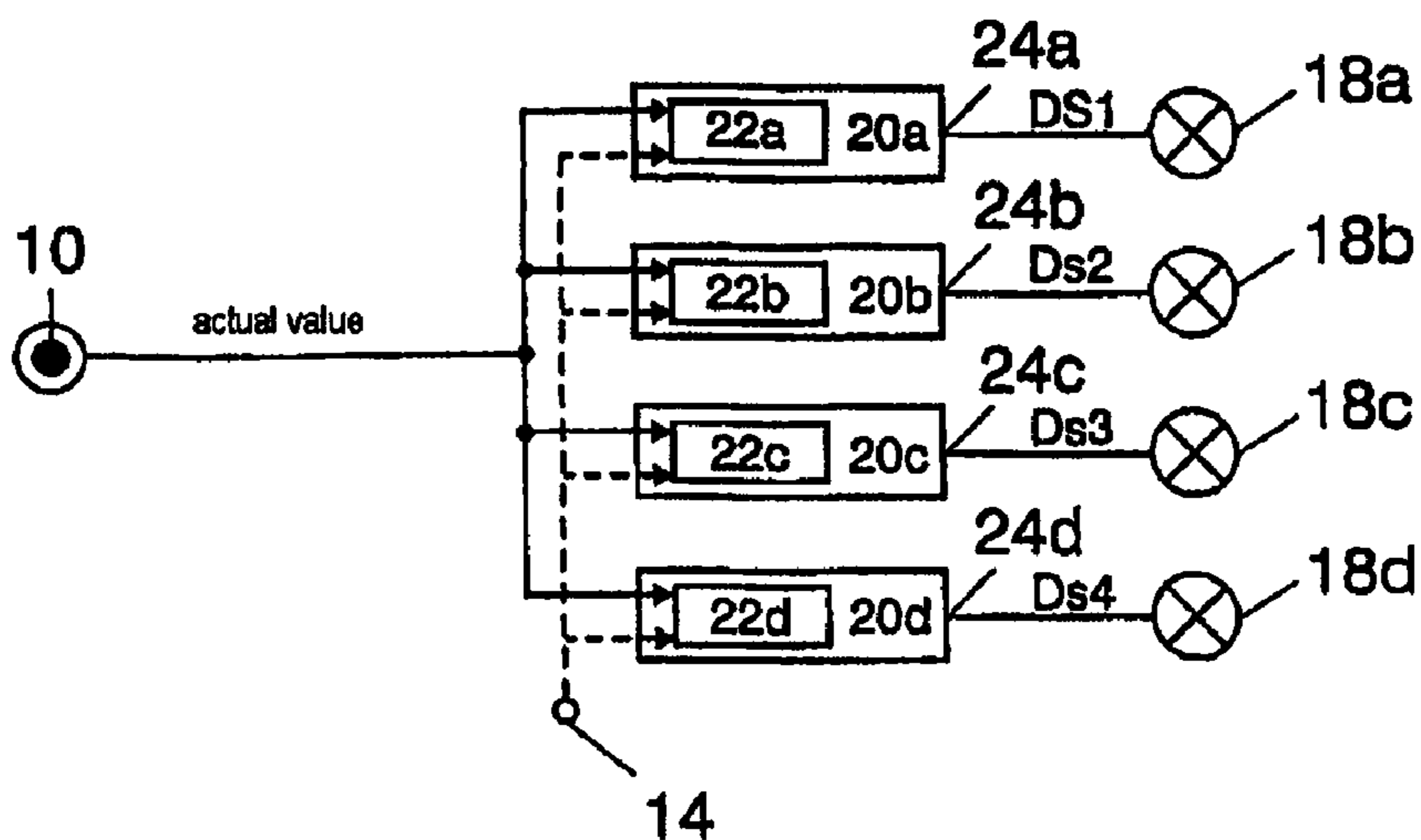
FIG 3 PRIOR ART
