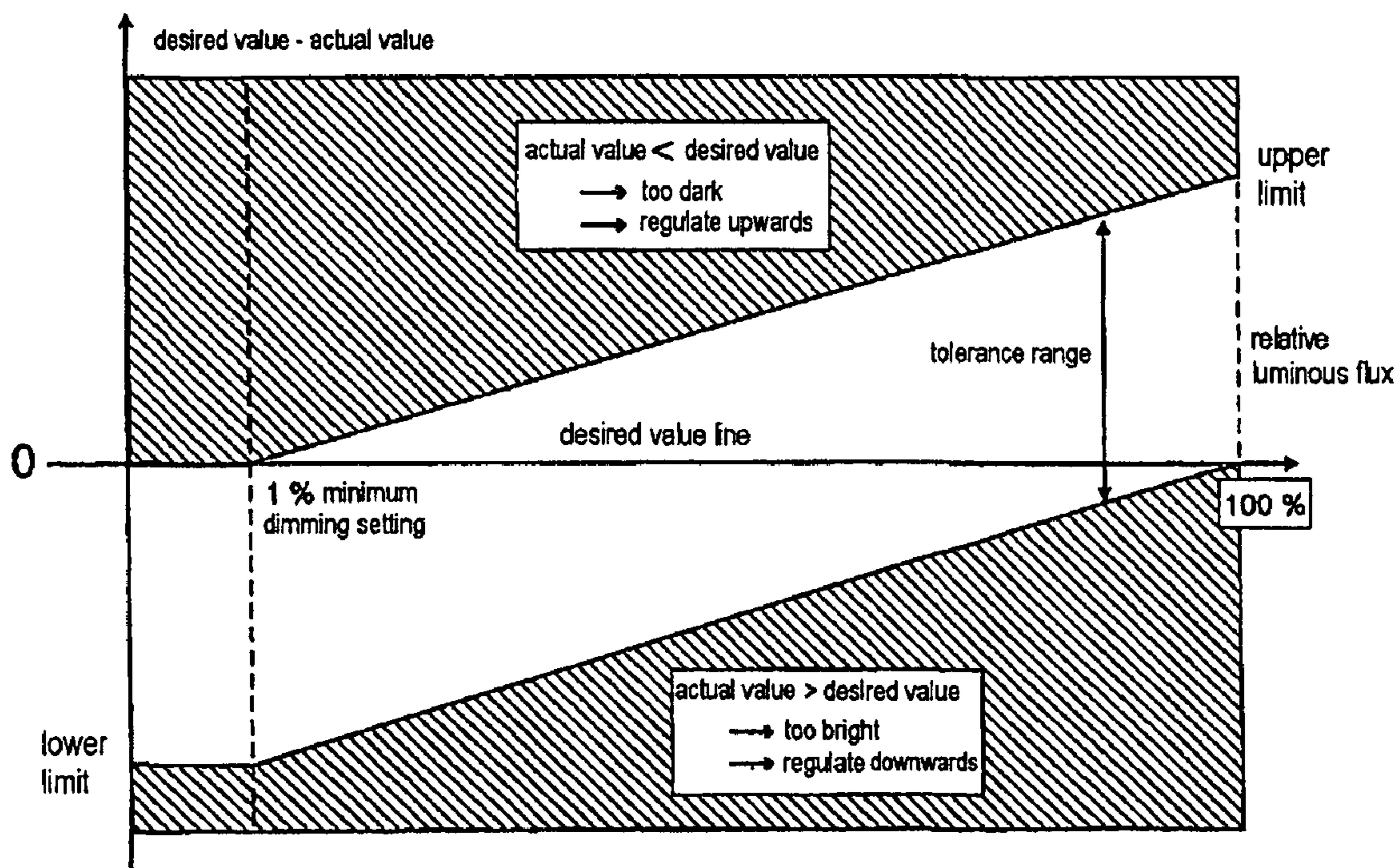
FIG 4 PRIOR ART
