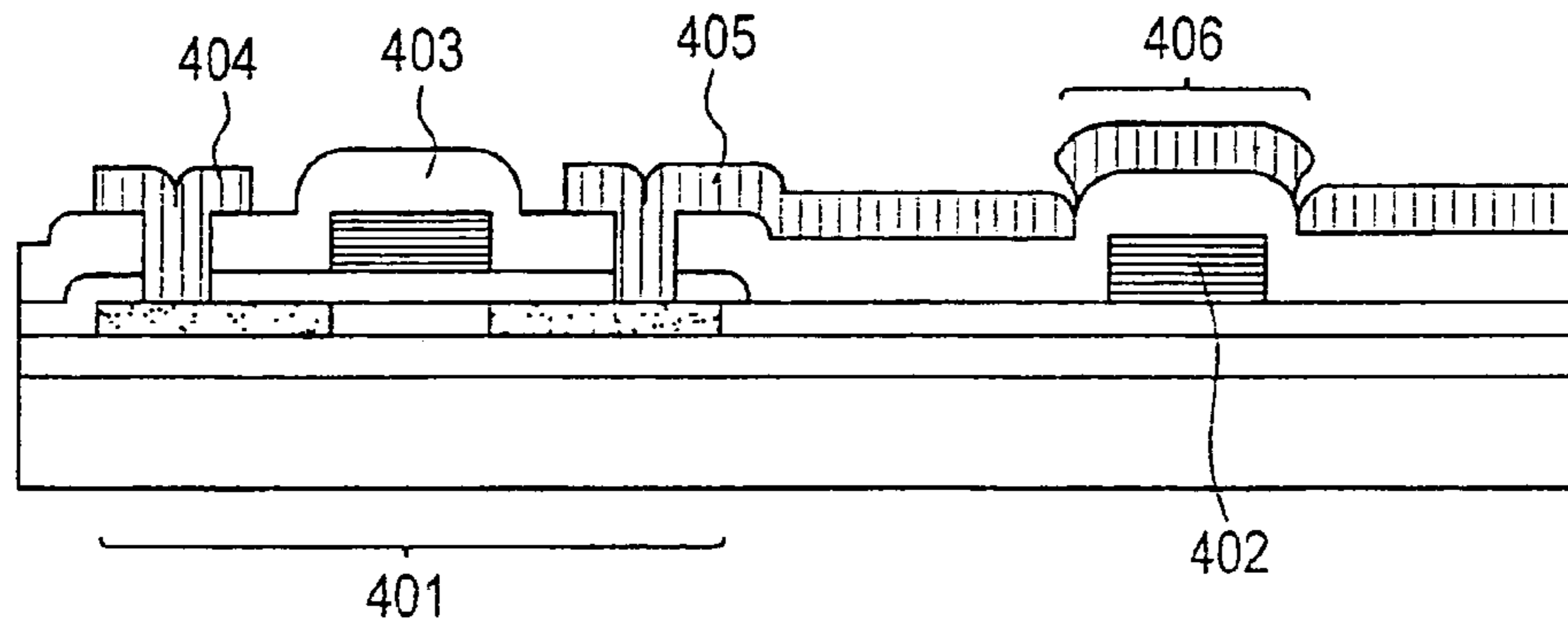
FIG.4 PRIOR ART
