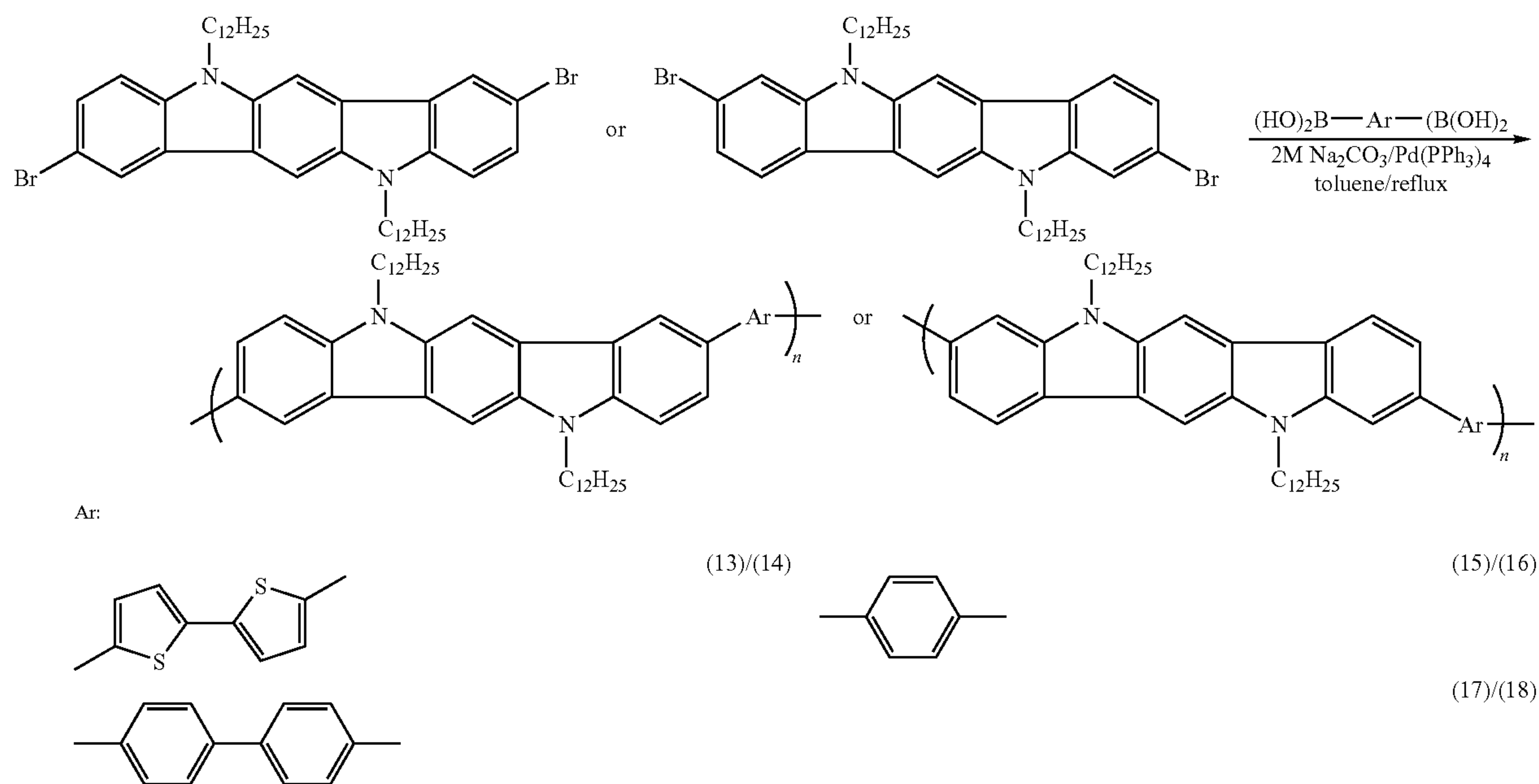
Scheme 2. Synthesis of polymer (13) through (18).
