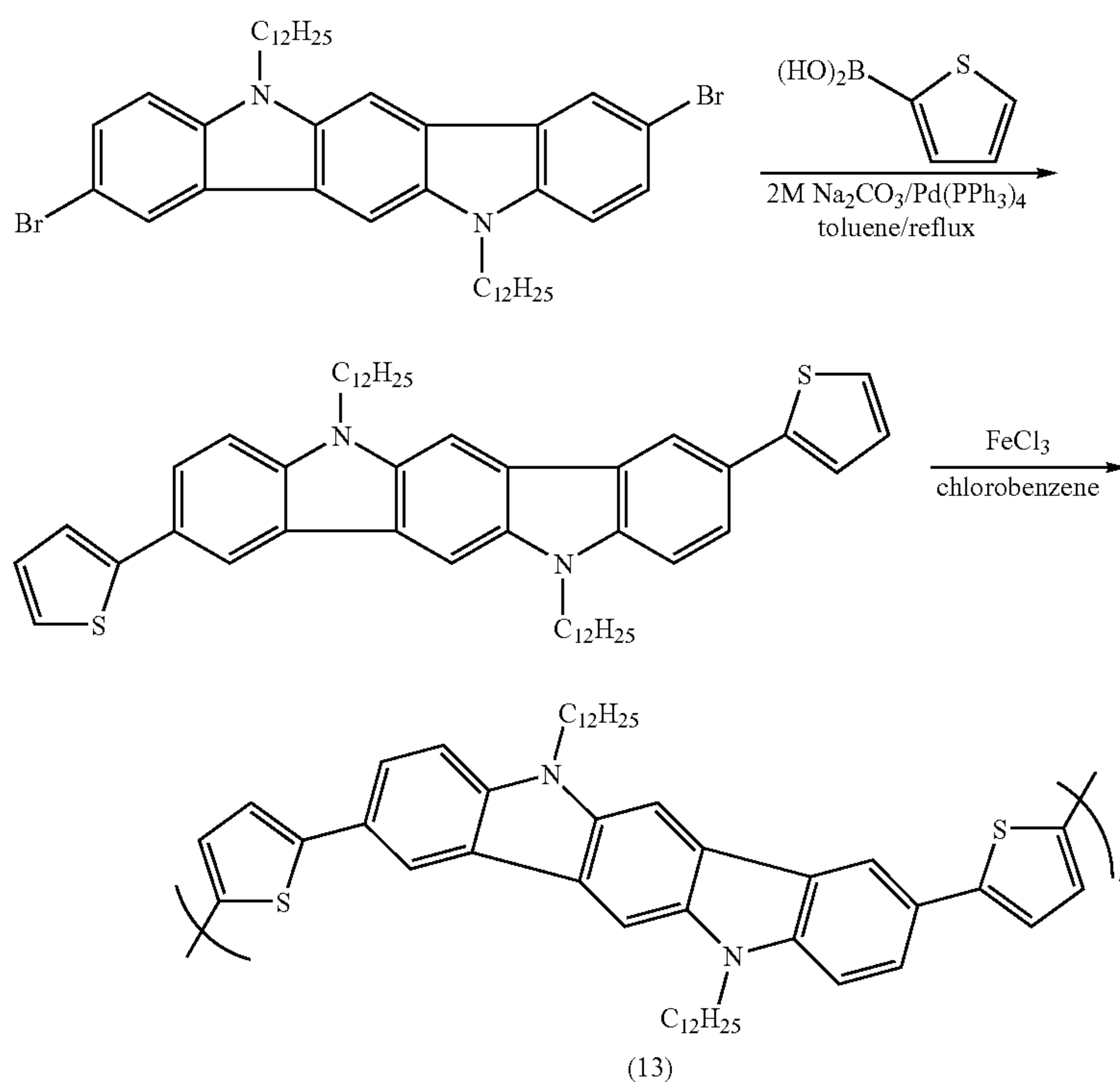
Scheme 3. Synthesis of polymer (13).
