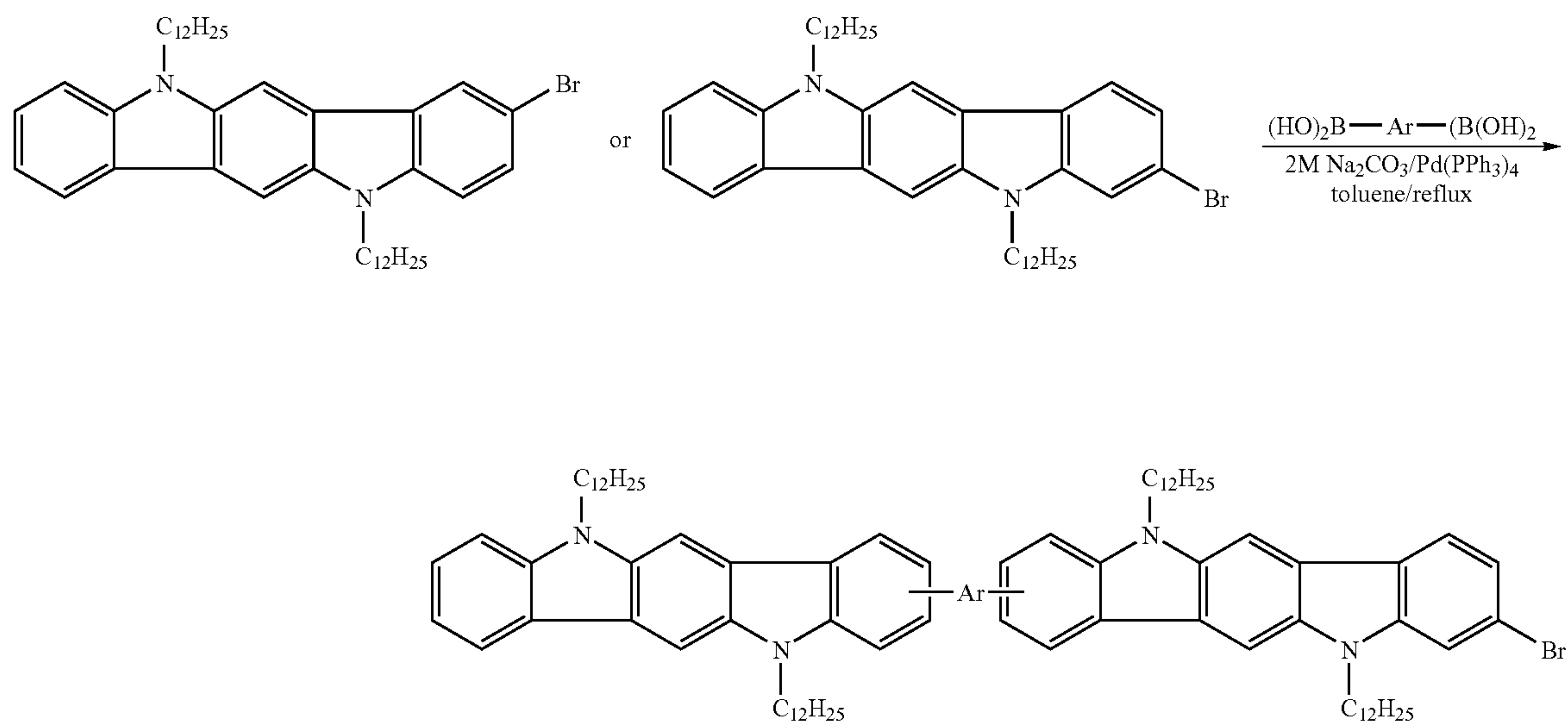
Scheme 1. Synthesis of Compound (1), (2), and (9) through (12).
