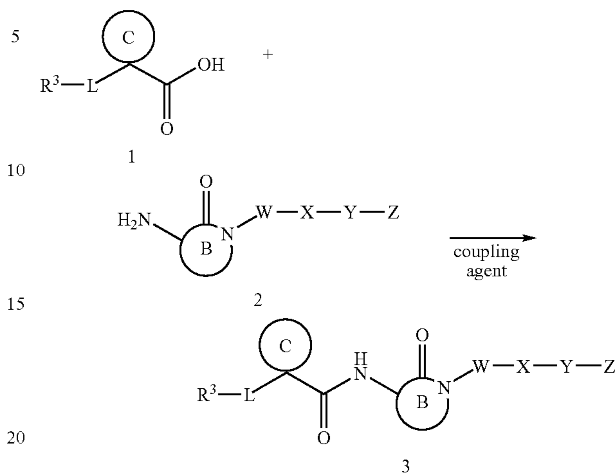
Scheme 1
