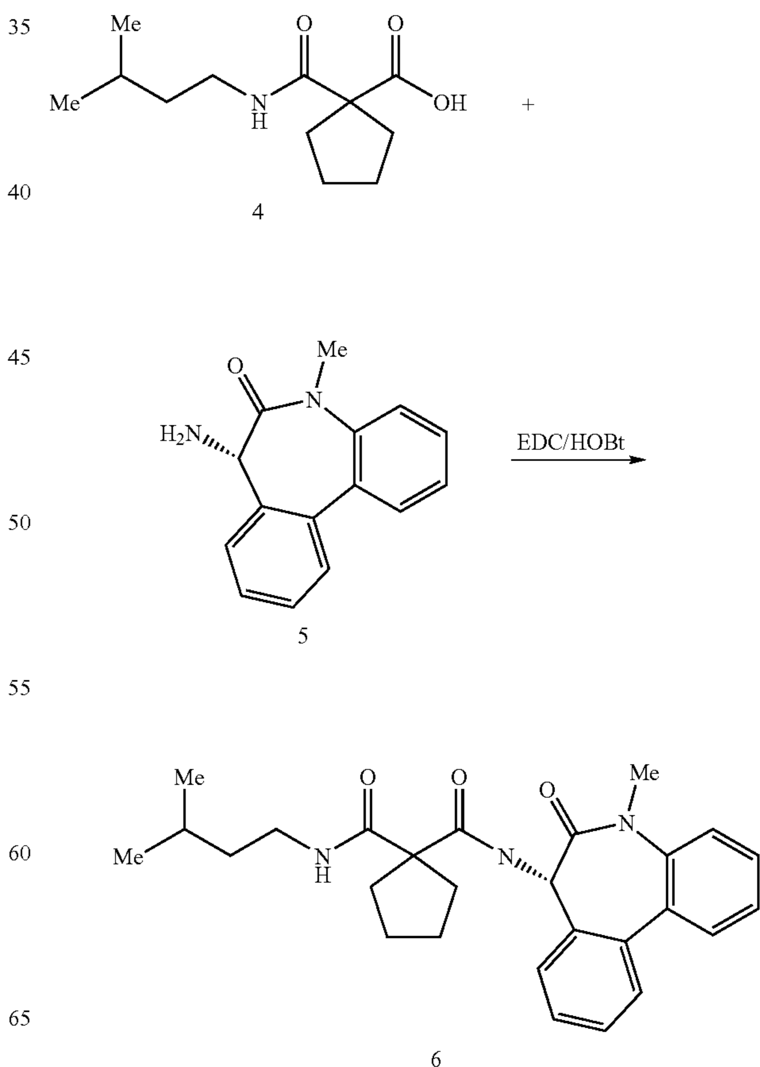
Scheme 2
