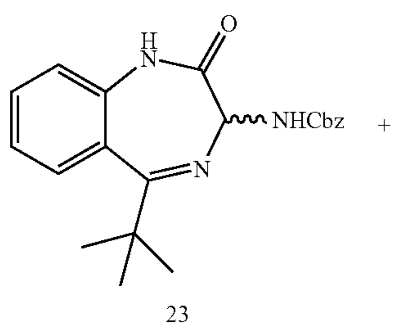
Scheme 7
