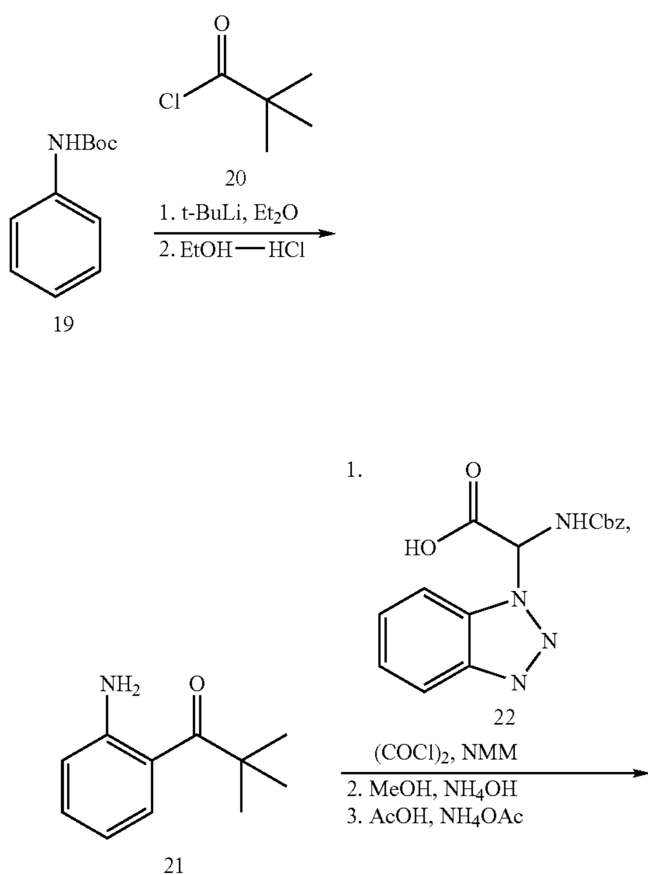
Scheme 6
