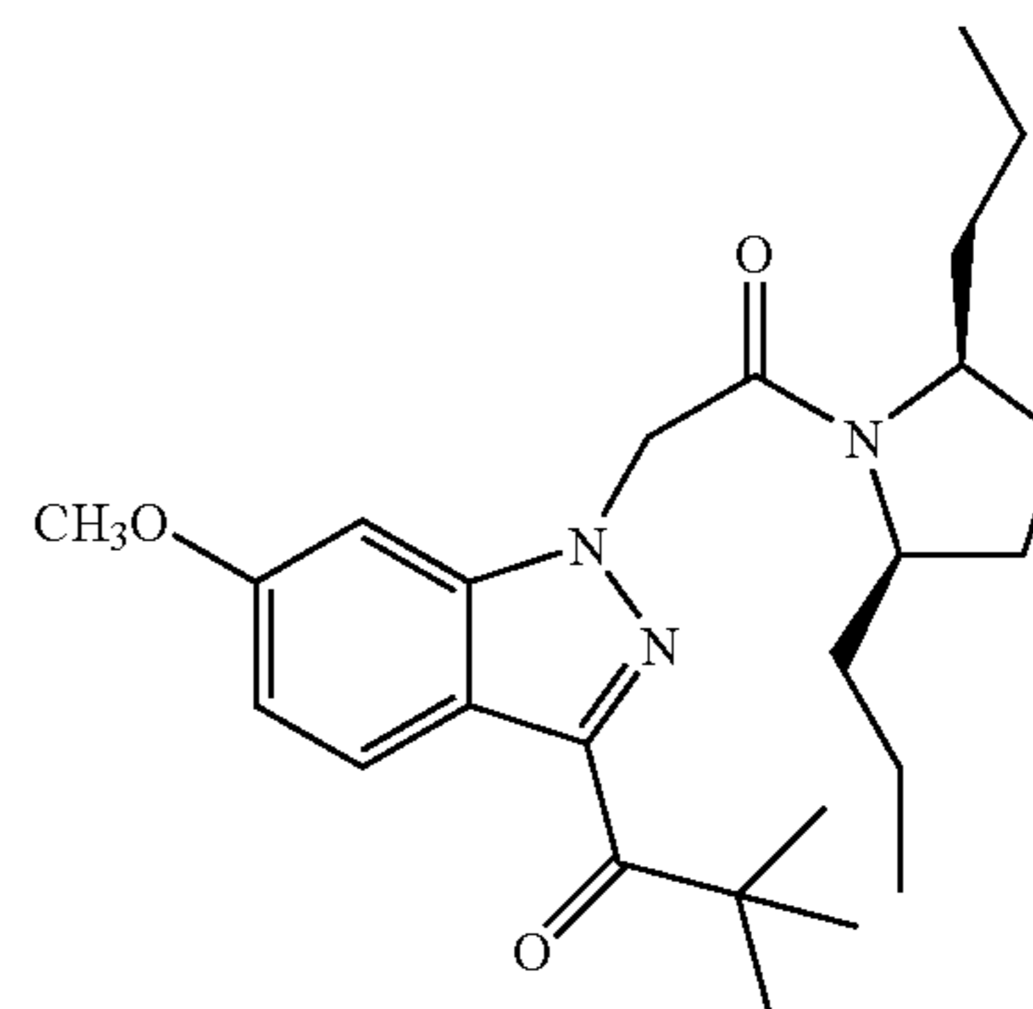
1-(1-{2-[Cis-2,5-dipropylpyrrolidin-1-yl]-2-oxoethyl}-6-methoxy-1H-indazol-3-yl)-2,2-dimethylpropan-1-one
