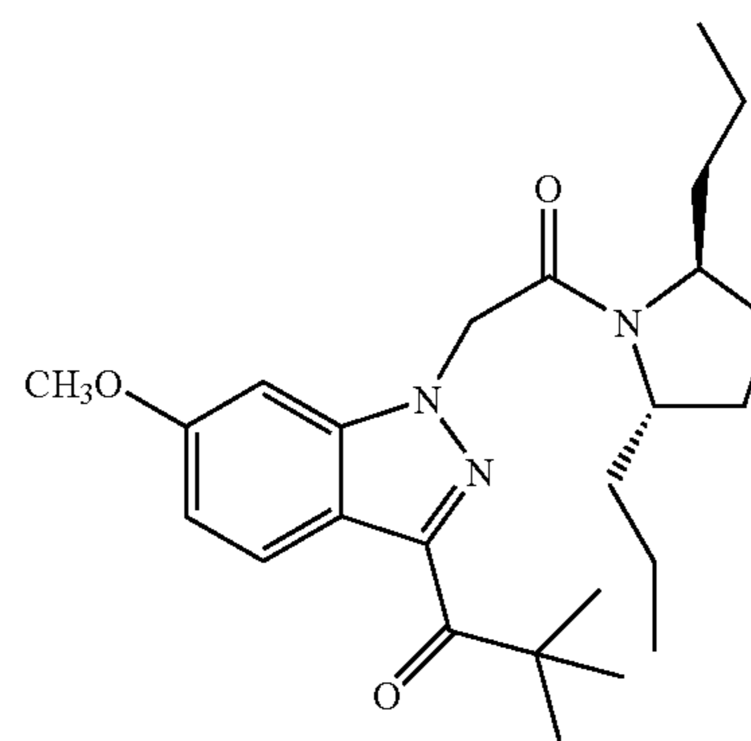
1-(1-{2-[Trans-2,5-dipropylpyrrolidin-1-yl]-2-oxoethyl}-6-methoxy-1H-indazol-3-yl)-2,2-dimethylpropan-1-one
