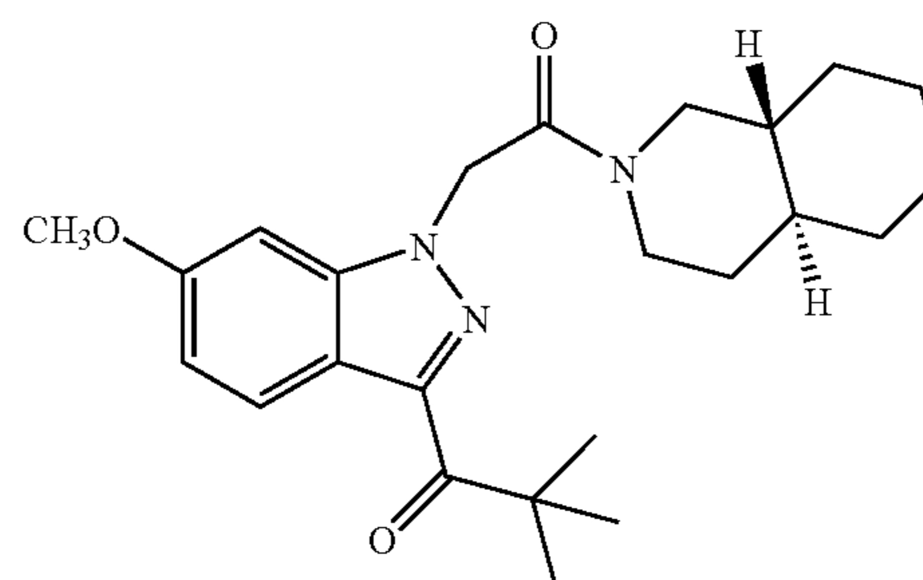
1-(6-methoxy-1-{2-[trans-octahydroisoquinolin-2(1H)-yl]-2-oxoethyl}-1H-indazol-3-yl)-2,2-dimethylpropan-1-one
