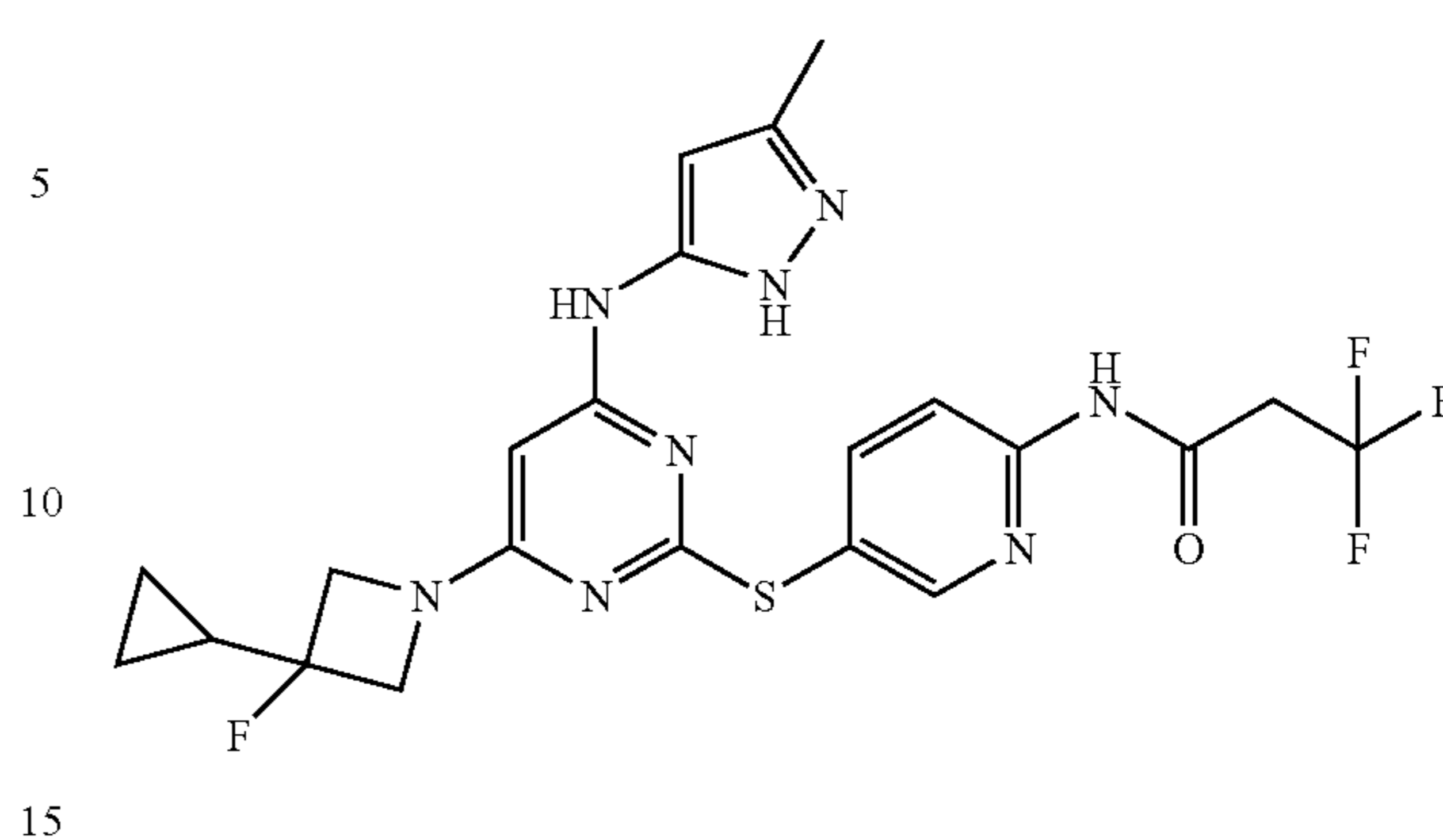
N-(5-(4-(3-methyl-1H-pyrazol-5-ylamino)-6-(3-cyclopropyl-3-fluoroazetidin-1-yl)pyrimidin-2-ylthio)pyridin-2-yl)-3,3,3-trifluoropropanamide (I-21)
