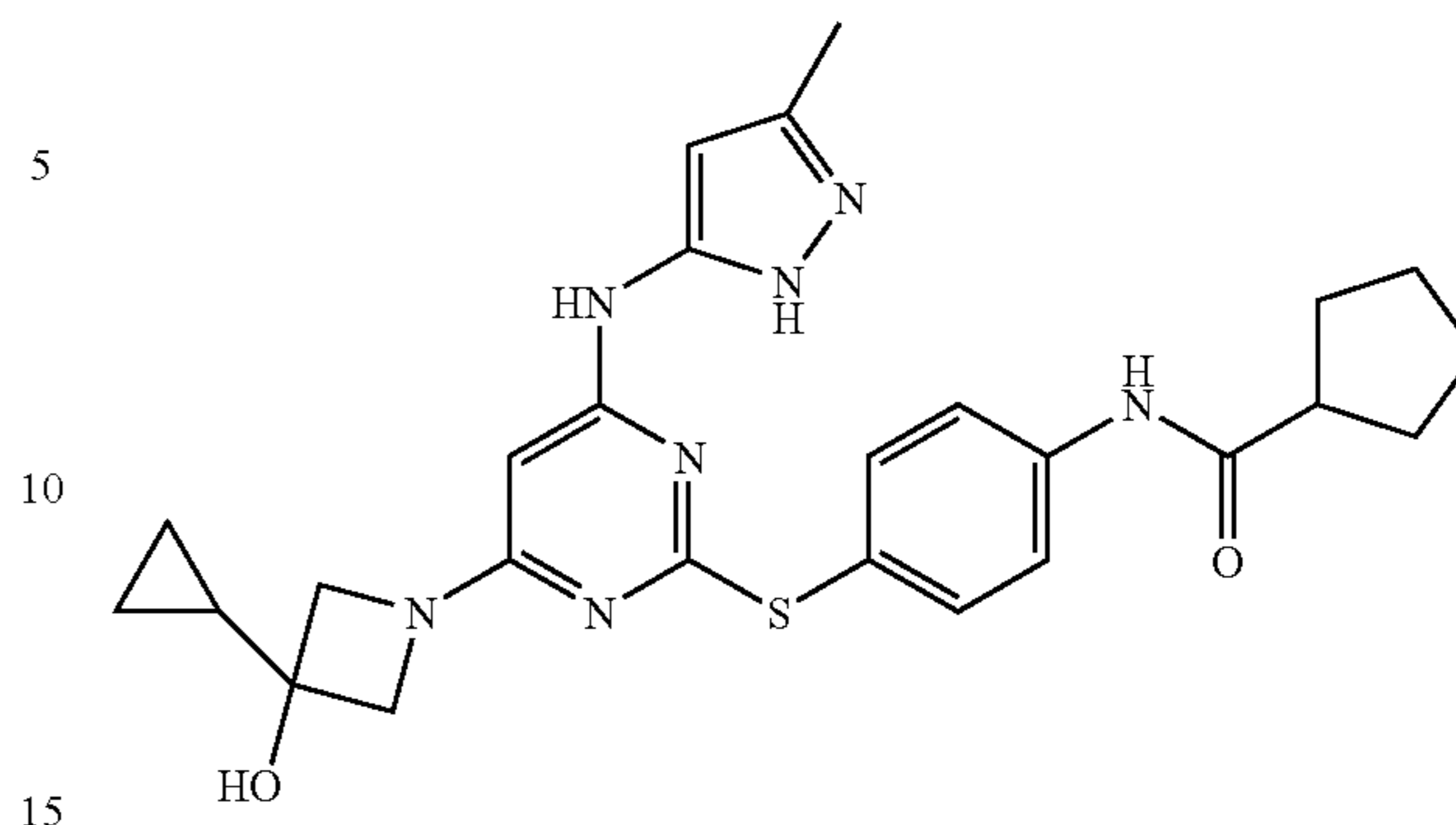
N-(4-((4-(3-methyl-1H-pyrazol-5-ylamino)-6-(3-cyclopropyl-3-hydroxyazetididin-1-yl)pyrimidin-2-yl)sulfanyl)phenyl)cyclopentanecarboxamide (I-9)
