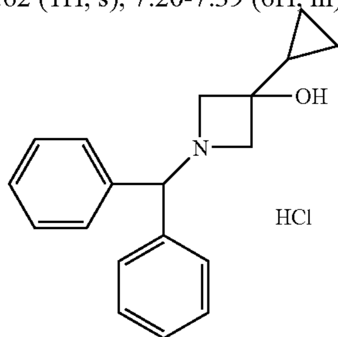
1-Benzhydryl-3-cyclopropylazetididin-3-ol hydrochloride
