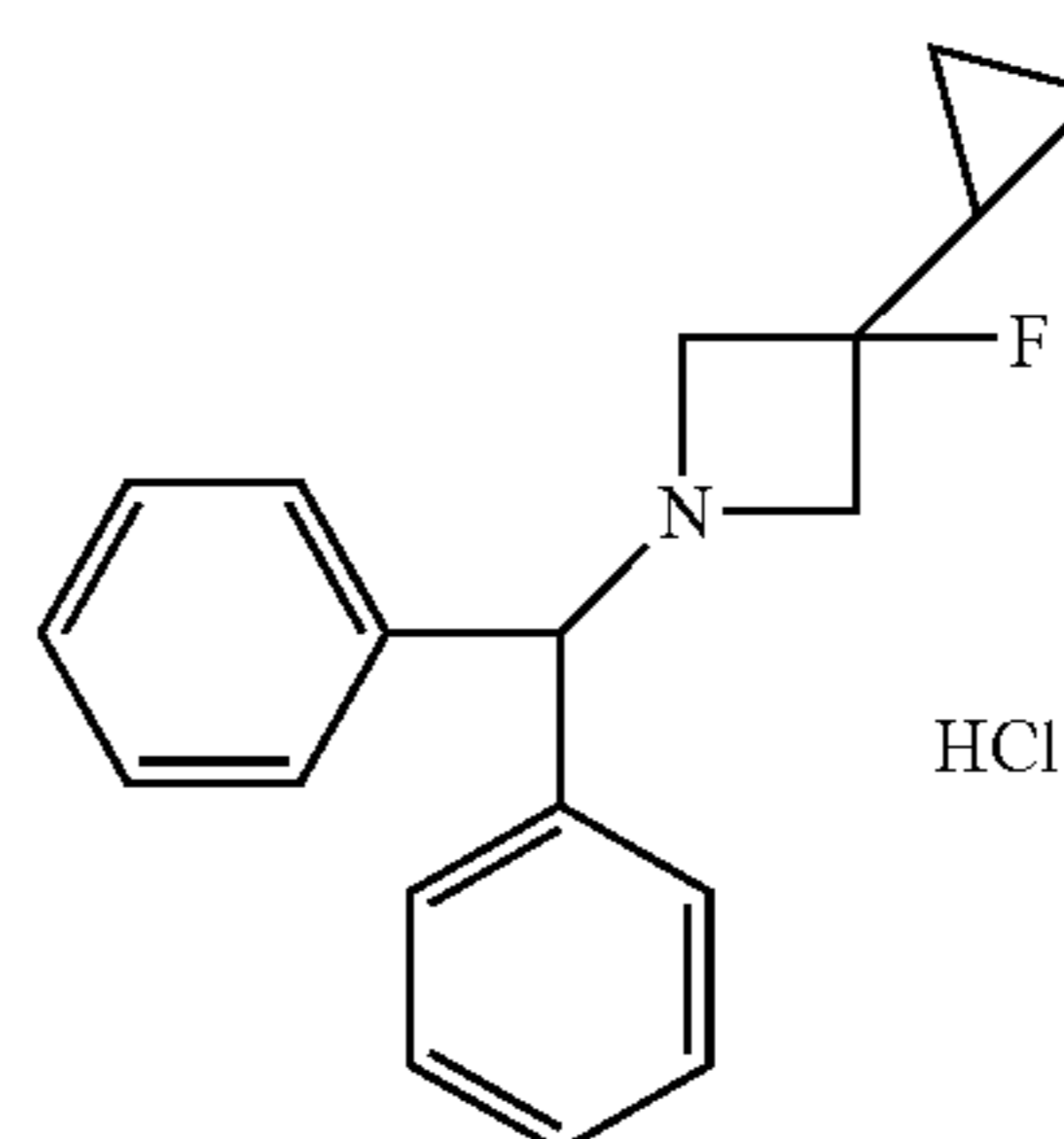
1-Benzhydryl-3-cyclopropyl-3-fluoroazetididine hydrochloride
