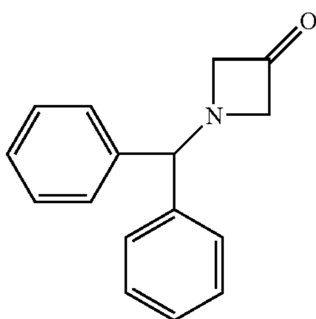
N-Benzhydrylazetididin-3-one
