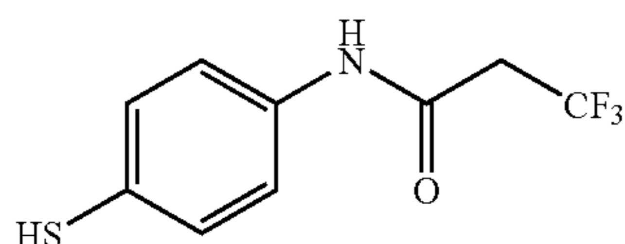
3,3,3-trifluoro-N-(4-mercaptophenyl)propanamide
