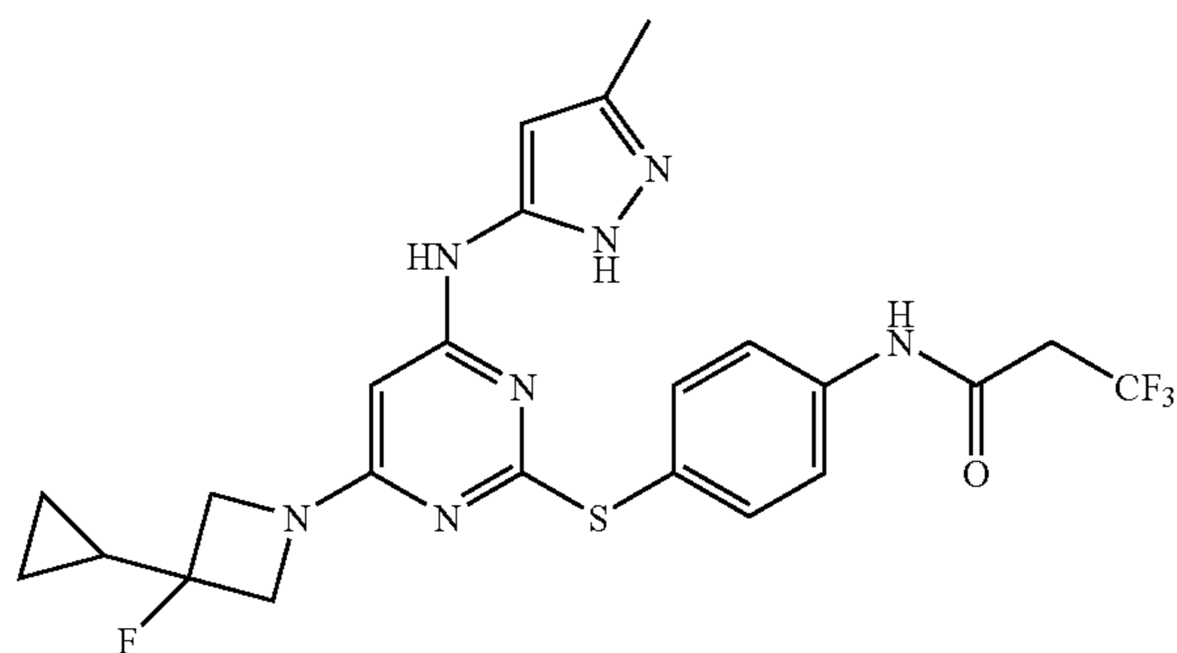
N-(4-(4-(3-methyl-1H-pyrazol-5-ylamino)-6-(3-cyclopropyl-3-fluoroazetidin-1-yl)pyrimidin-2-ylthio)phenyl)-3,3,3-trifluoropropanamide (Compound I-14)
