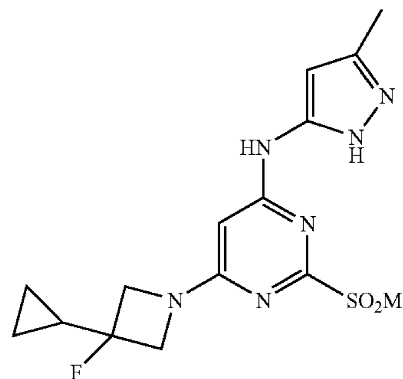
6-(3-cyclopropyl-3-fluoroazetidin-1-yl)-N-(3-methyl-1H-pyrazol-5-yl)-2-(methylsulfonyl)pyrimidin-4-amine
