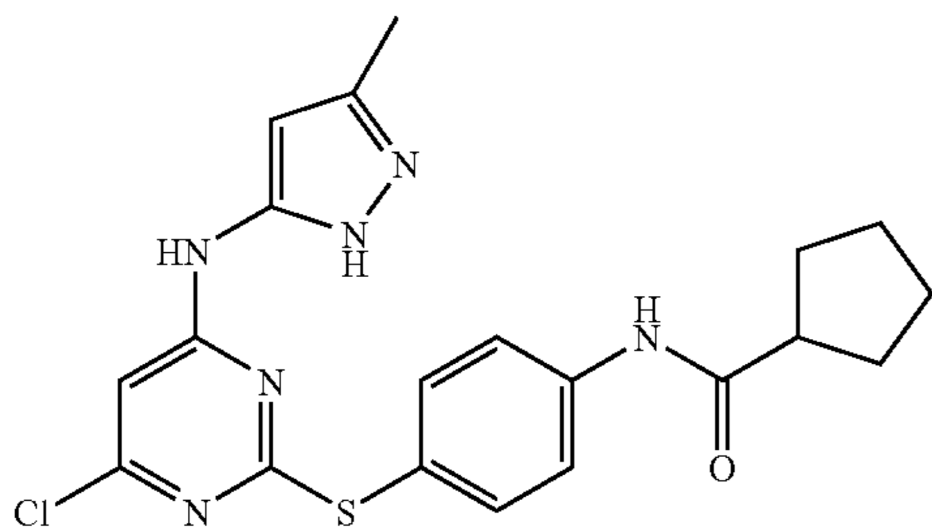
N-(4-(4-(3-methyl-1H-pyrazol-5-ylamino)-6-chloropyrimidin-2-ylthio)phenyl)cyclopentanecarboxamide
