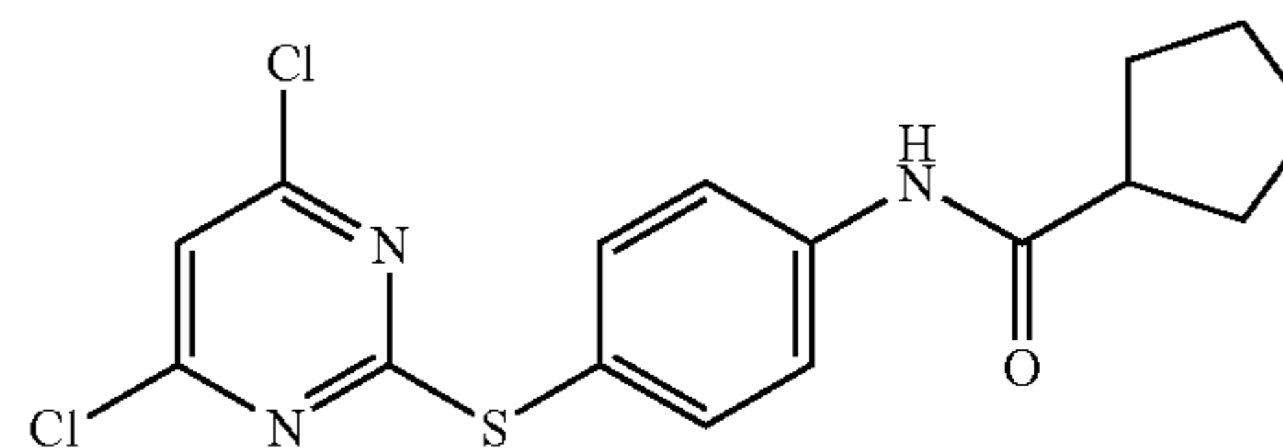
N-(4-(4,6-dichloropyrimidin-2-ylthio)phenyl)cyclopentane carboxamide
