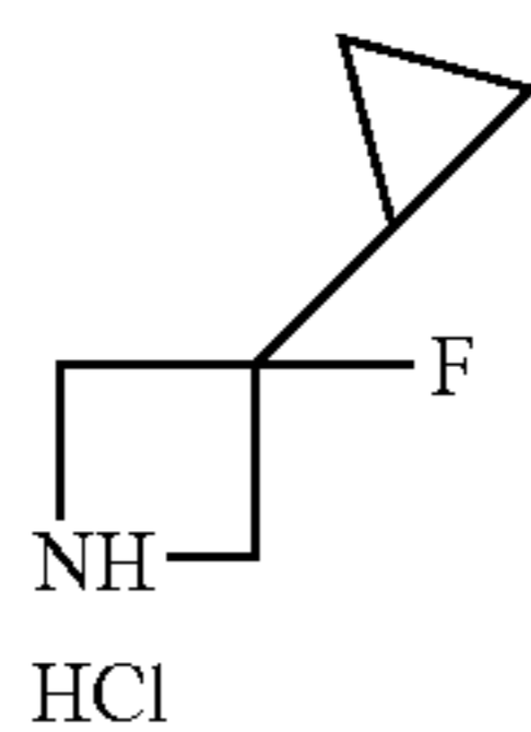
3-cyclopropyl-3-fluoroazetidine hydrochloride
