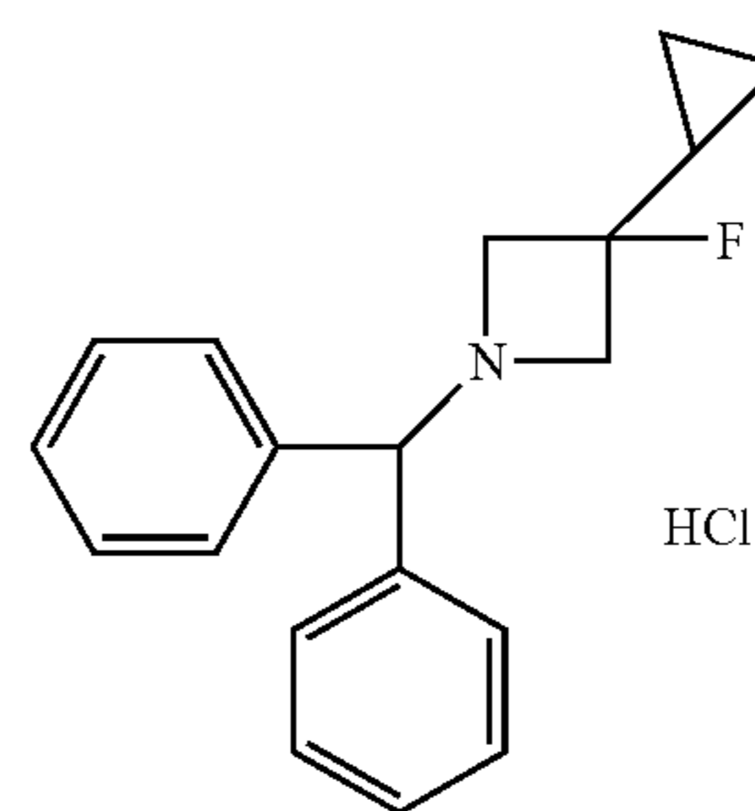
1-Benzhydryl-3-cyclopropyl-3-fluoroazetididine hydrochloride
