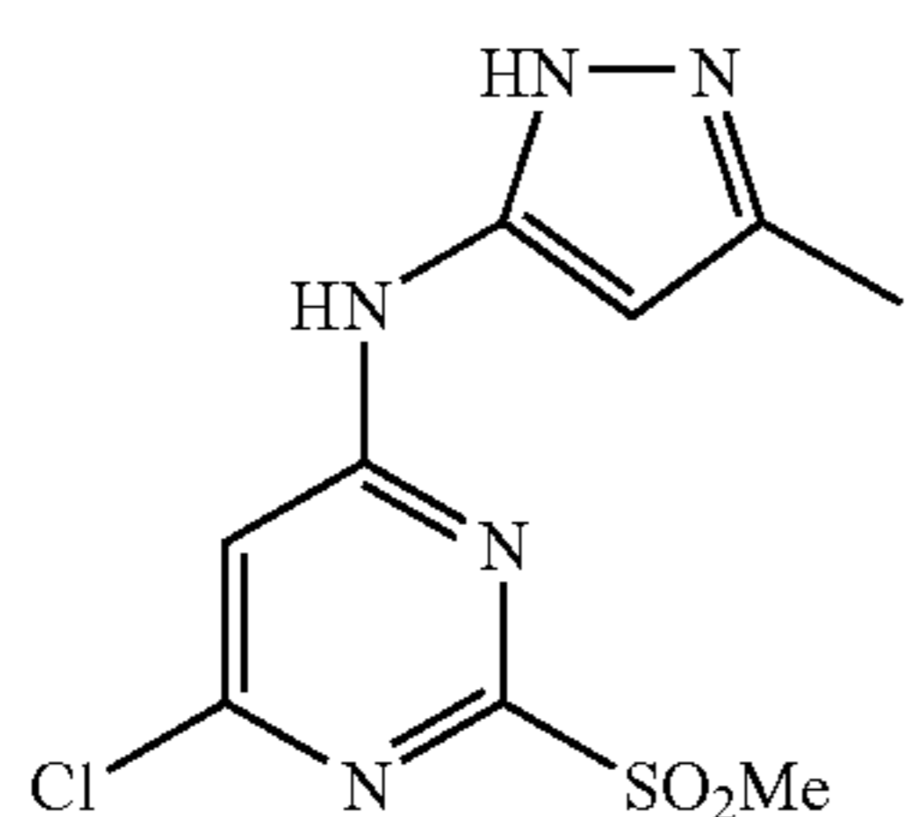
6-chloro-N-(3-methyl-1H-pyrazol-5-yl)-2-(methylsulfonyl)pyrimidin-4-amine
