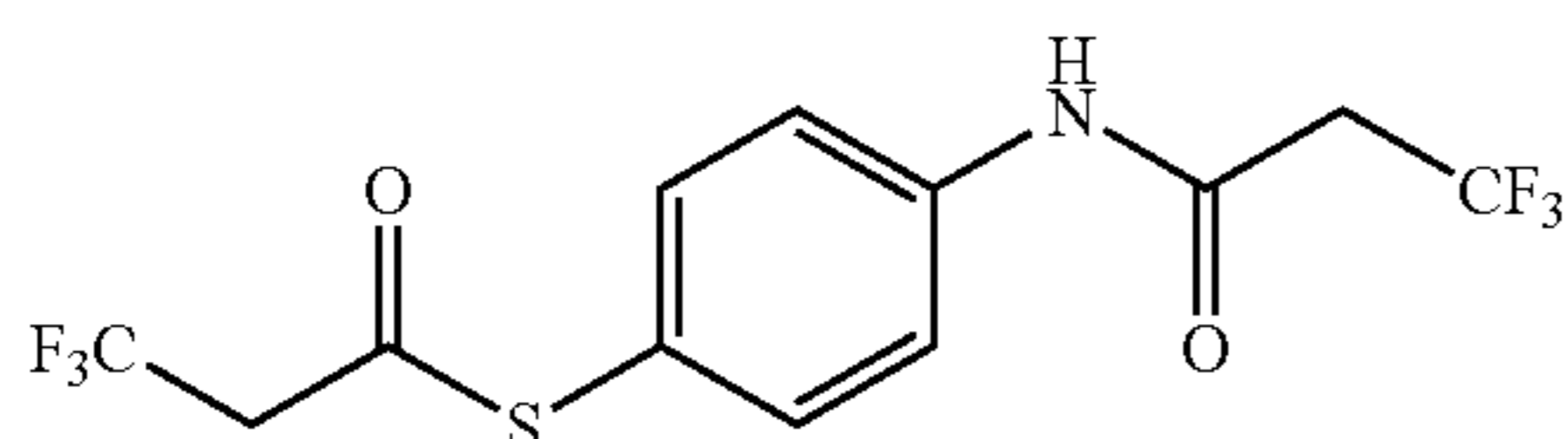
S-4-(3,3,3-trifluoropropanamido)phenyl 3,3,3-trifluoropropanethioate
