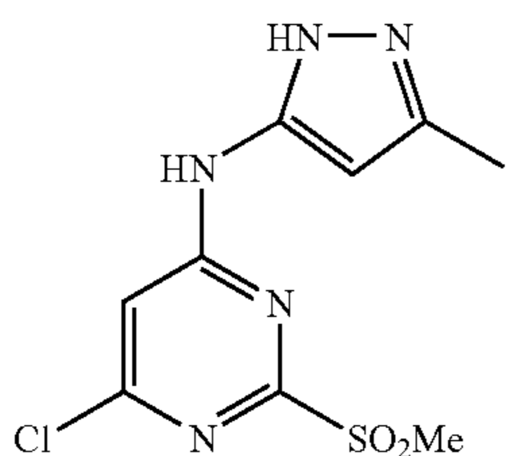
6-chloro-N-(3-methyl-1H-pyrazol-5-yl)-2-(methylsulfonyl)pyrimidin-4-amine
