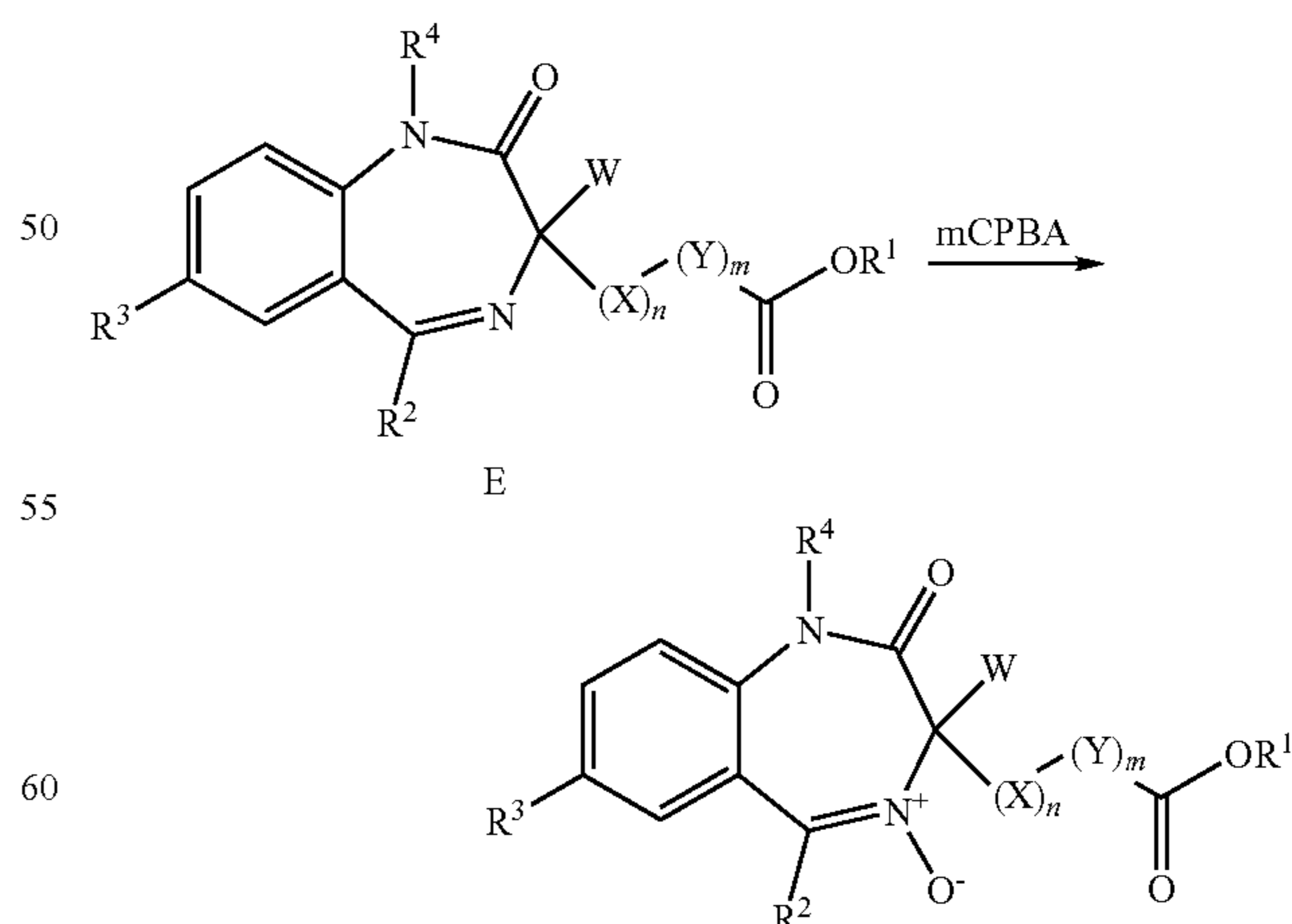
SCHEME 1b
