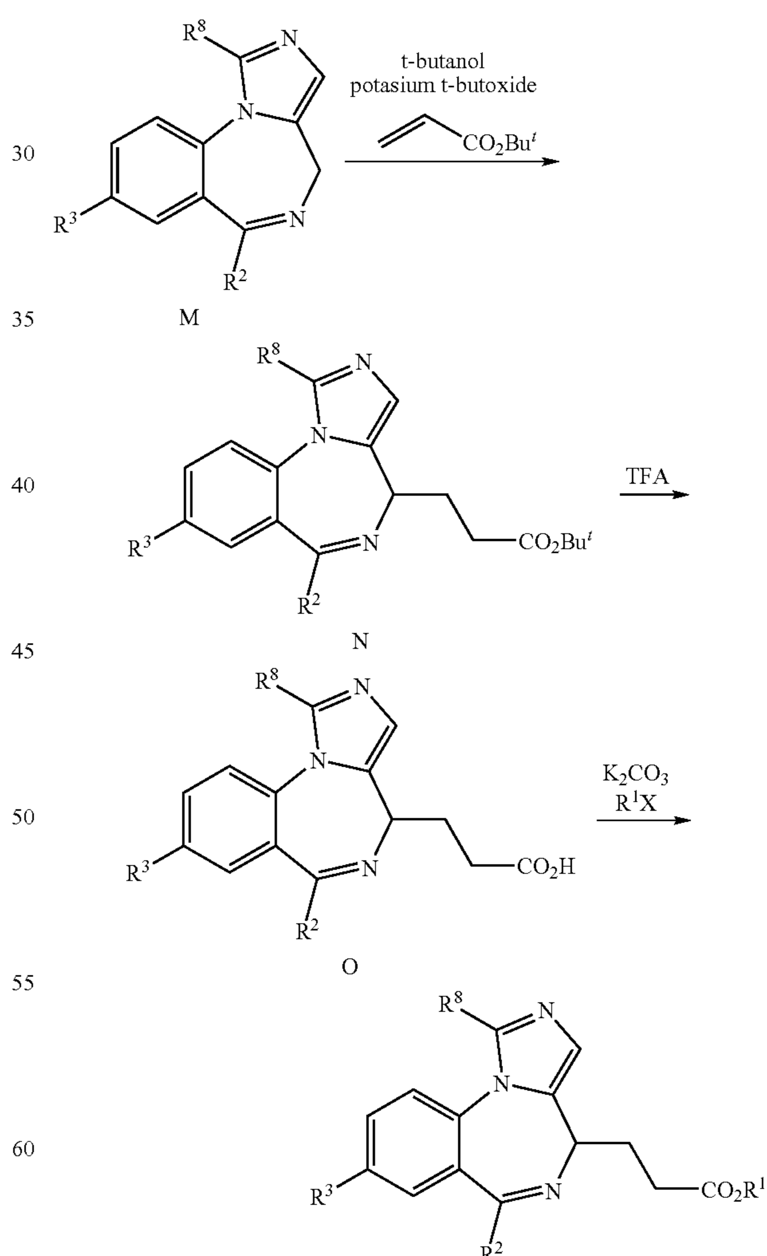
SCHEME 6
