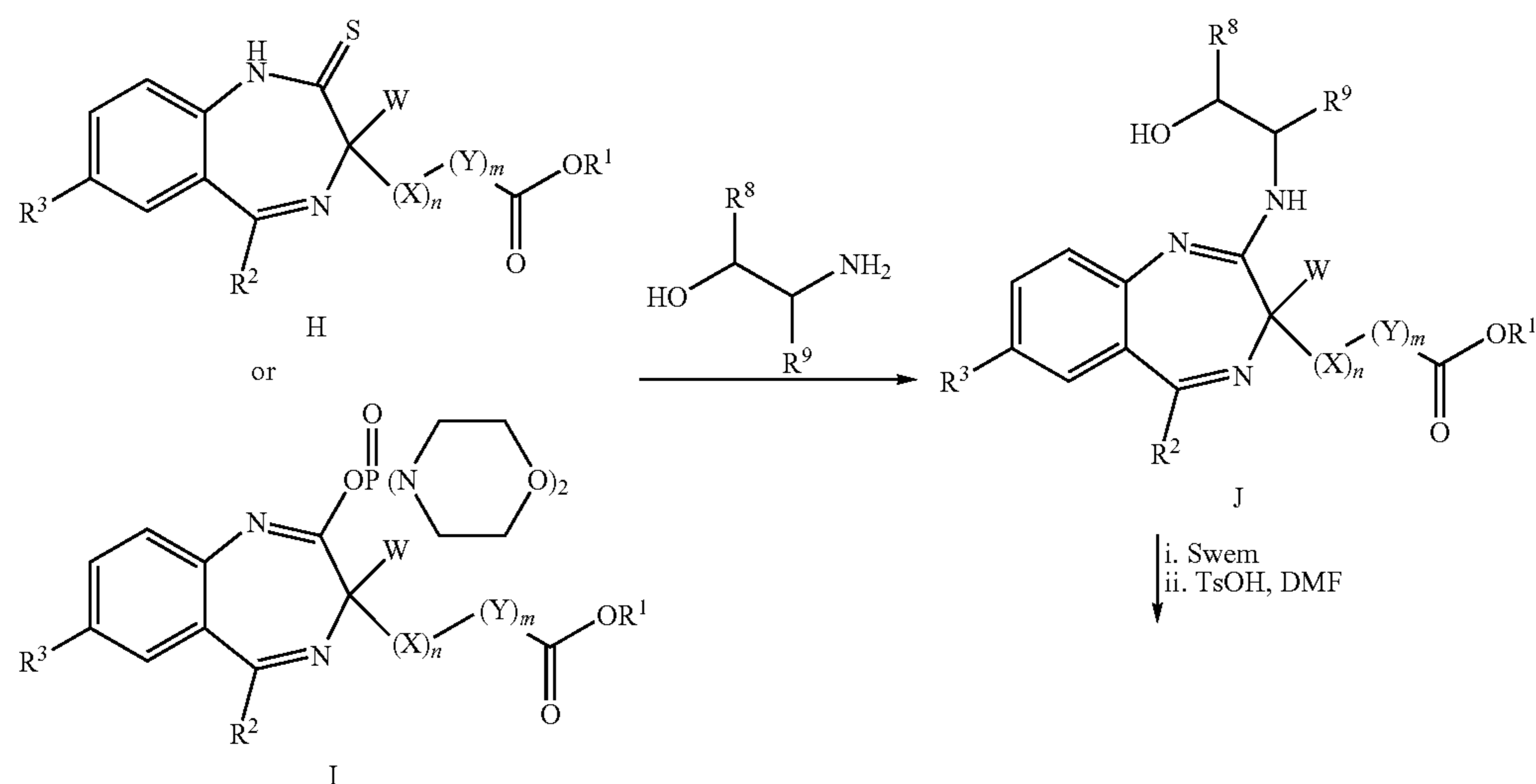
SCHEME 4
