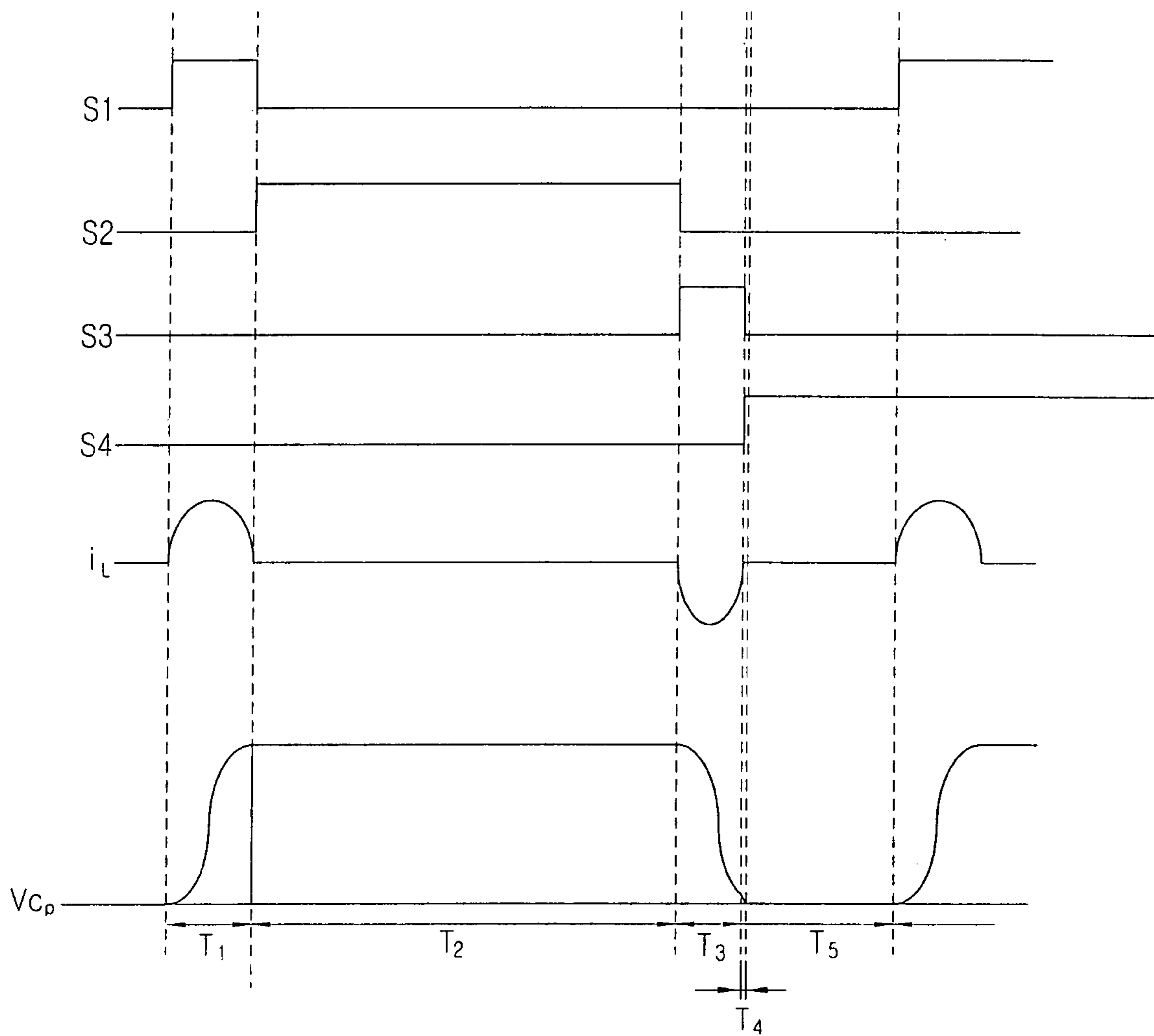
FIG. 4 CONVENTIONAL ART
