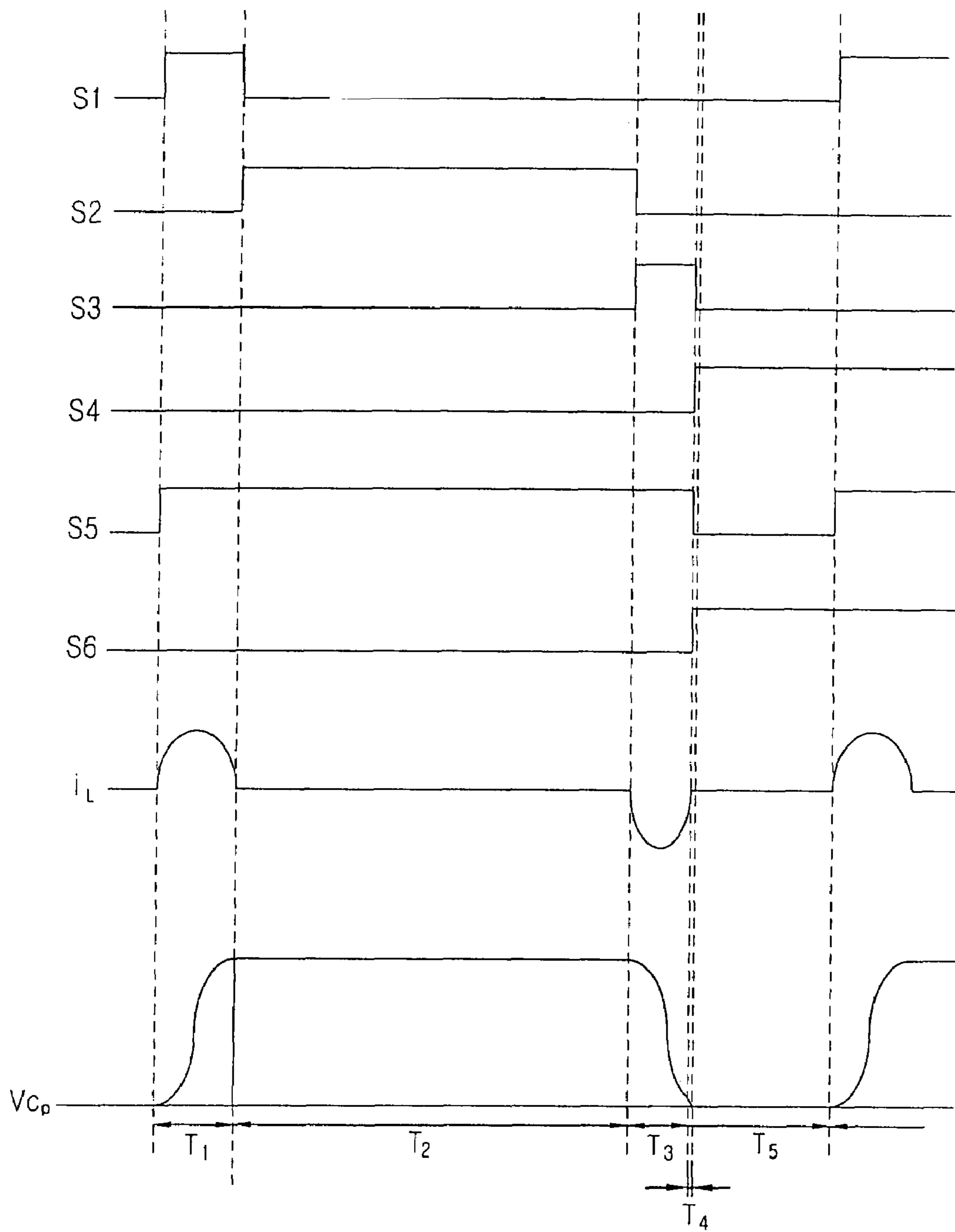
FIG. 6 CONVENTIONAL ART
