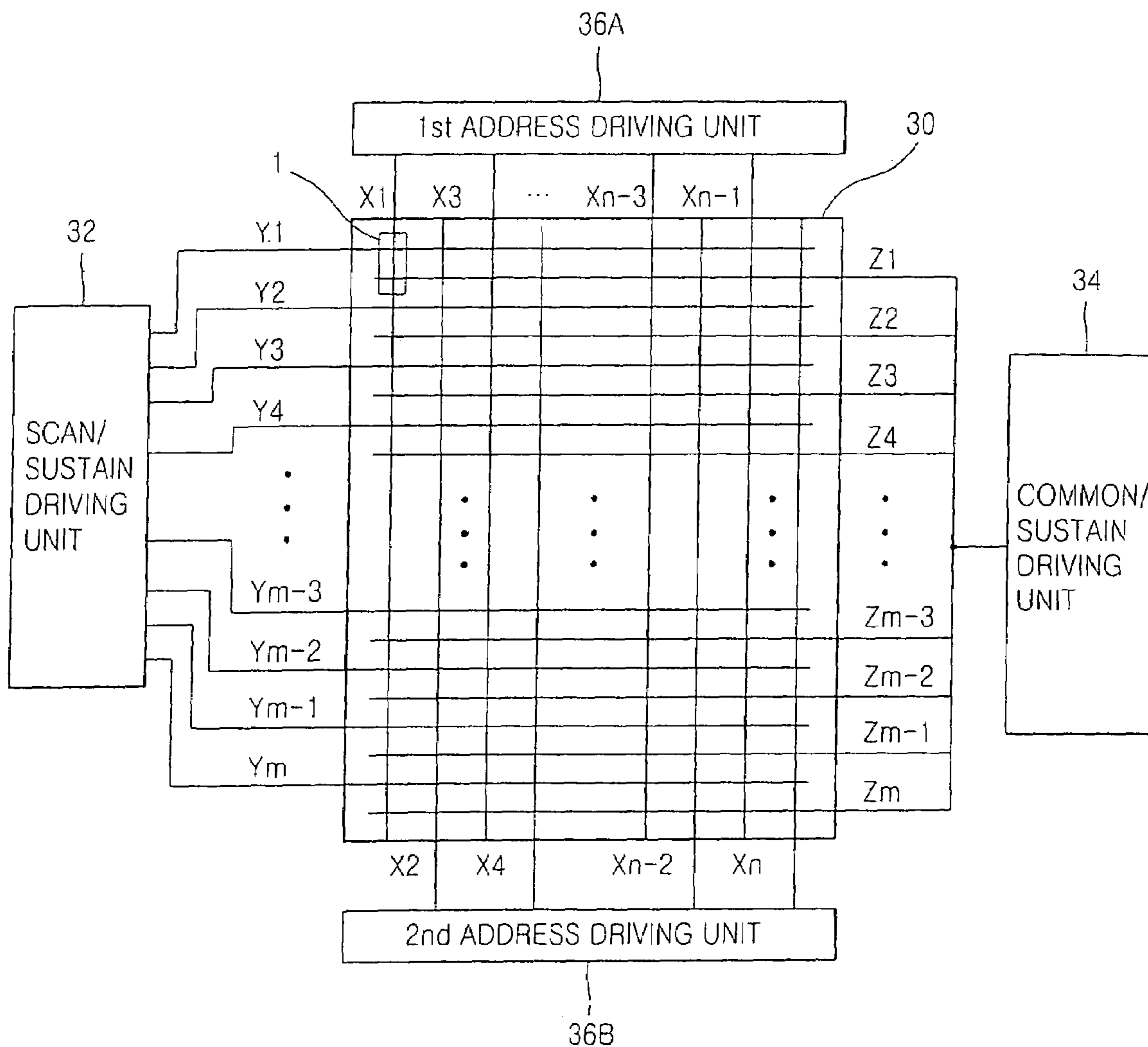
FIG. 2 CONVENTIONAL ART
