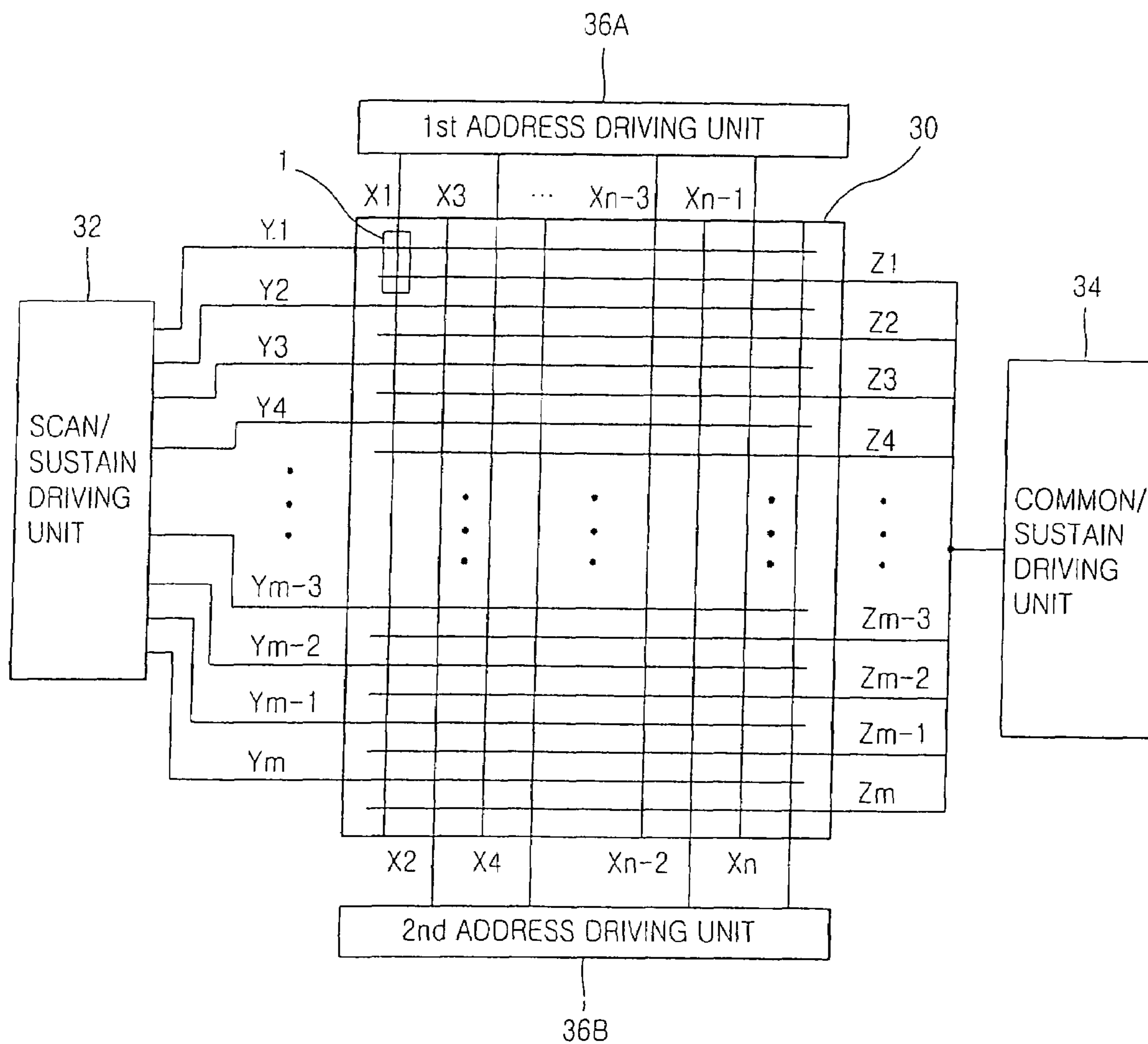
FIG. 2 CONVENTIONAL ART
