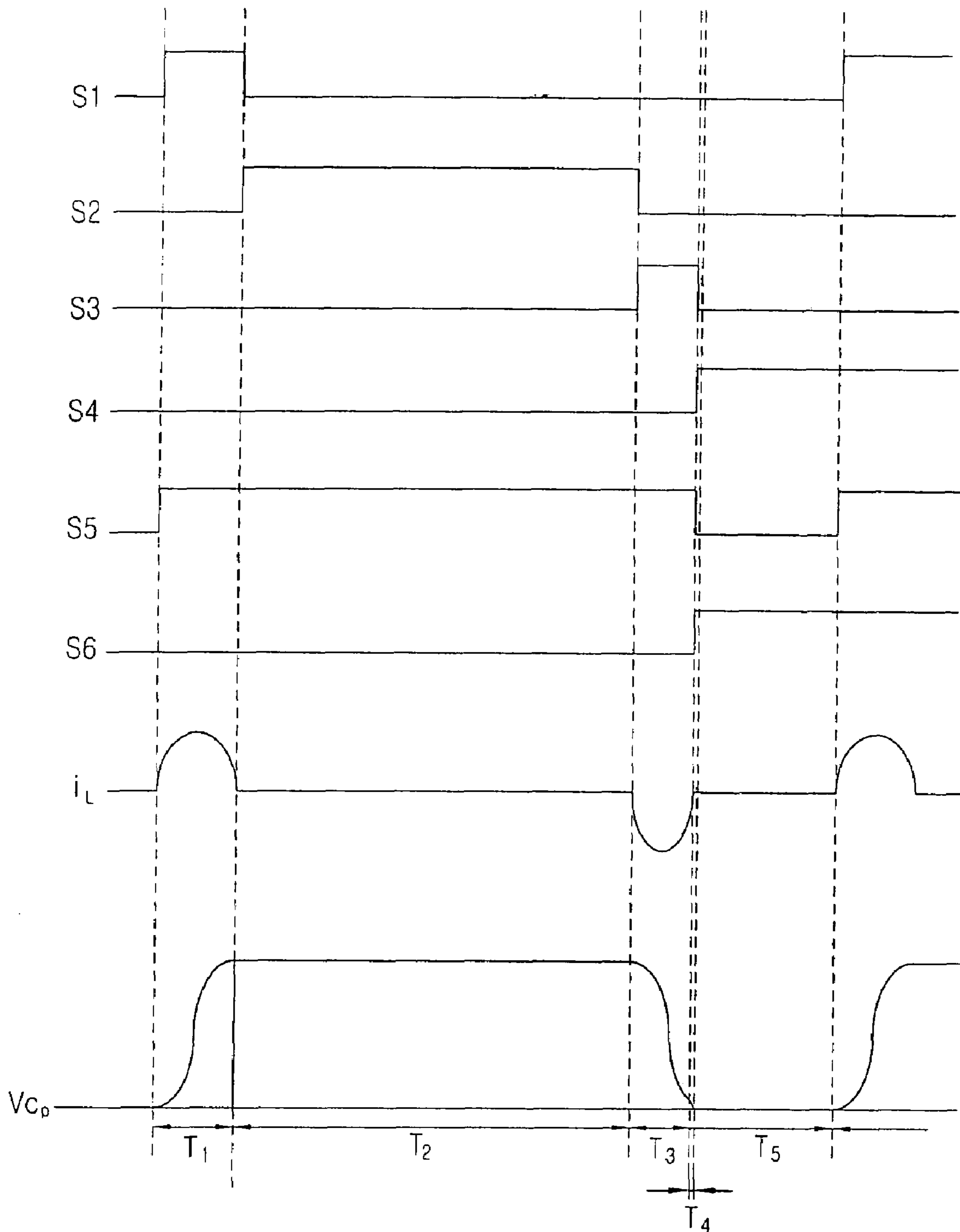
FIG. 6 CONVENTIONAL ART
