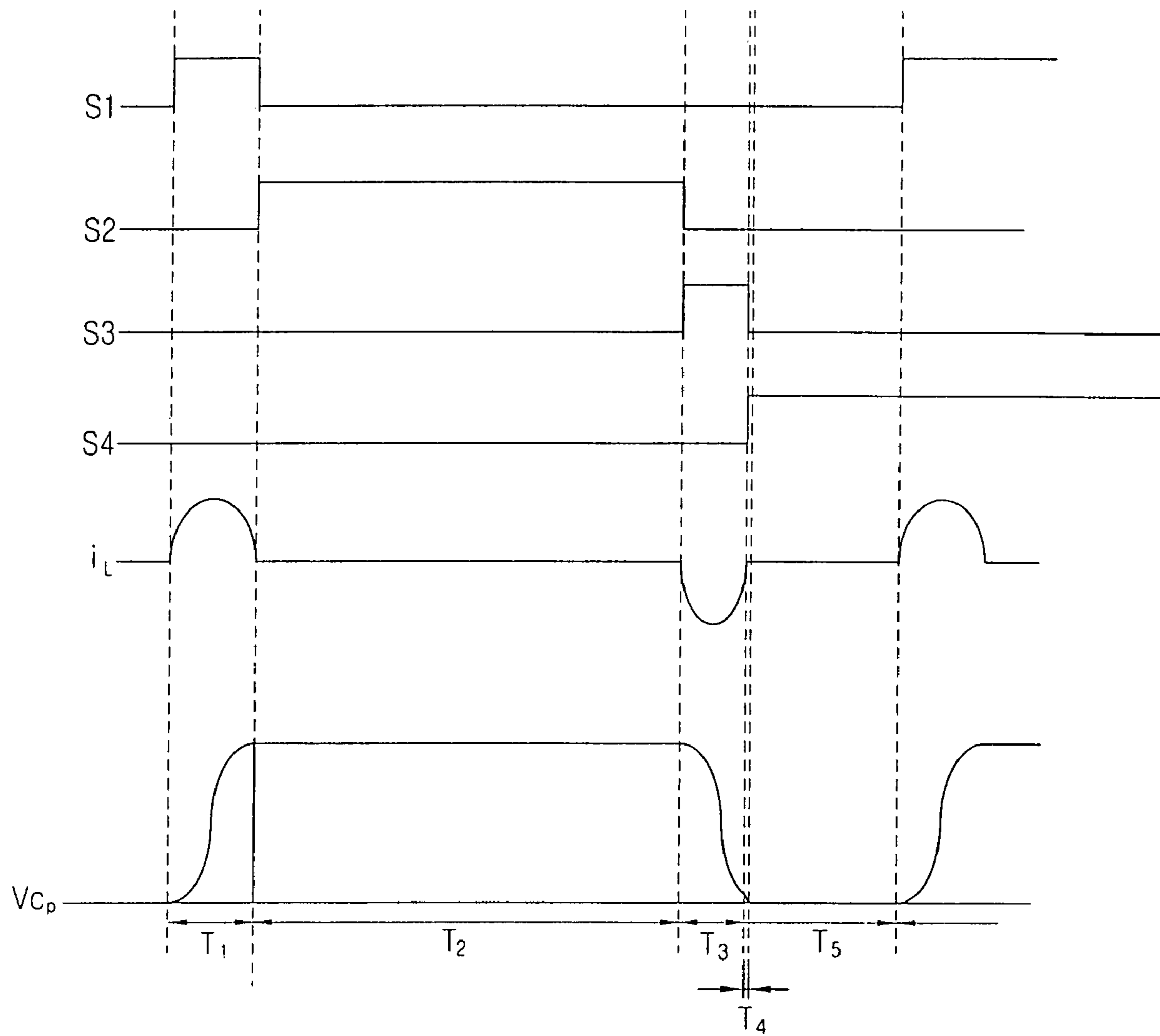
FIG. 4 CONVENTIONAL ART
