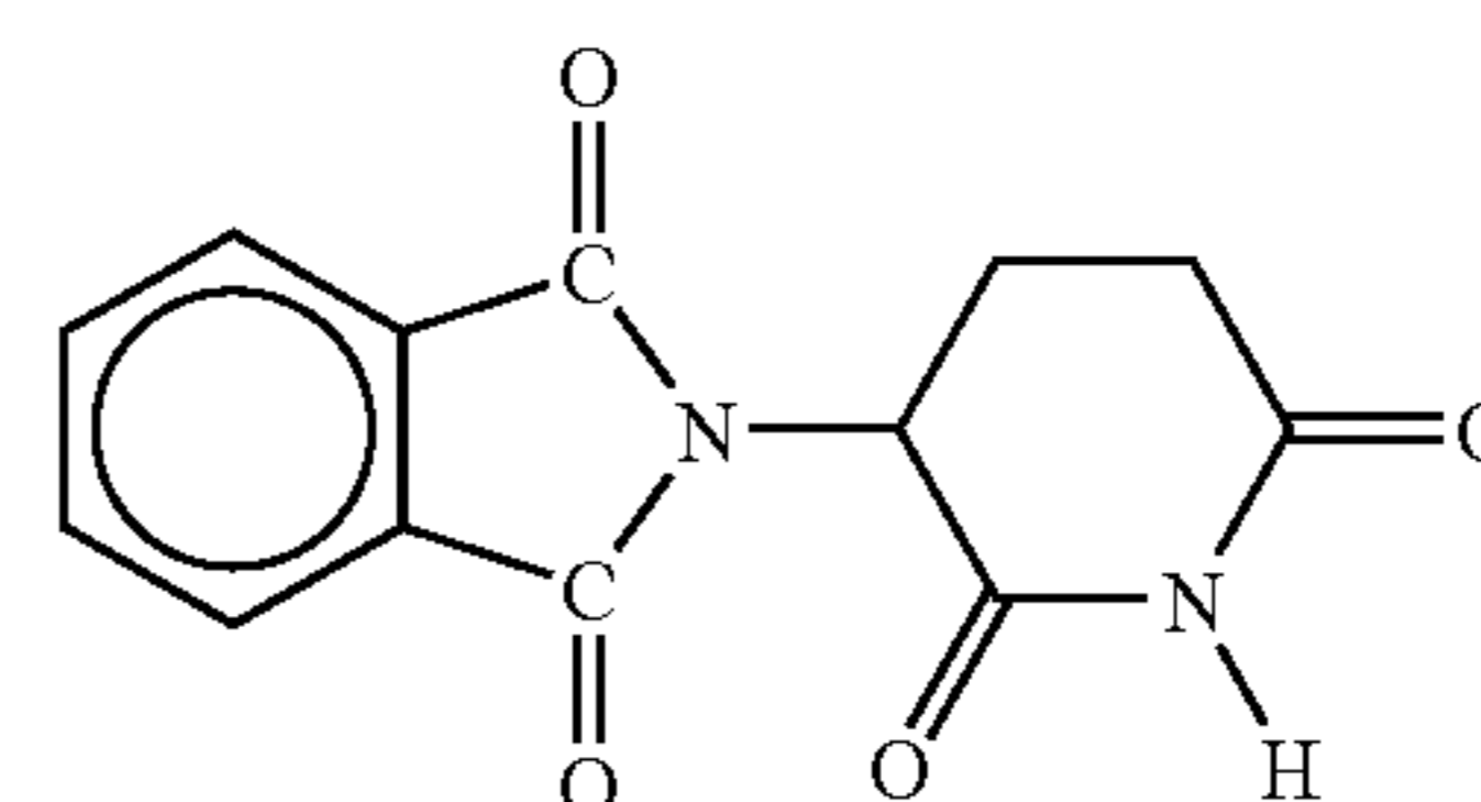
thalidomide
