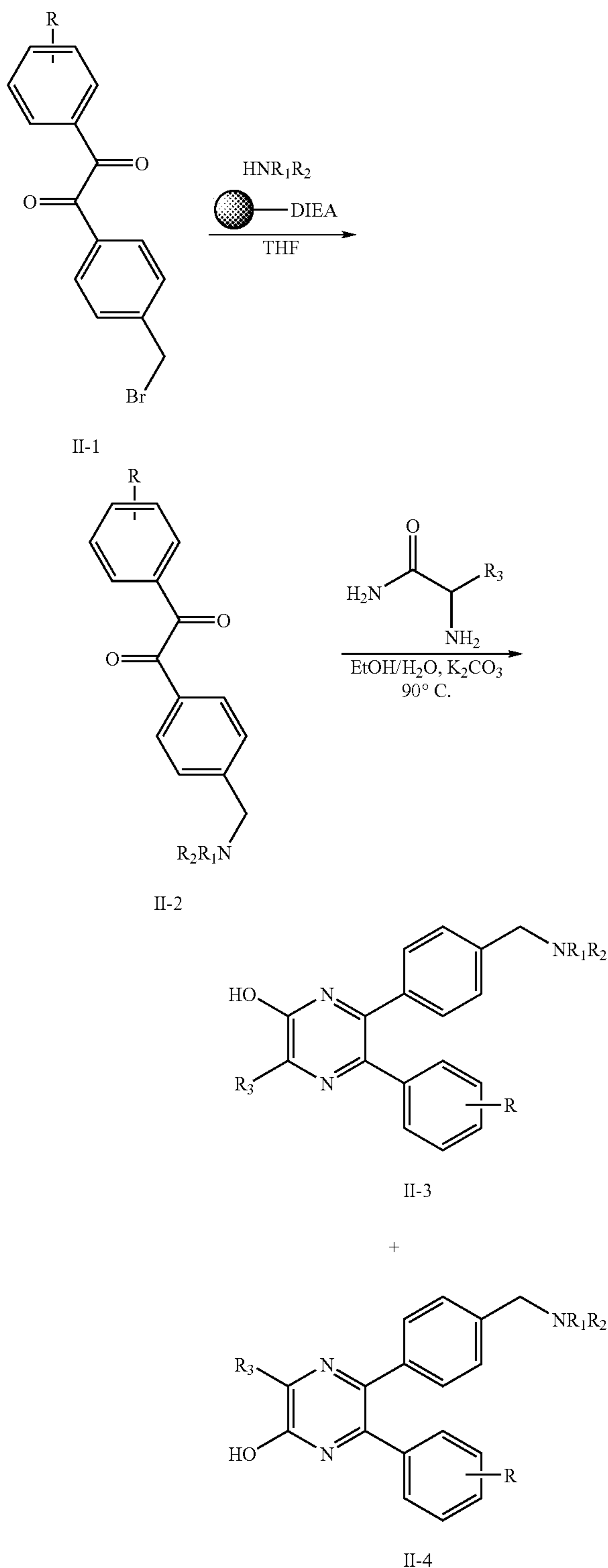
Reaction Scheme II
