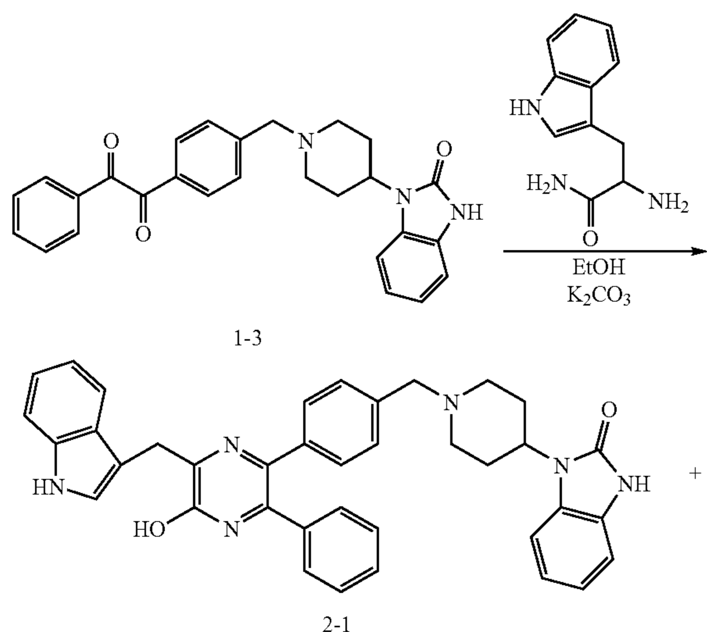
SCHEME 2
