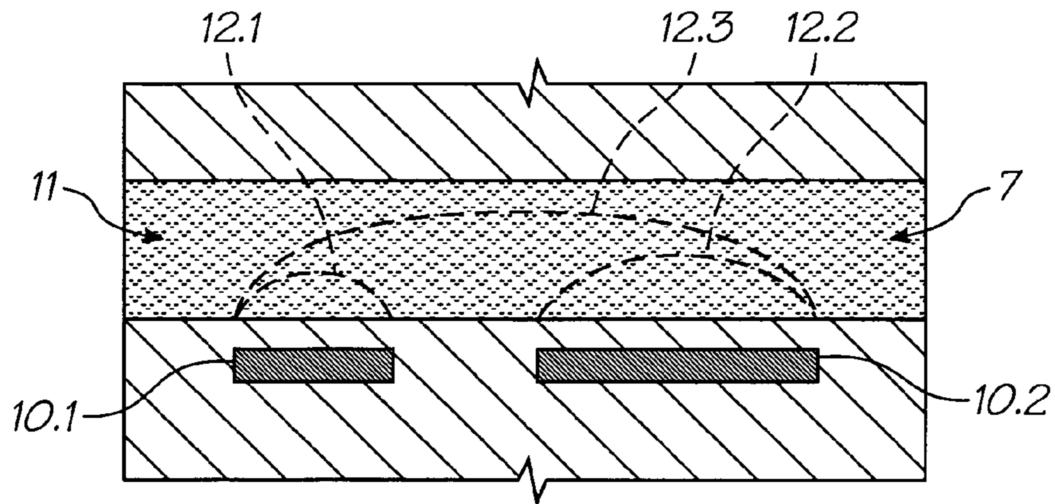
FIG. 52 (PRIOR ART)
