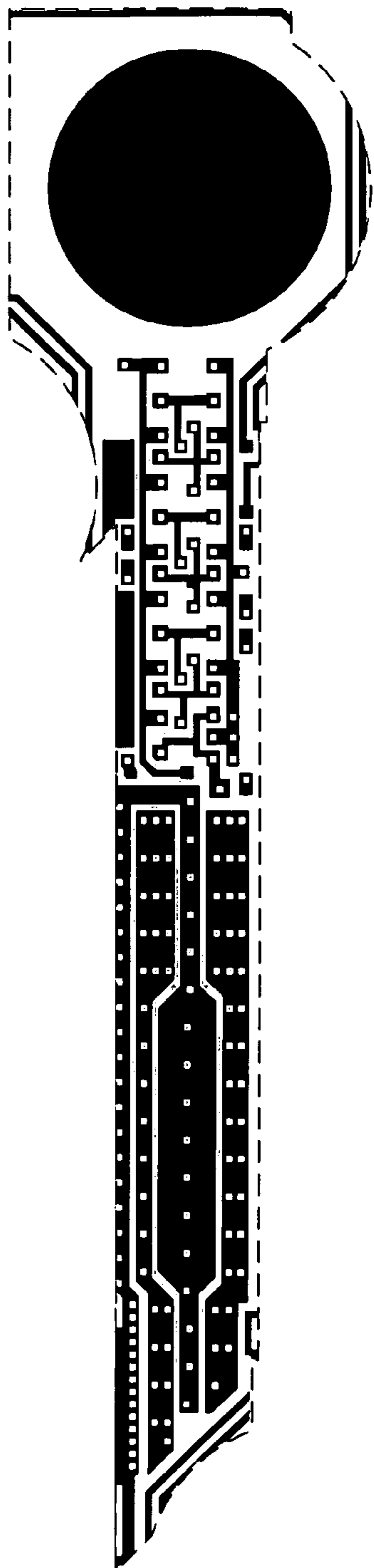
Metal 1 mask
