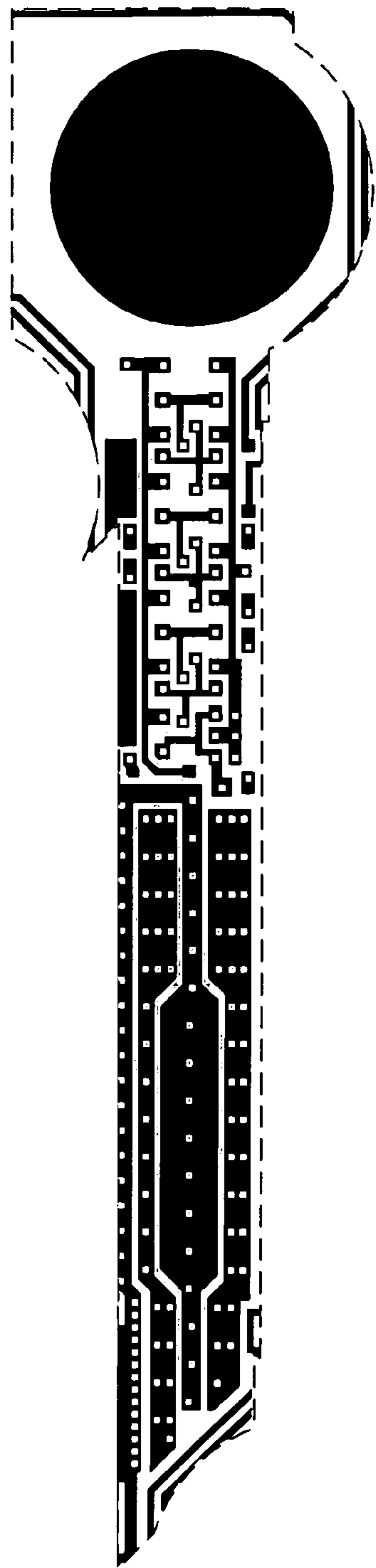
Metal 1 mask
