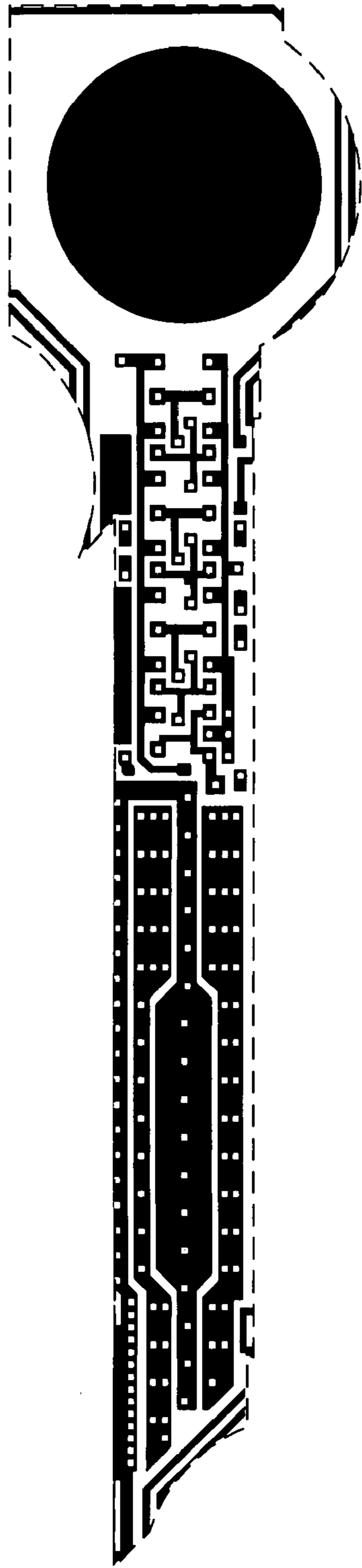
Metal 1 mask
