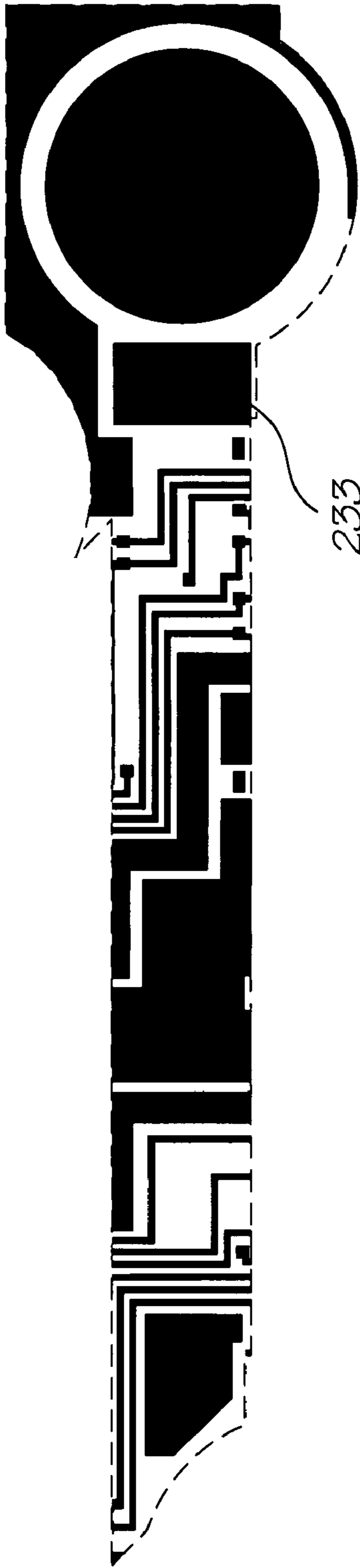
Metal 2 mask
