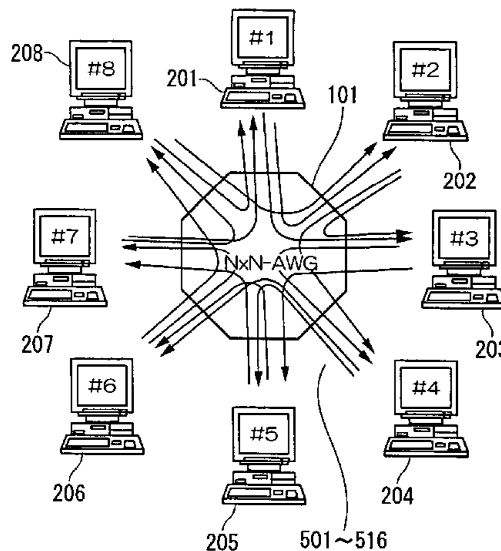
POINT-TO-POINT TRAFFIC=3 (3/N PER NODE)
