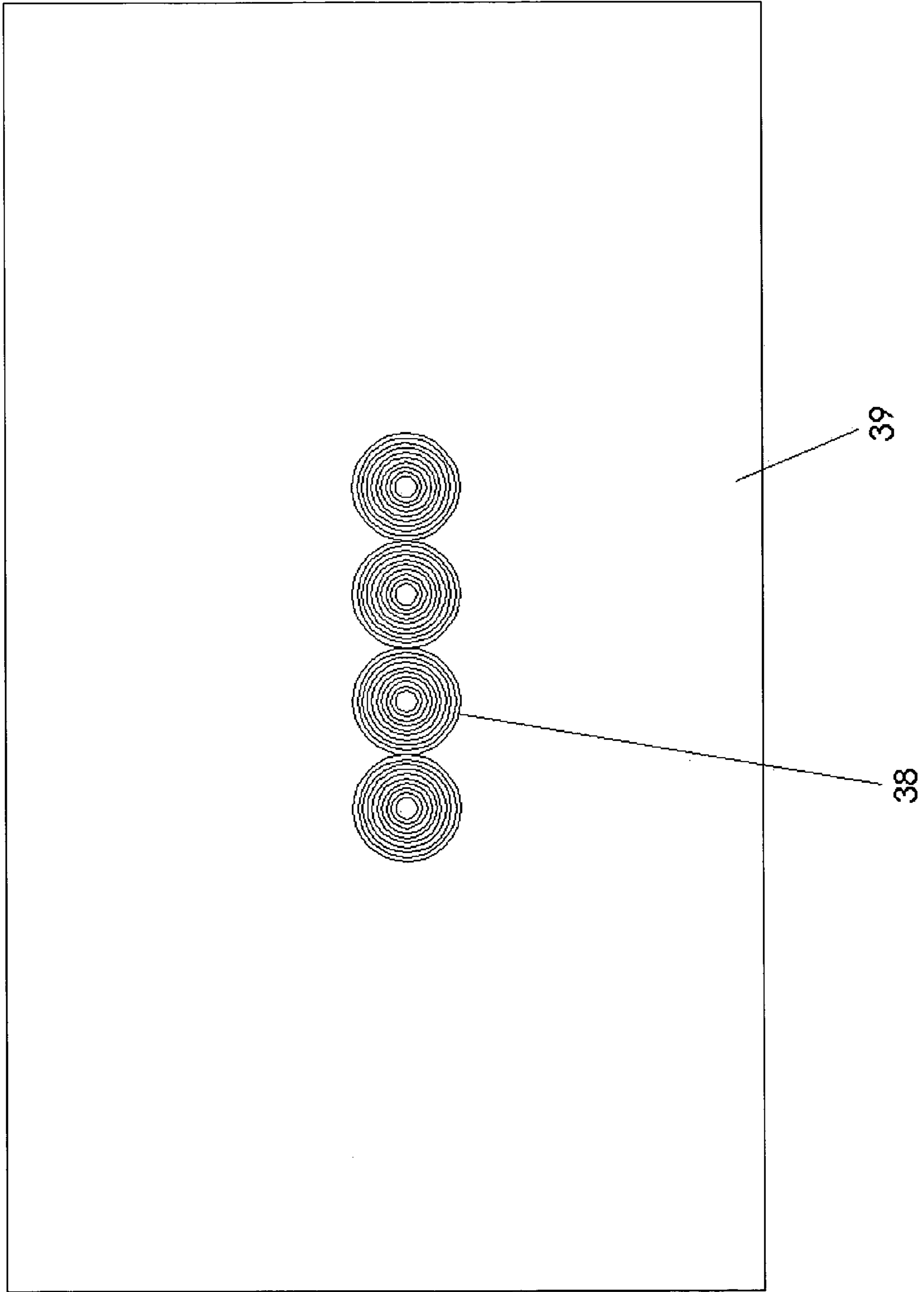
Figure 20 - Microlens Array on Glass Substrate (Top)
