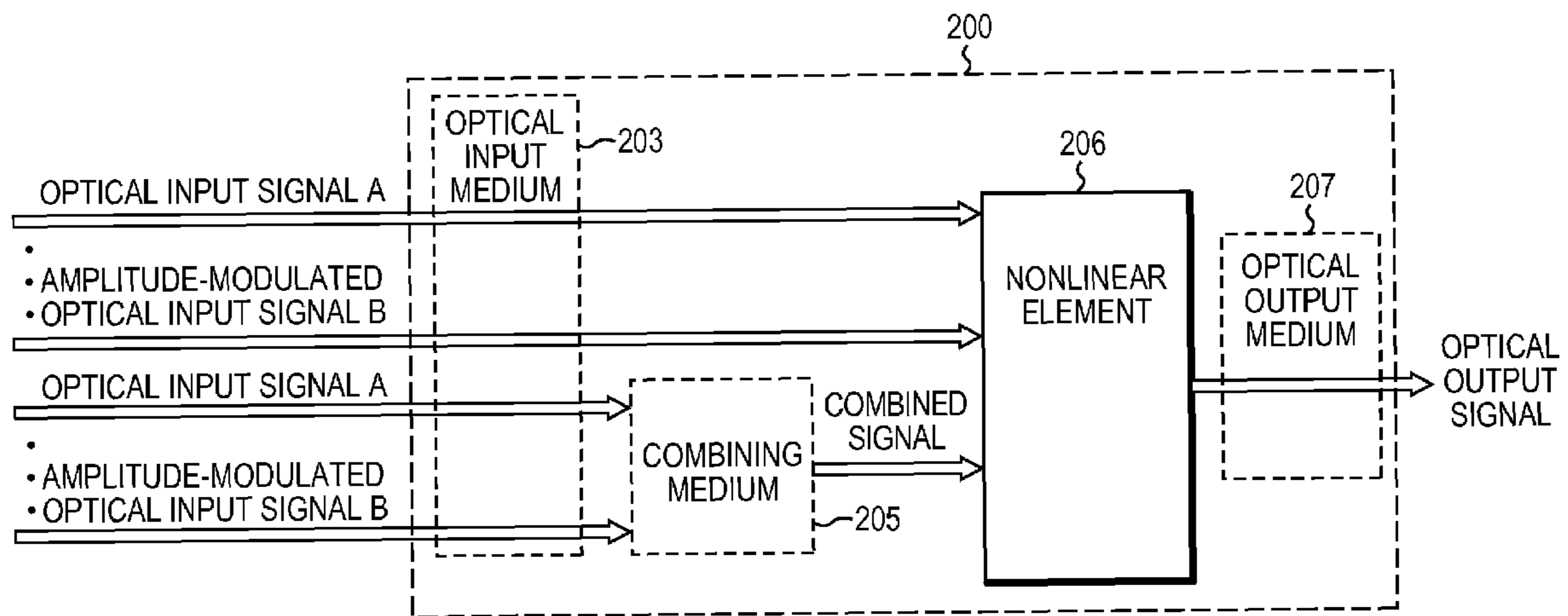
GENERALIZED ALL-OPTICAL LOGICAL GATE
