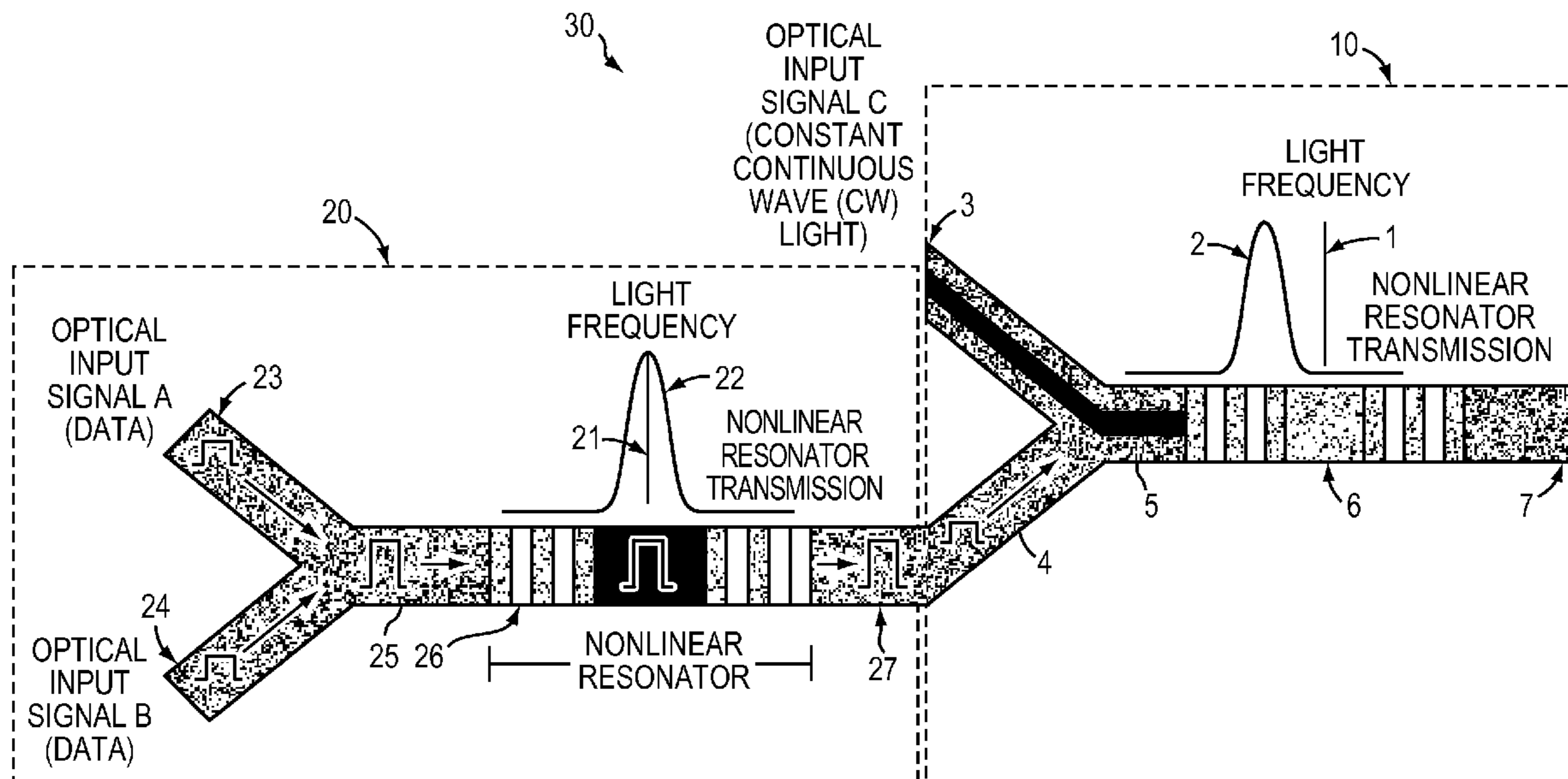
ALL-OPTICAL NAND GATE RECEIVING 1 BITS AS OPTICAL INPUT SIGNALS AND OUTPUTTING A 0-BIT AS OPTICAL OUTPUT SIGNAL
