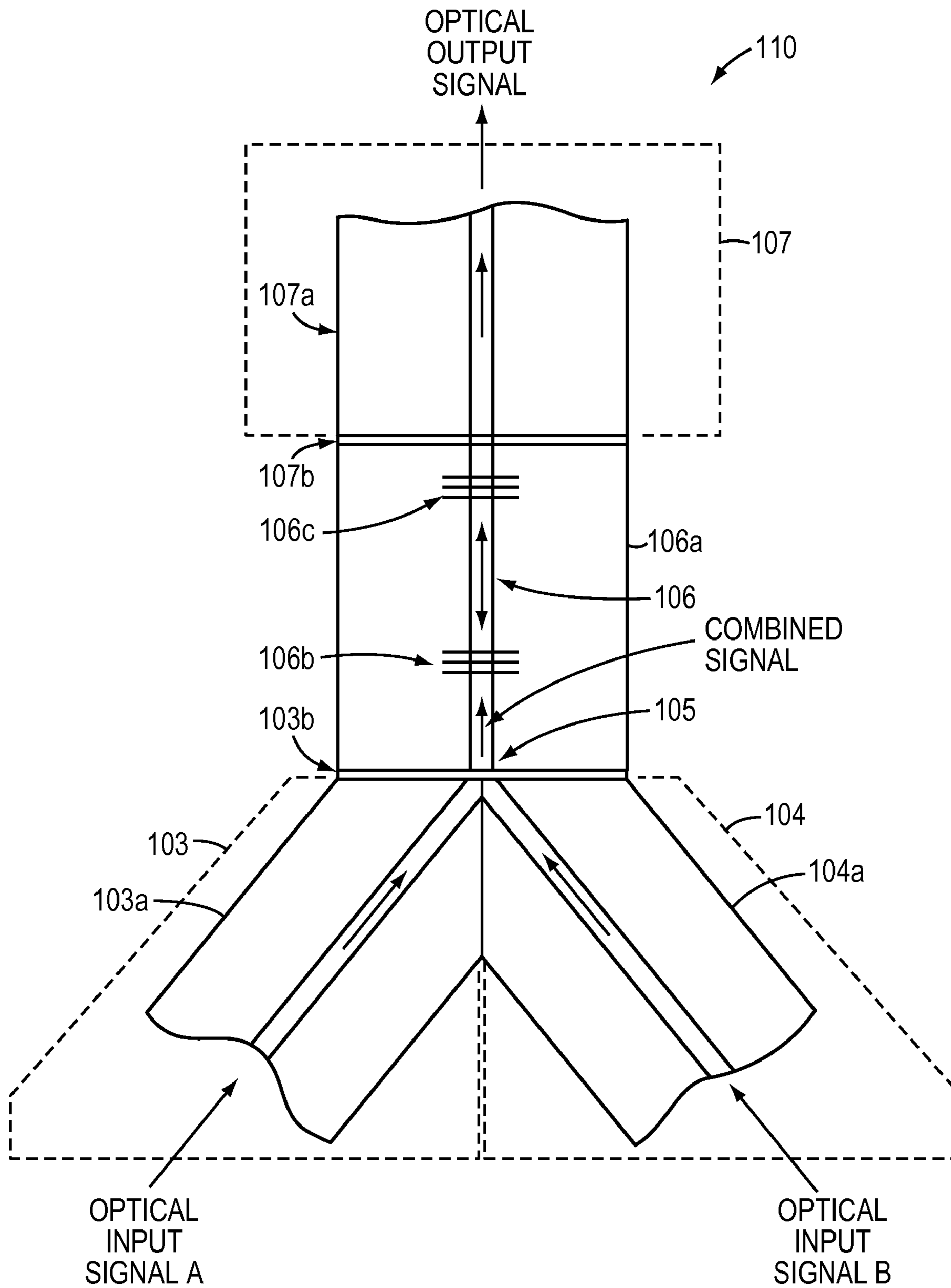
ALL-OPTICAL LOGICAL GATE IMPLEMENTED WITH OPTICAL FIBERS
