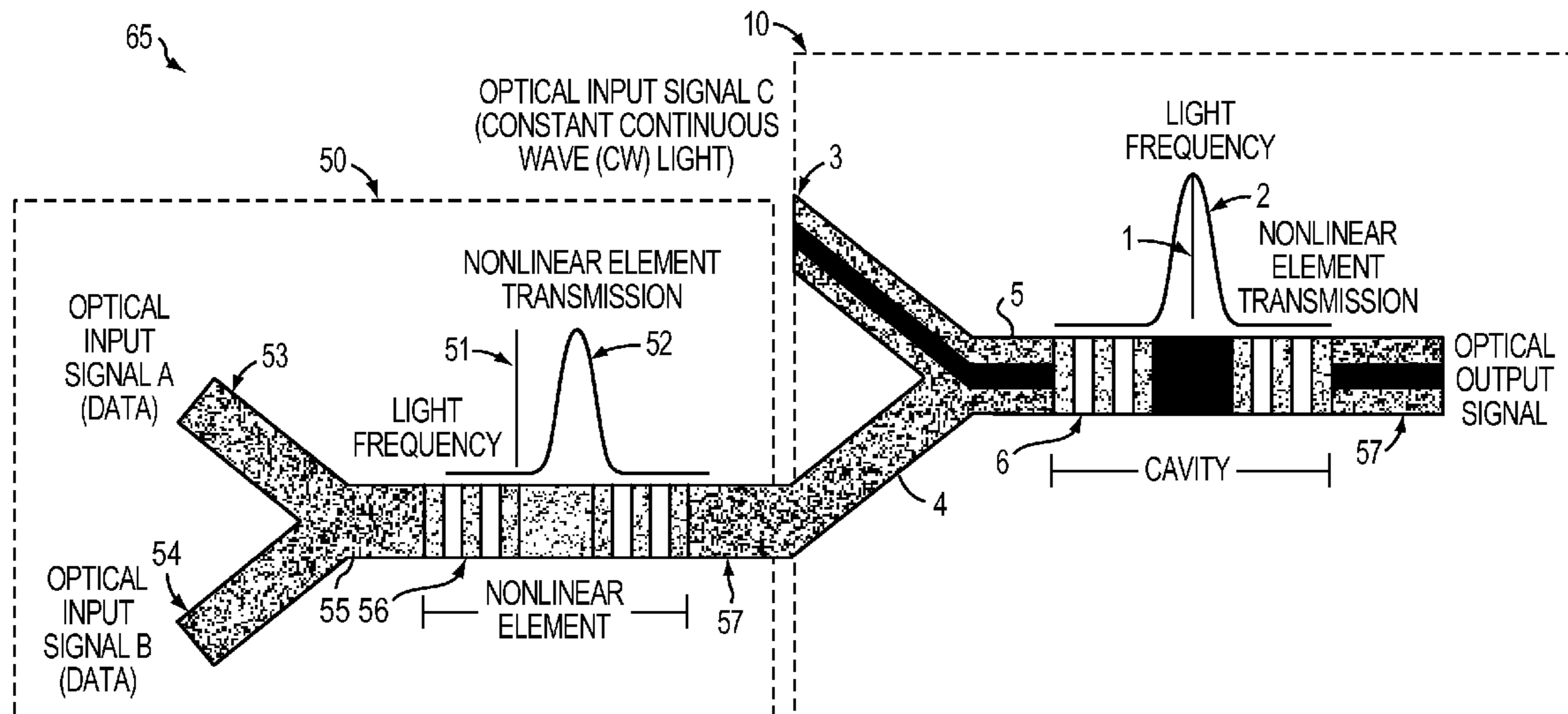
ALL-OPTICAL XNOR GATE WITH LOGIC LEVEL RESTORATION
