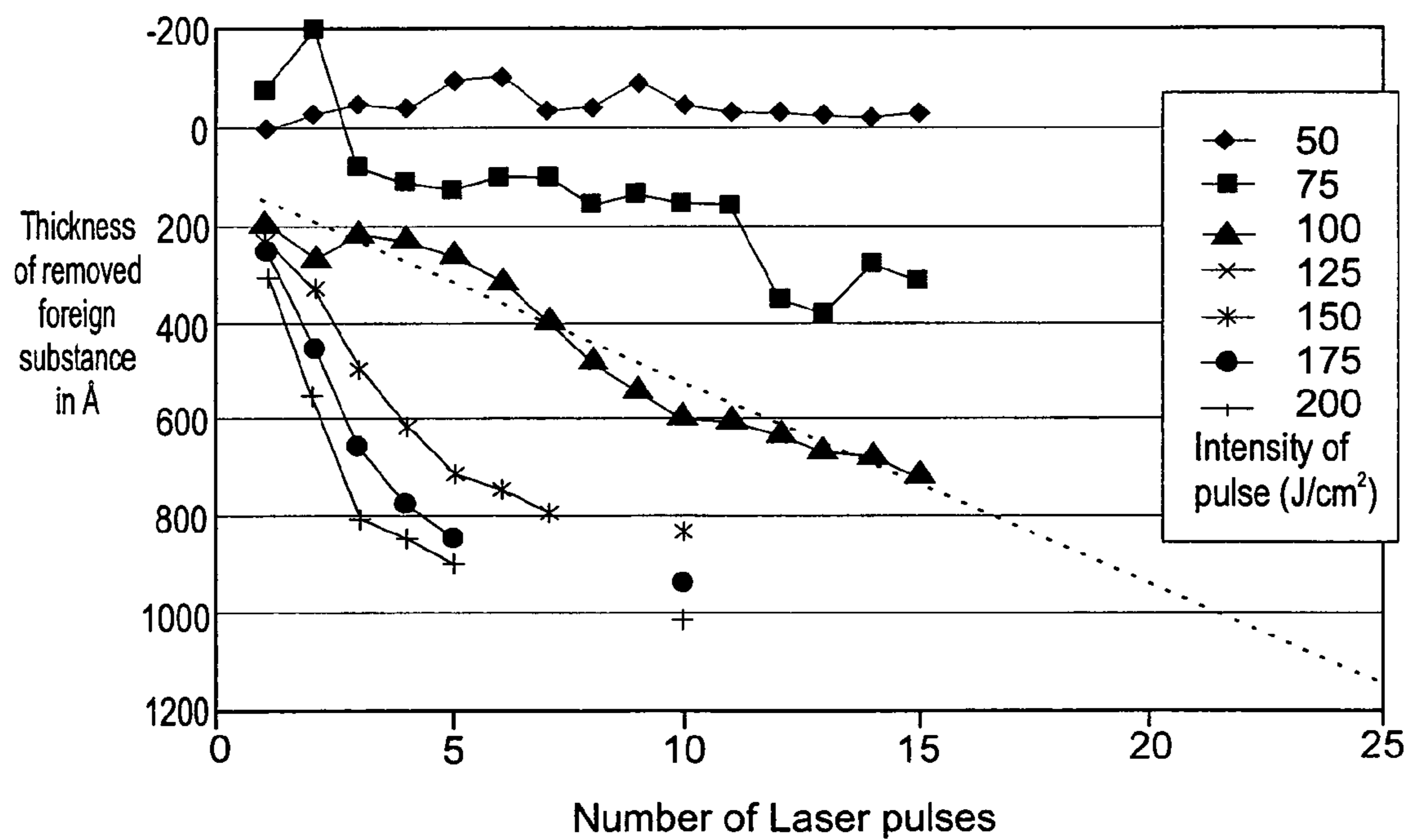
Laser Removal of Organic Emission Layer 150 absent Auxiliary Layers 120/130
