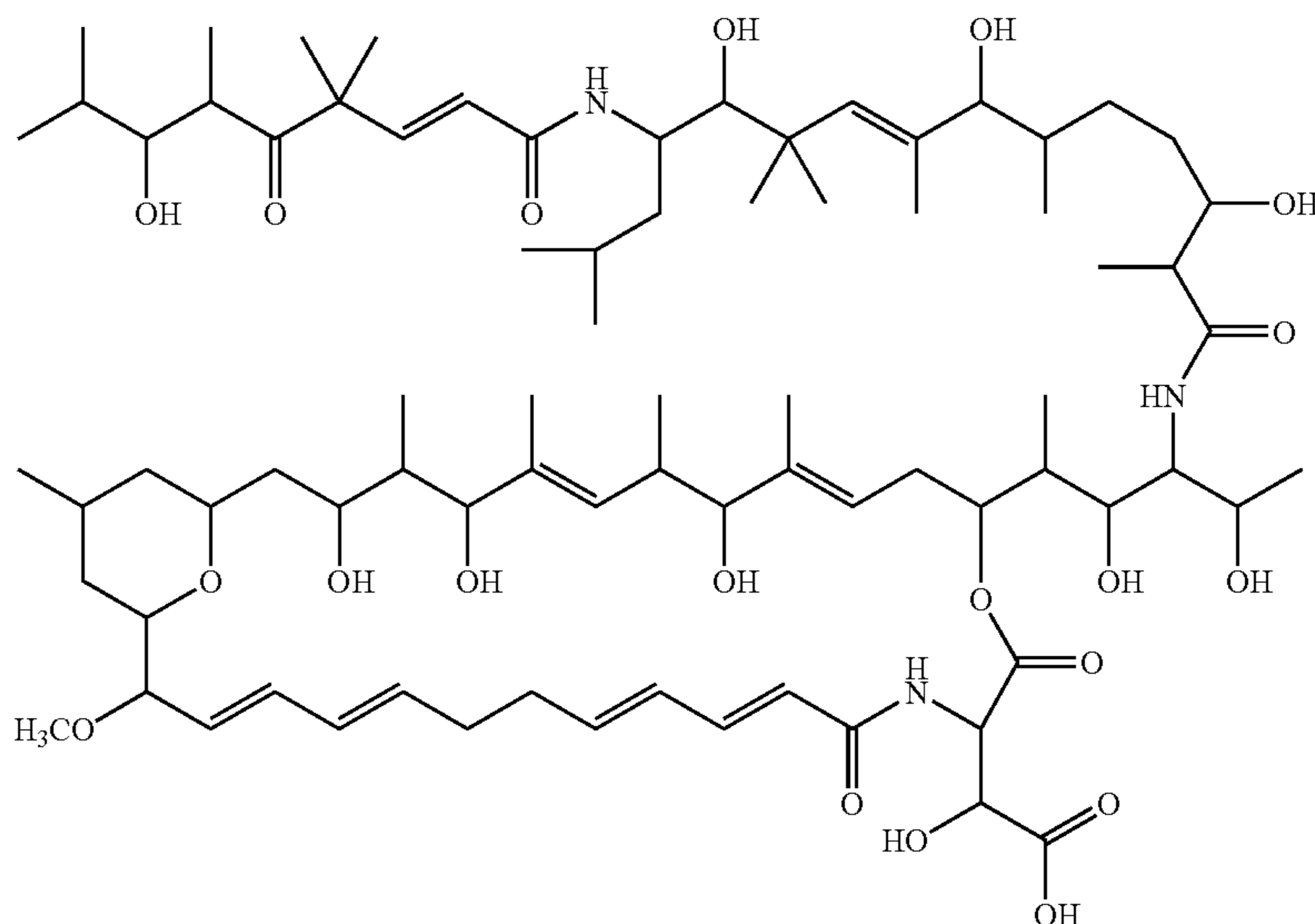
poecillastrin A (1)
