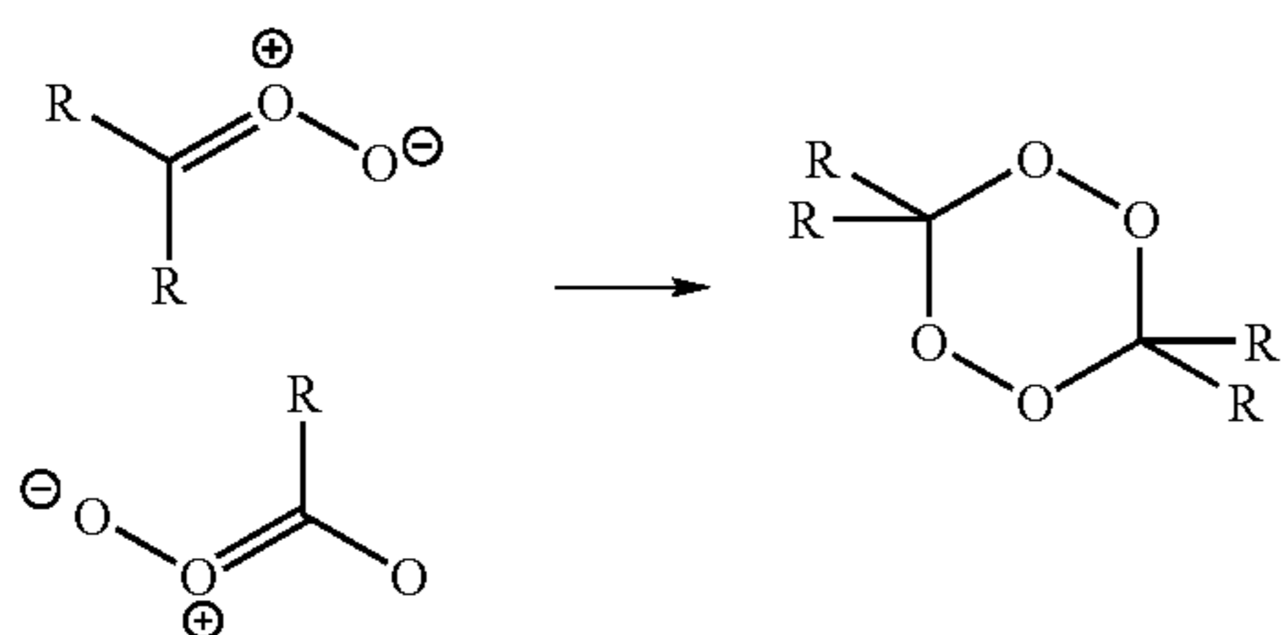
SCHEME 2
