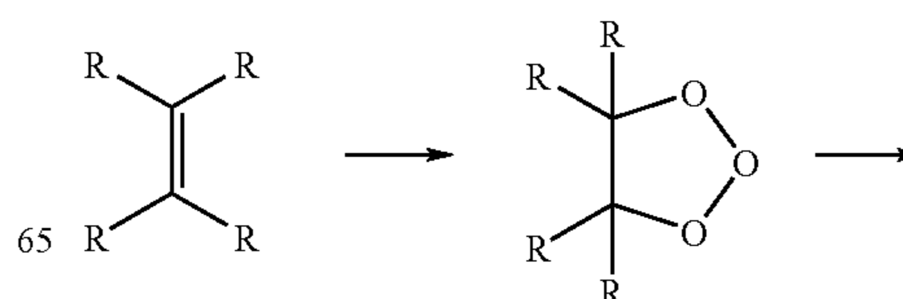
SCHEME 1
