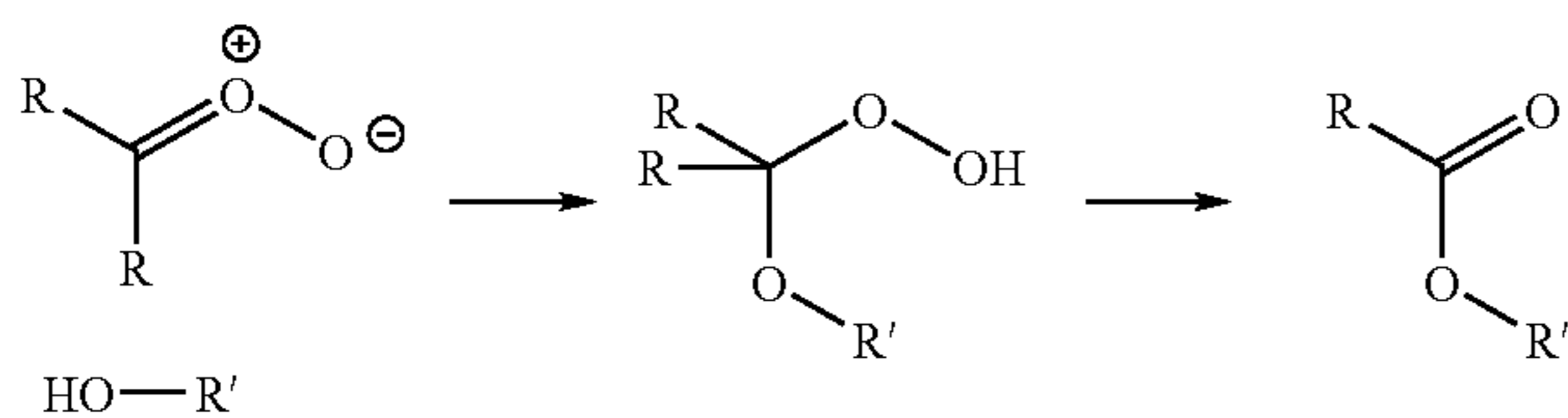
SCHEME 3
