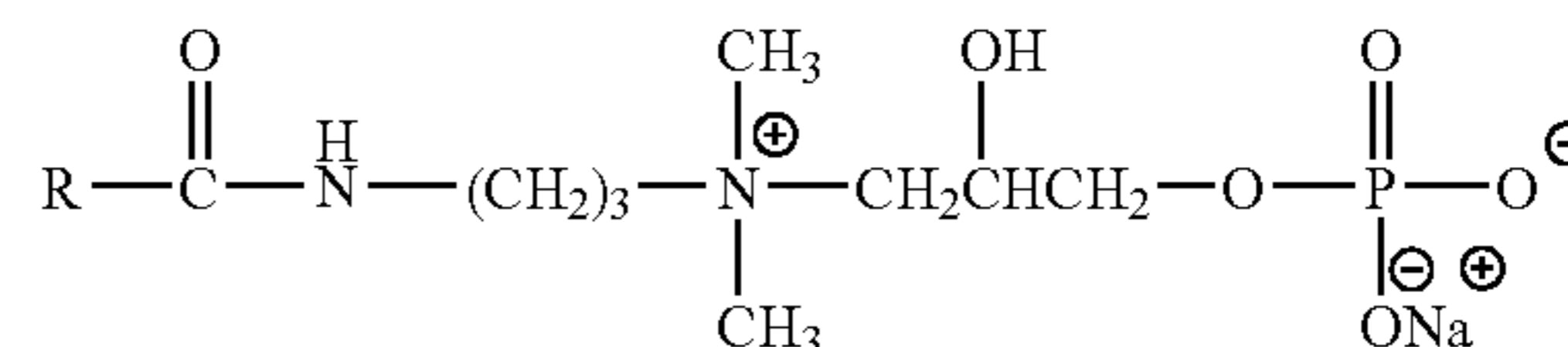
Structure 2A
