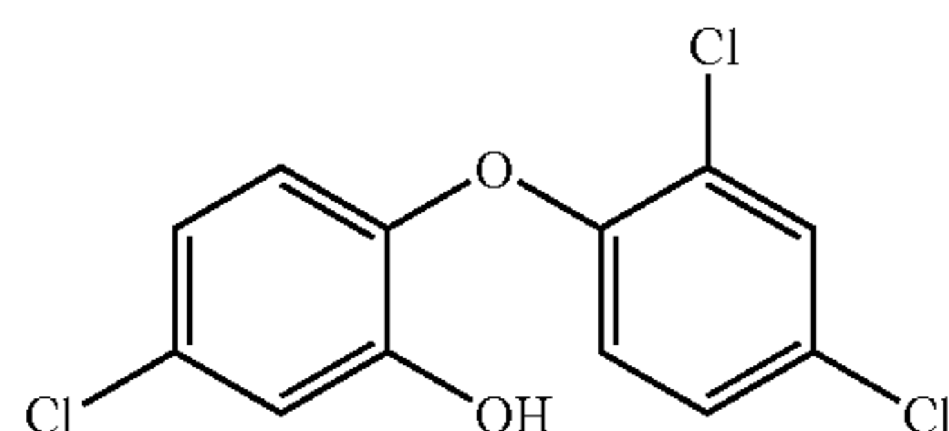
2,4,4'-trichloro-2'-hydroxydiphenyl ether
