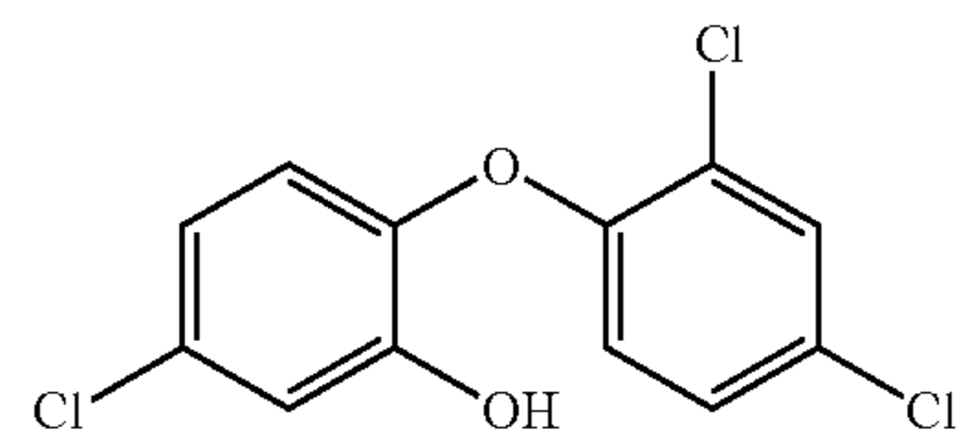
2,4,4'-trichloro-2'-hydroxydiphenyl ether
