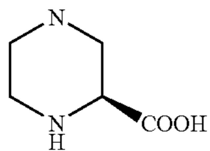
2-carboxy-piperazine
