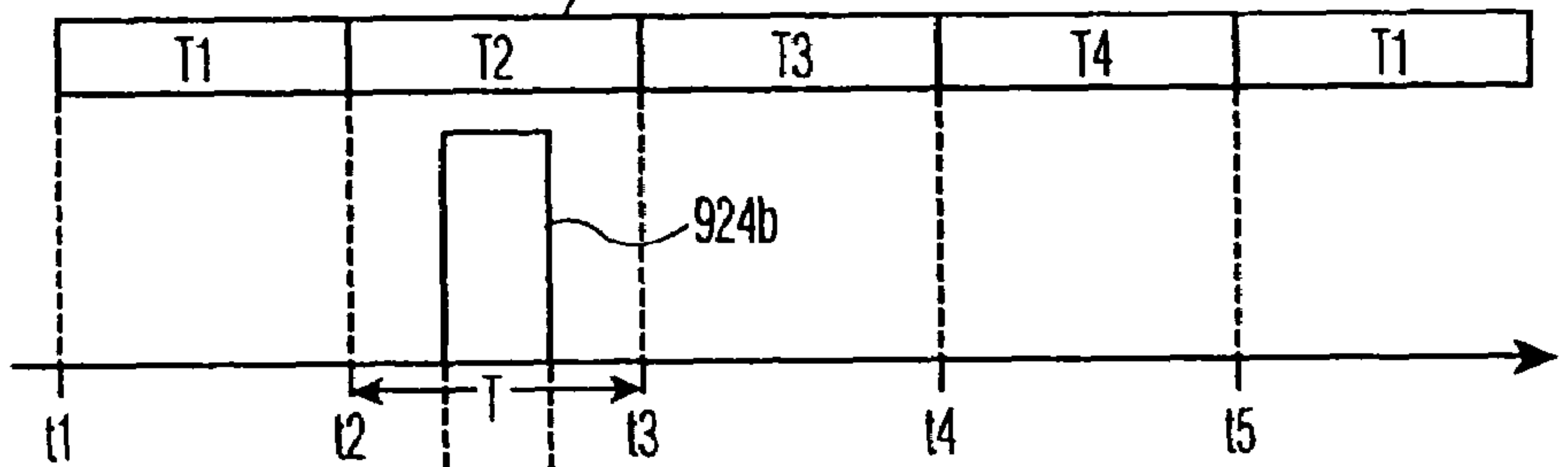
(3) RECORDED SIGNAL OF "01"
