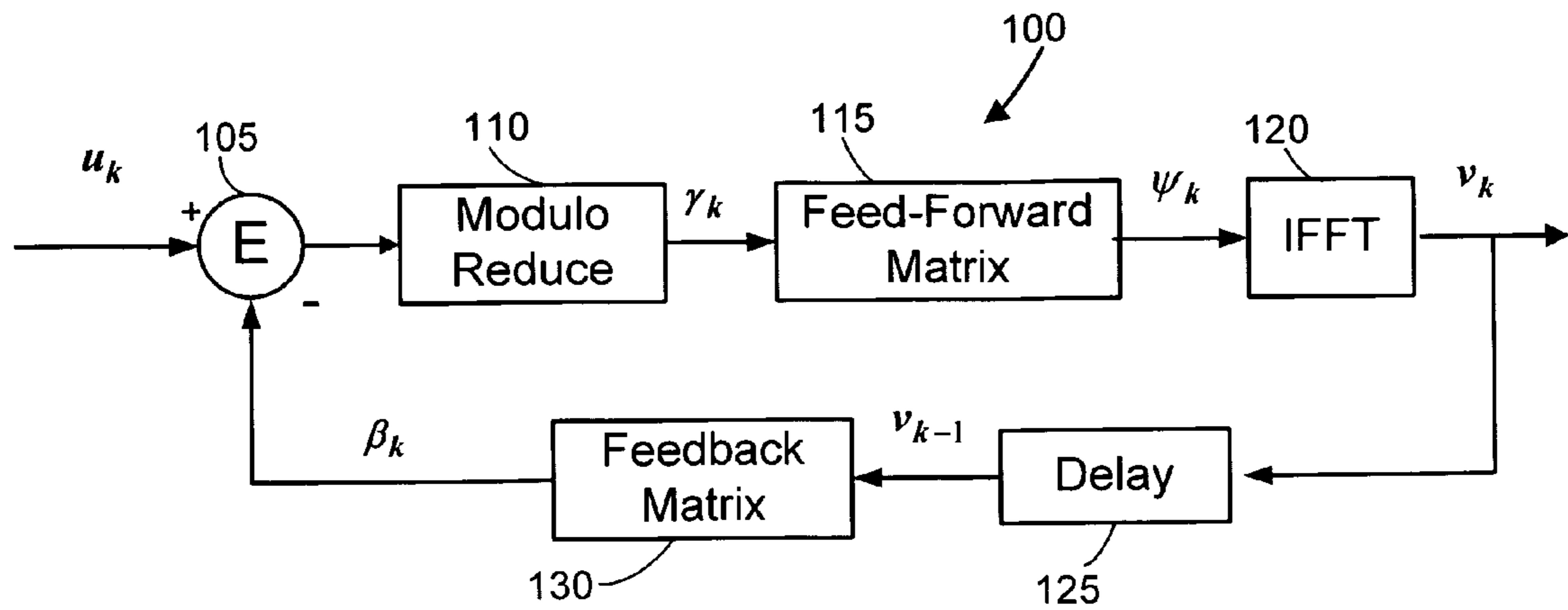
FIG. 1 (prior art)
